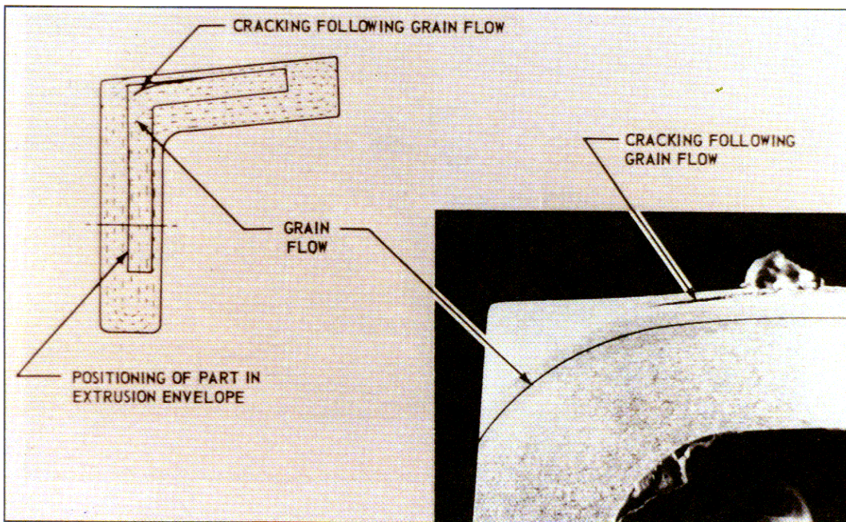
FIGURE 2-14. STRESS-CORROSION CRACKING OF AN EXTRUDED SECTION
