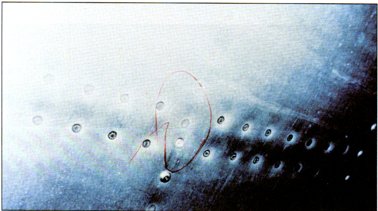
FIGURE 5-4. POPPED RIVET HEADS RESULTING FROM CORROSION PRODUCTS
