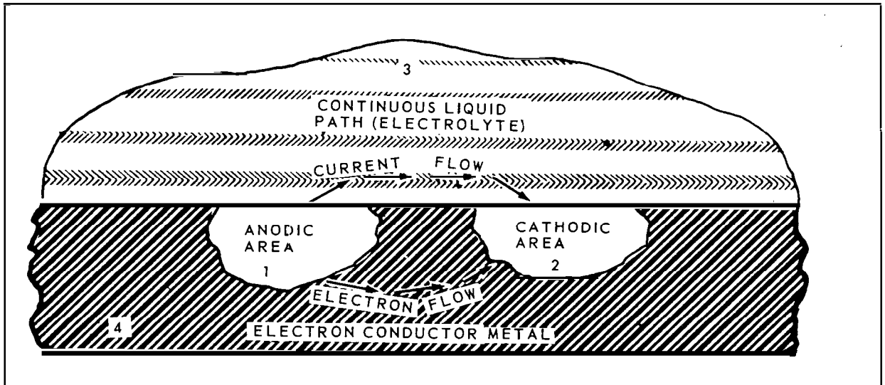
FIGURE 2-1. SIMPLIFIED CORROSION CELL SHOWING CONDITIONS WHICH MUST EXIST FOR ELECTROCHEMICAL CORROSION.
