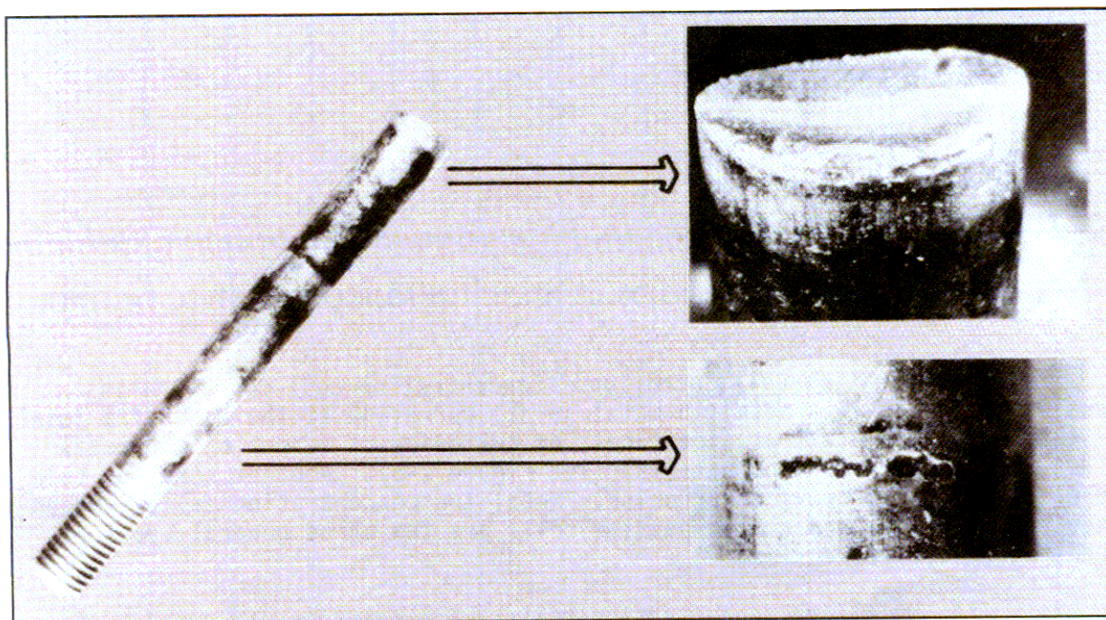
FIGURE 2-4. PITTING CORROSION
