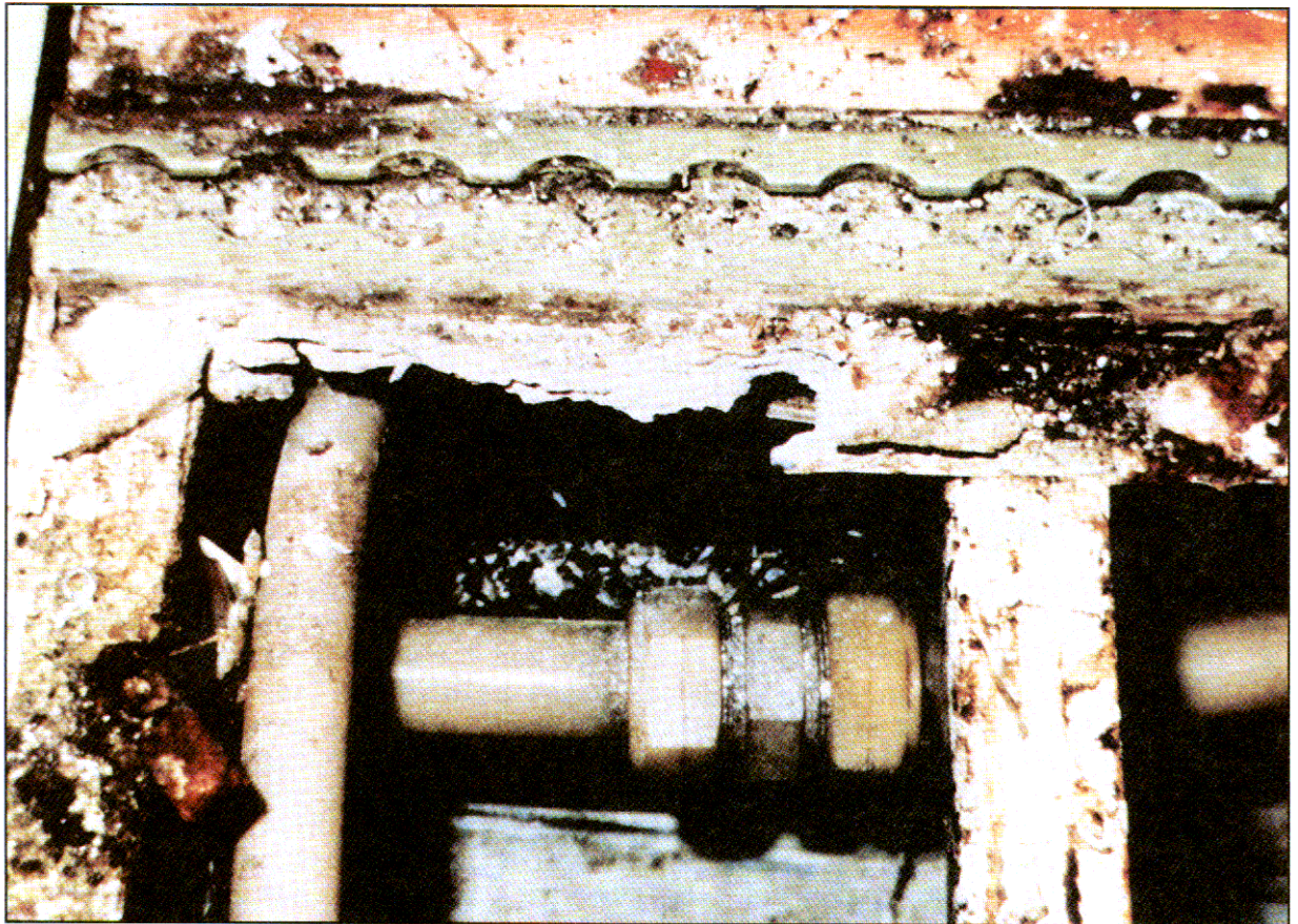
FIGURE 2-8. SEVERE EXFOLIATION CORROSION OF A SEAT TRACK
