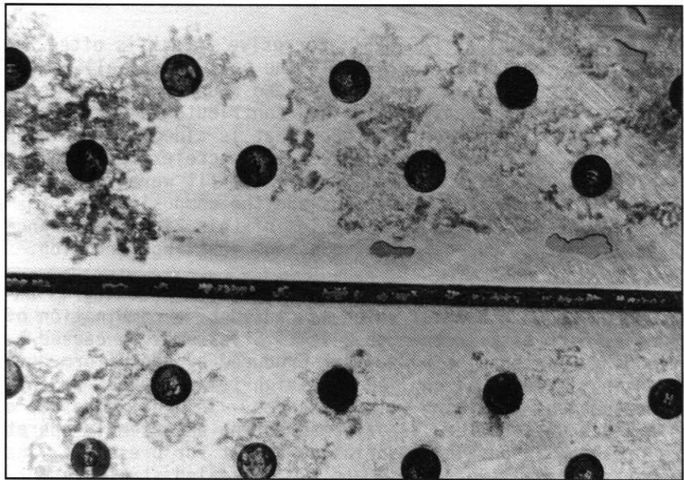
FIGURE 2-10. FILIFORM CORROSION
