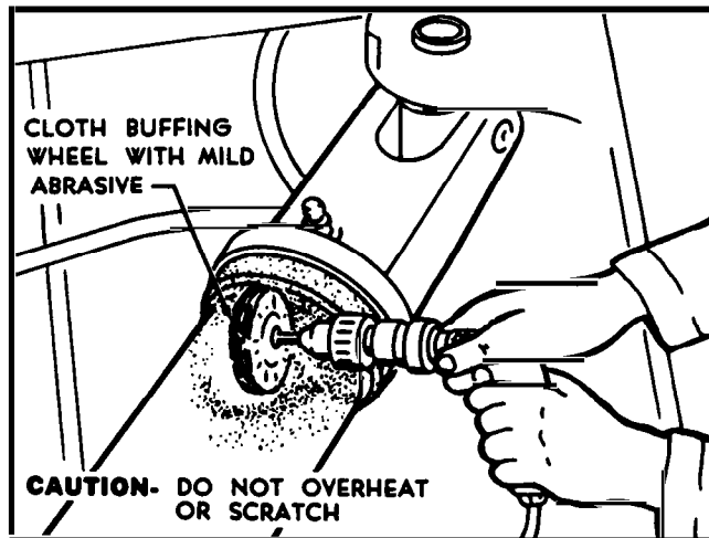
FIGURE 6-18. REMOVING CORROSION PRODUCTS FROM HIGHLY STRESSED STEEL PARTS
