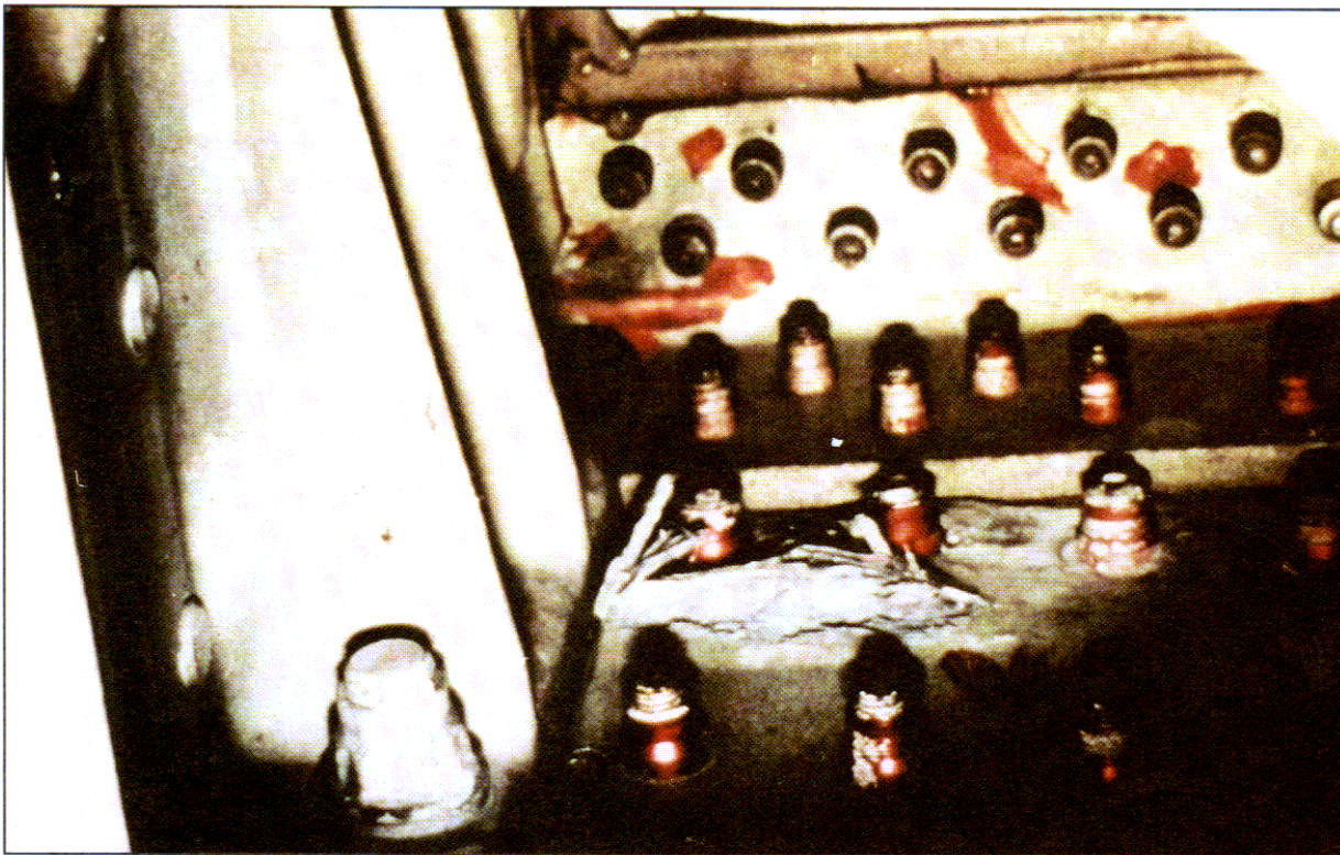
FIGURE 2-9. SEVERE EXFOLIATION CORROSION
