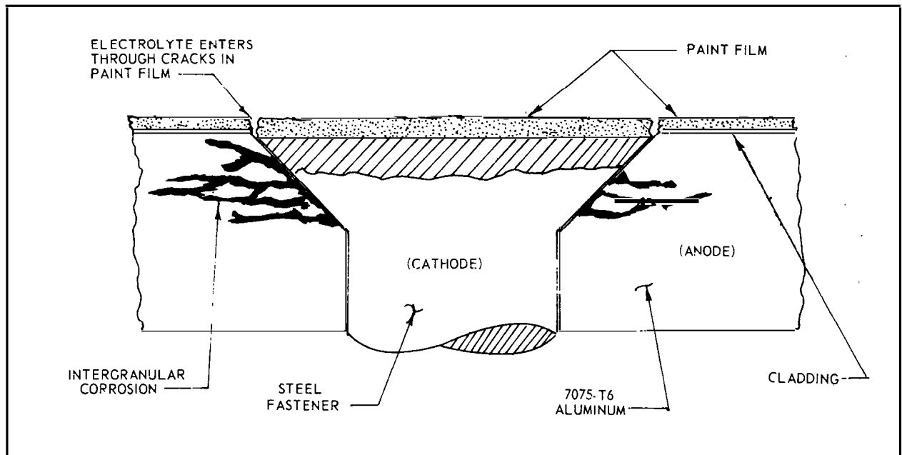
FIGURE 4-4. INTERGRANULAR CORROSION OF 7075-T6 ALUMINUM ADJACENT TO STEEL FASTENER
