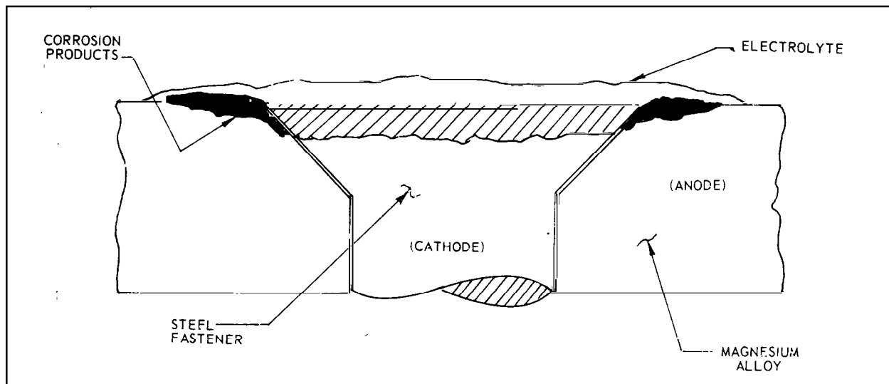
FIGURE 2-5. GALVANIC CORROSION OF MAGNESIUM ADJACENT TO STEEL FASTENER
