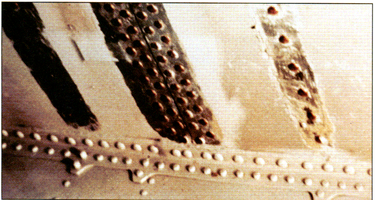
FIGURE 5-16. LOCAL PAINT REMOVAL REQUIRED TO EXPOSE FULL EXTENT OF CORROSION
