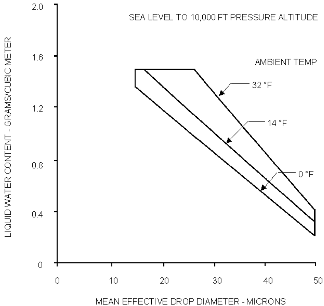
FIGURE 693-4. INTERMITTENT ICING-LIQUID WATER CONTENT VS DROP DIAMETER
