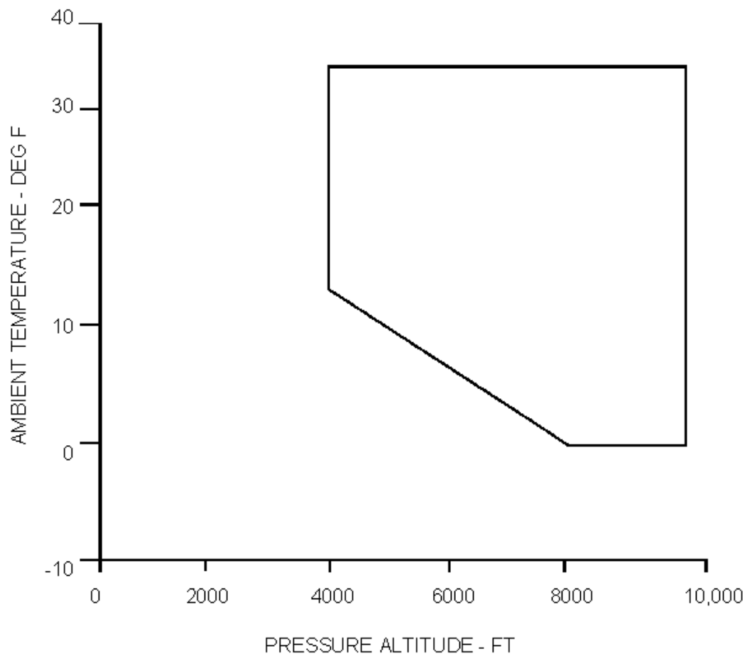
FIGURE 693-2. INTERMITTENT ICING - TEMPERATURE VS ALTITUDE LIMITS
