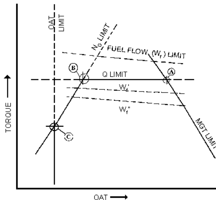
FIGURE 450-1. FUEL FLOW
