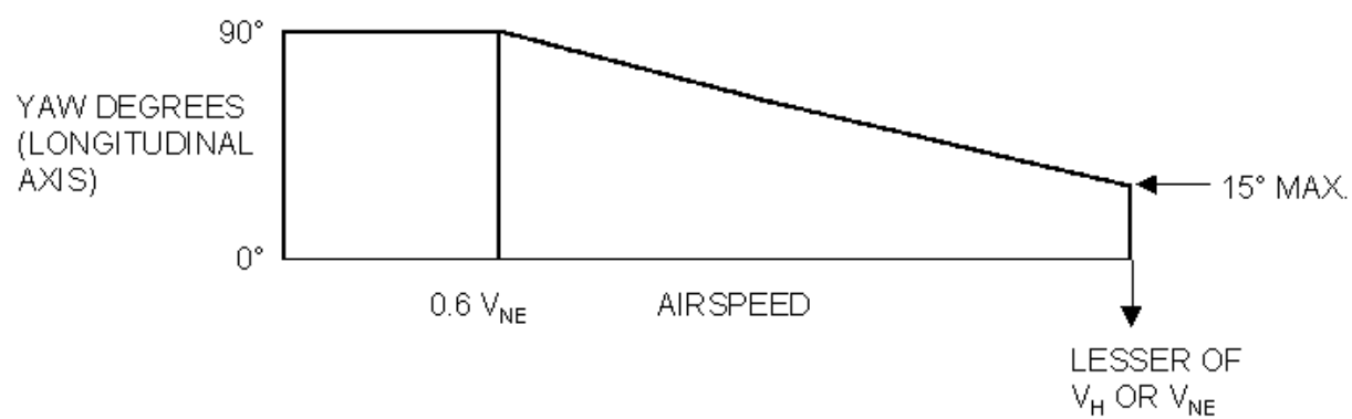
FIGURE 140-1. SAMPLE YAW/FORWARD SPEED DIAGRAM
