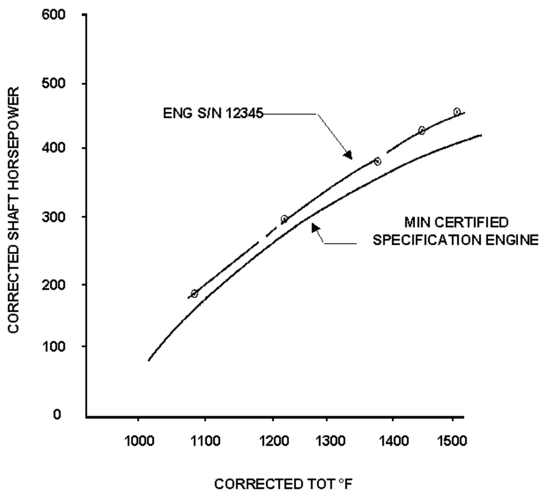
FIGURE 58-3. SHAFT HORSEPOWER VS TURBINE OUTLET TEMPERATURE - SEA LEVEL STANDARD DAY
