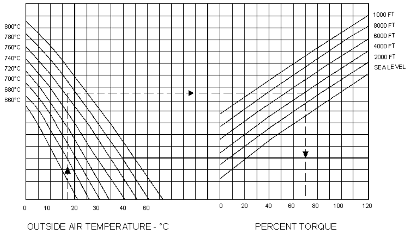
FIGURE 58-6. POWER ASSURANCE CHECK CHART
