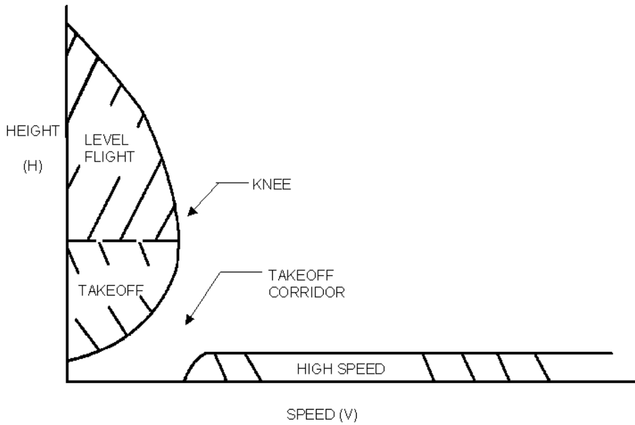
FIGURE 69-1. HEIGHT - VELOCITY DIAGRAM
