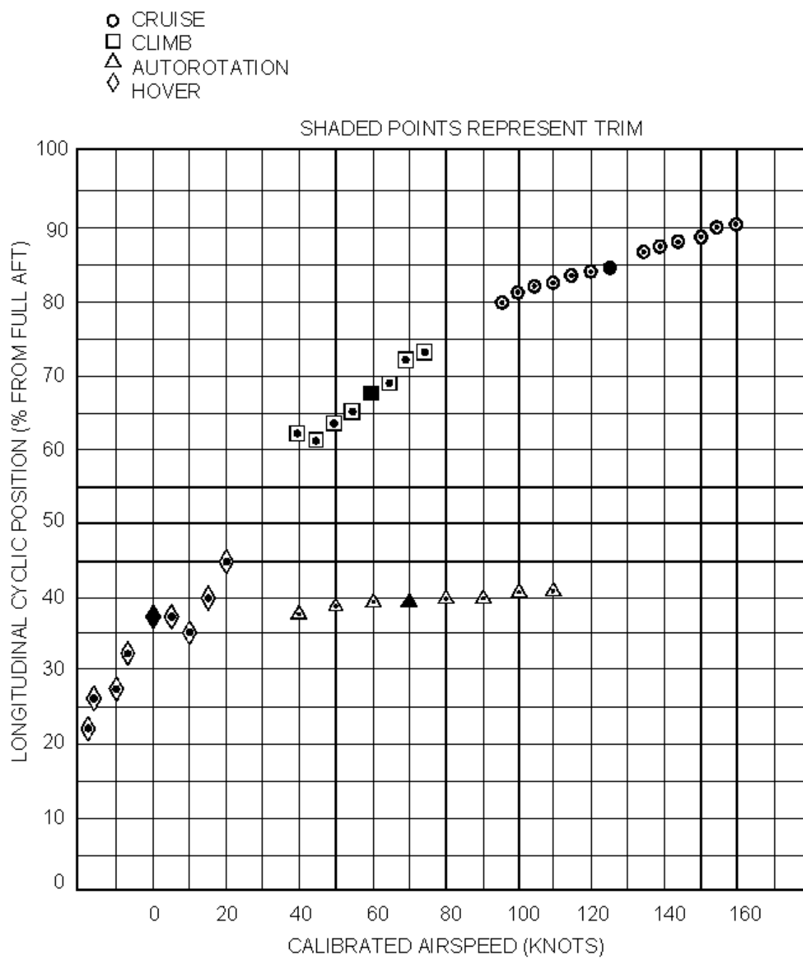
FIGURE 86-1. STATIC LONGITUDINAL STABILITY
