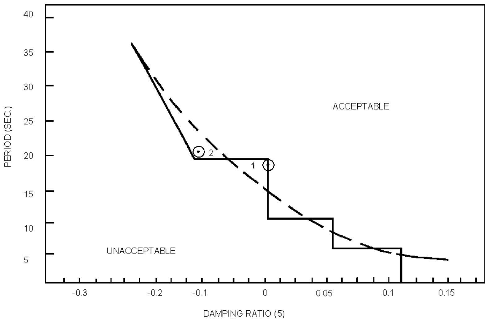
FIGURE 775-1. ROTORCRAFT DYNAMIC STABILITY REQUIREMENTS FOR IFR
