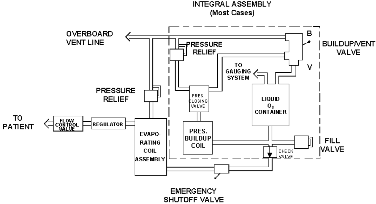
FIGURE 786-1 TYPICAL LIQUID OXYGEN SYSTEM
