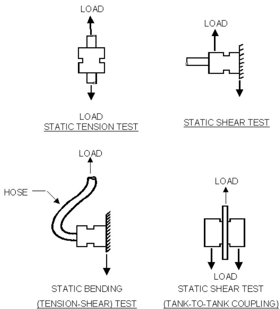
FIGURE 447-1. STATIC TENSION AND SHEAR LOADING MODES
