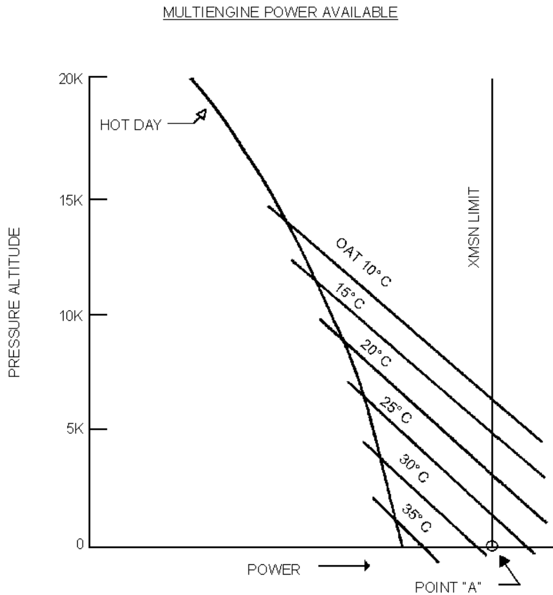
FIGURE 516-1 ADDITIONAL COOLING TEST POINT
