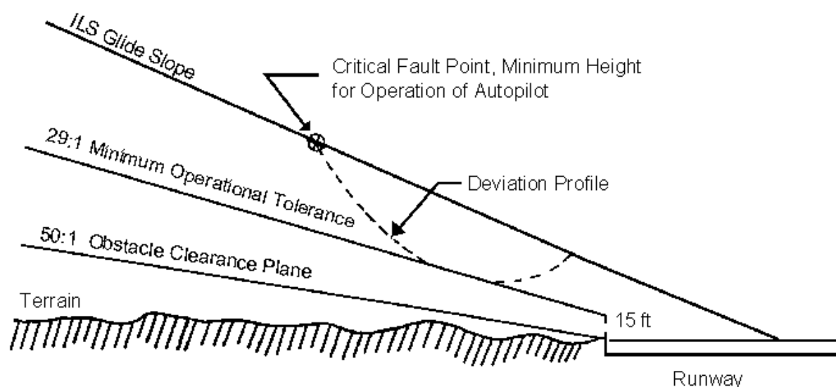
FIGURE 637-2 OPERATIONAL LIMITATION
