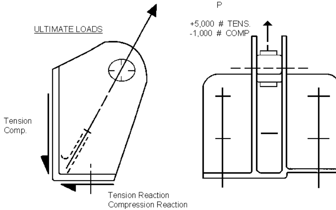
FIGURE 250-1 EXAMPLE OF CASTING LOAD SHEET RETRACT ACTUATOR SUPPORT - LANDING GEAR
