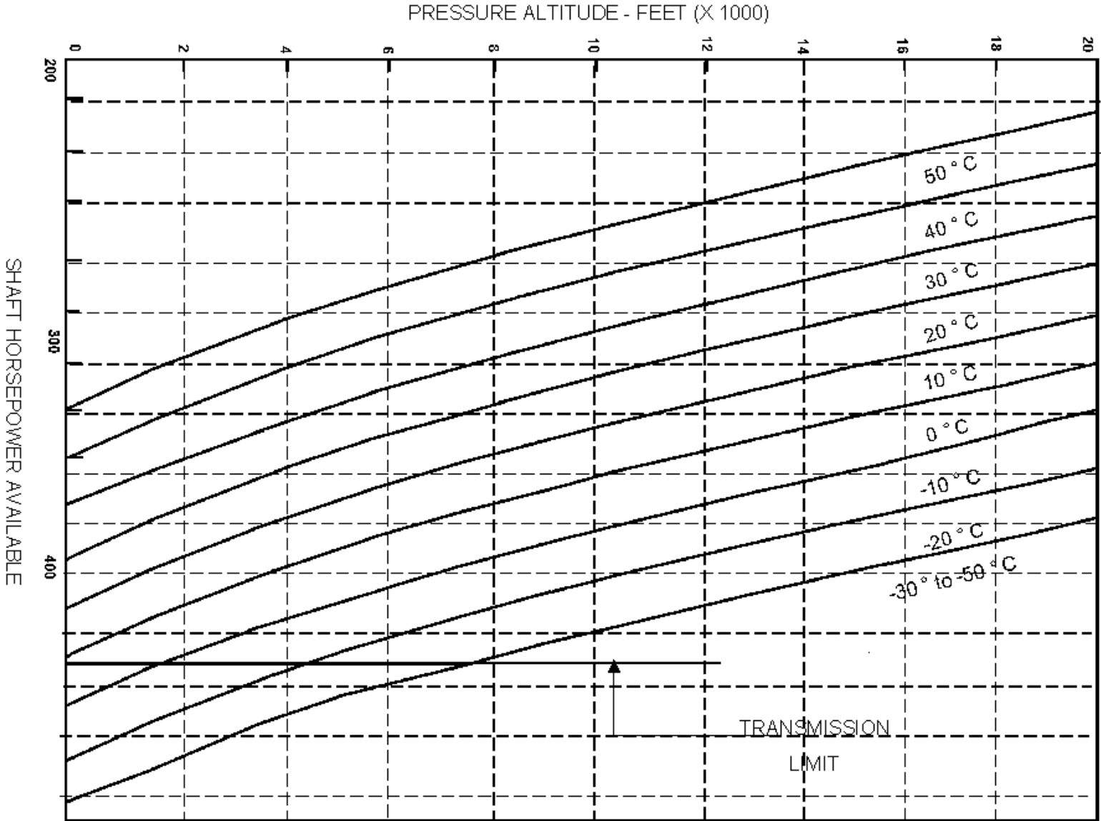
FIGURE 58-5. INSTALLED TAKEOFF POWER AVAILABLE, ANTI-ICE OFF, 400 RPM
