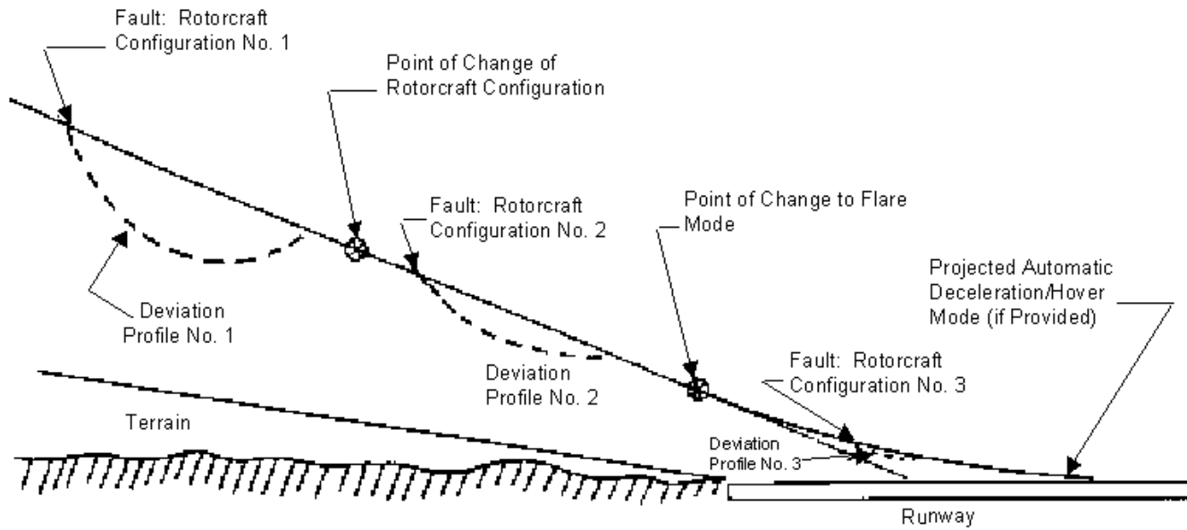
FIGURE 637-1 DEVIATION PROFILE
