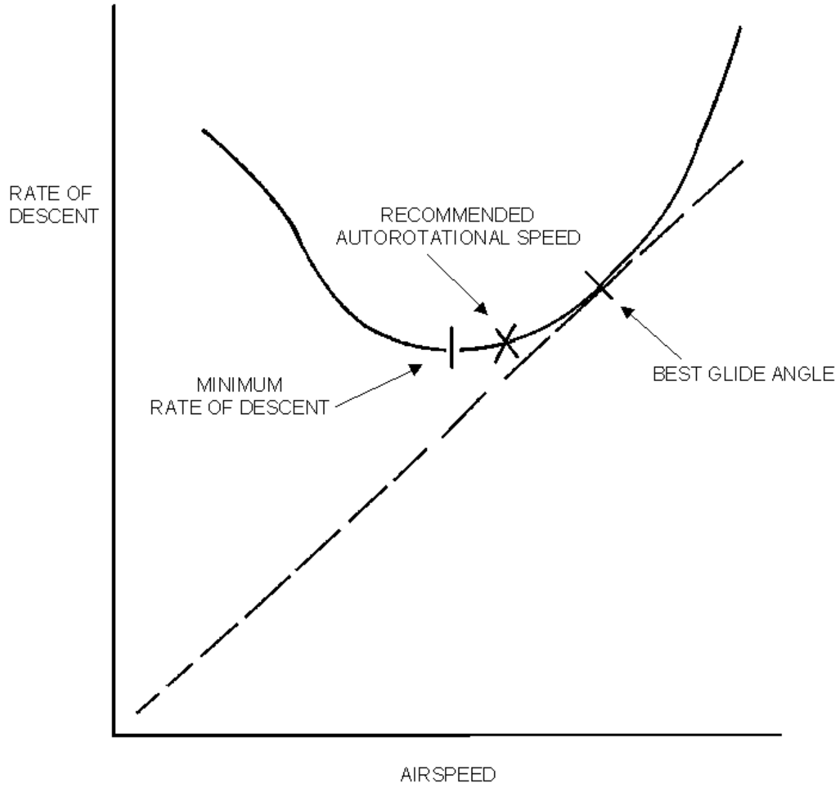
FIGURE 65-1. AUTOROTATIONAL CHARACTERISTICS - TYPICAL
