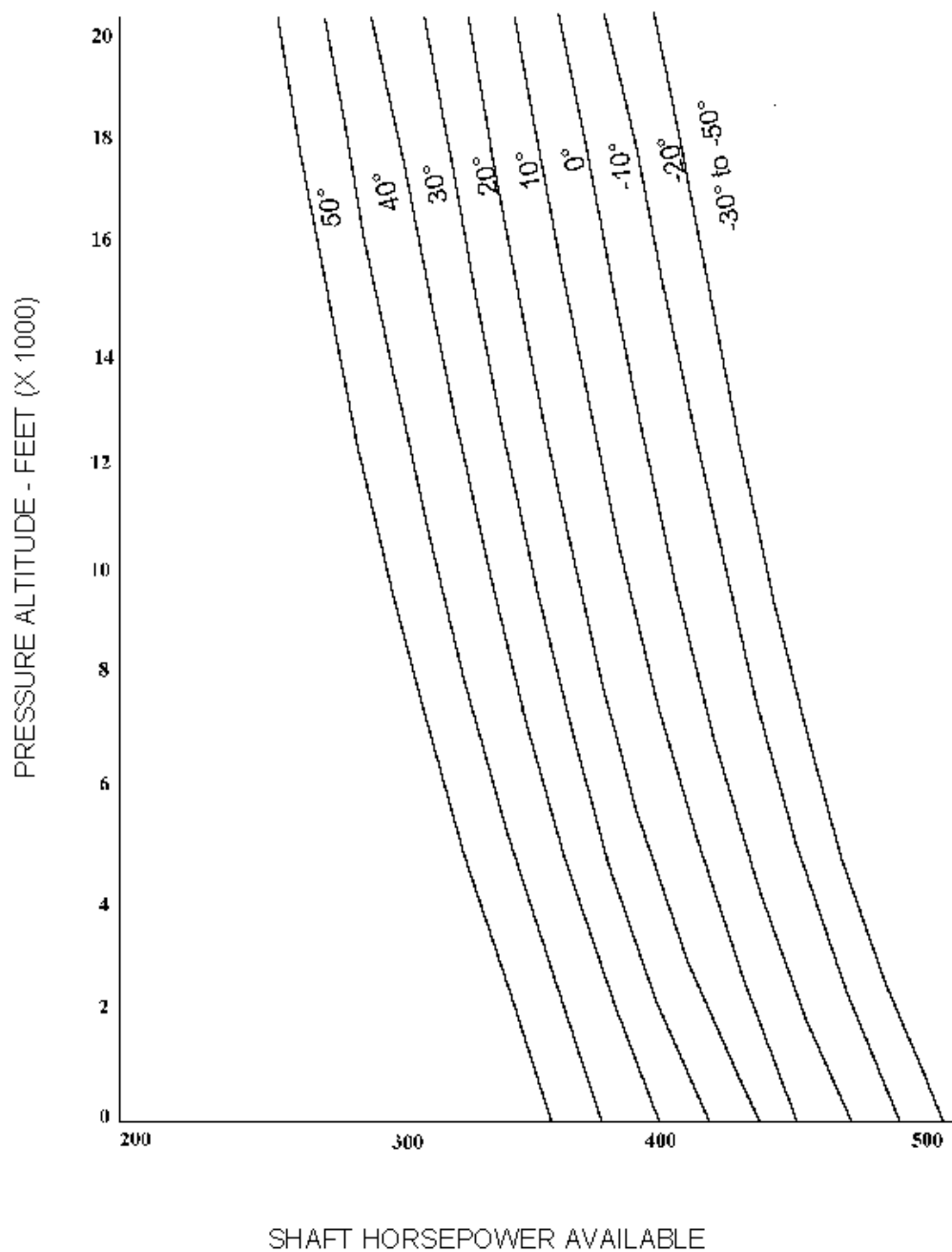
FIGURE 58-4. UNINSTALLED TAKEOFF POWER AVAILABLE
