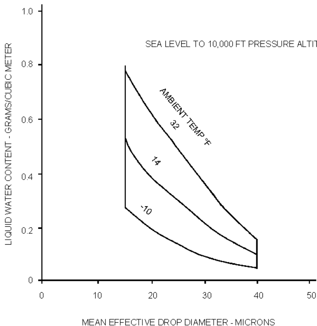
FIGURE 693-3. CONTINUOUS ICING-LIQUID WATER CONTENT VS. DROP DIAMETER
