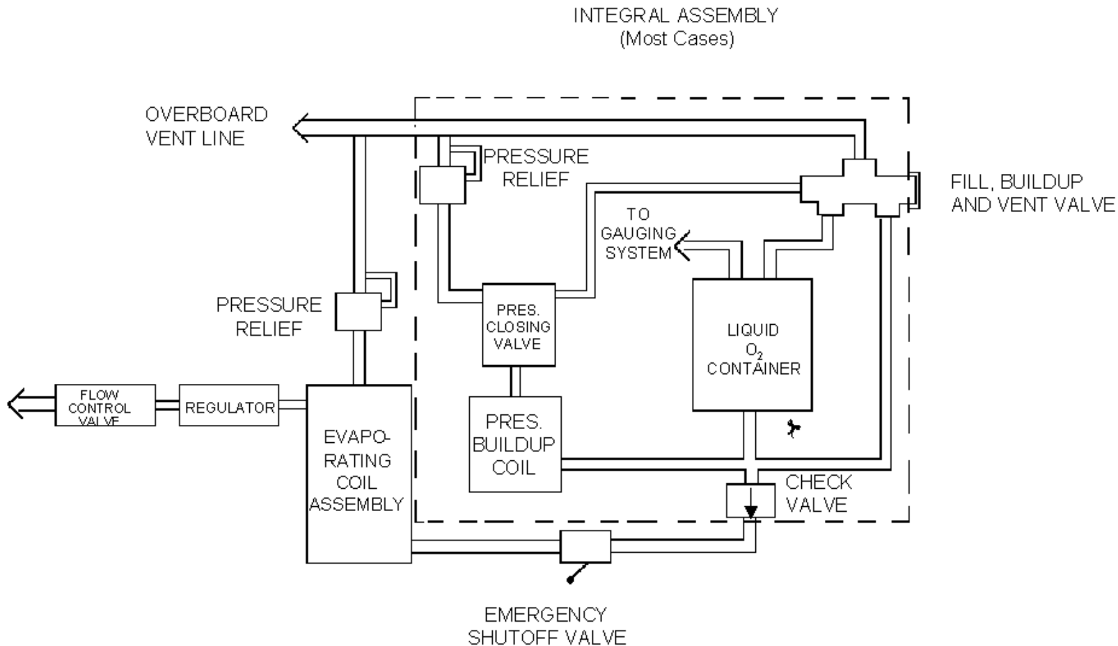
FIGURE 786-2 TYPICAL LIQUID OXYGEN SYSTEM - USING COMBINATION VALVE
