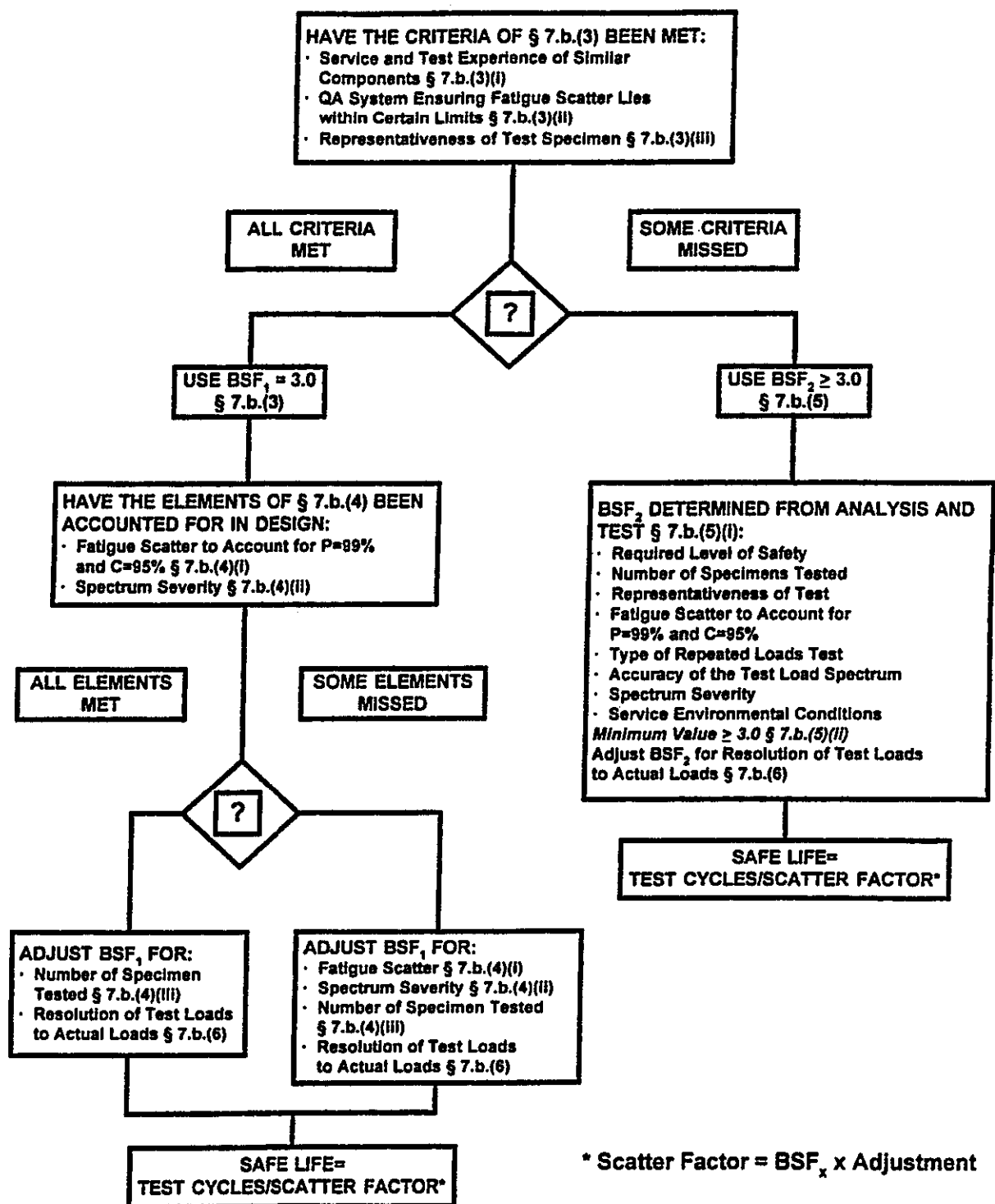
Figure 1. Safe-Life Determination
