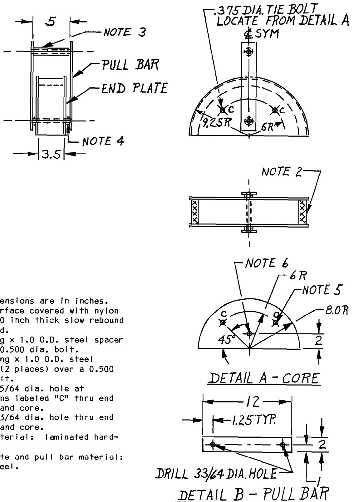
Figure 2 - SHOULDER HARNESS BLOCK
