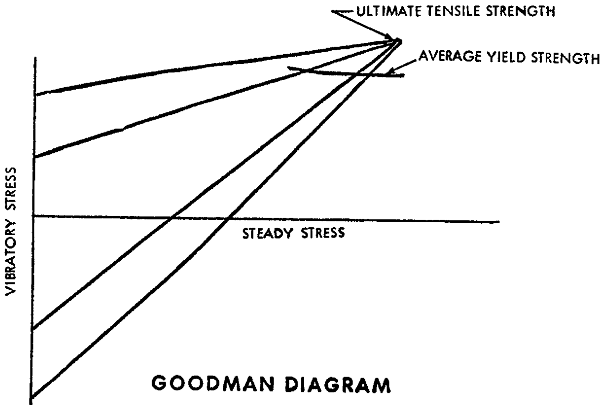
FIGURE 1. GOODMAN DIAGRAMS
