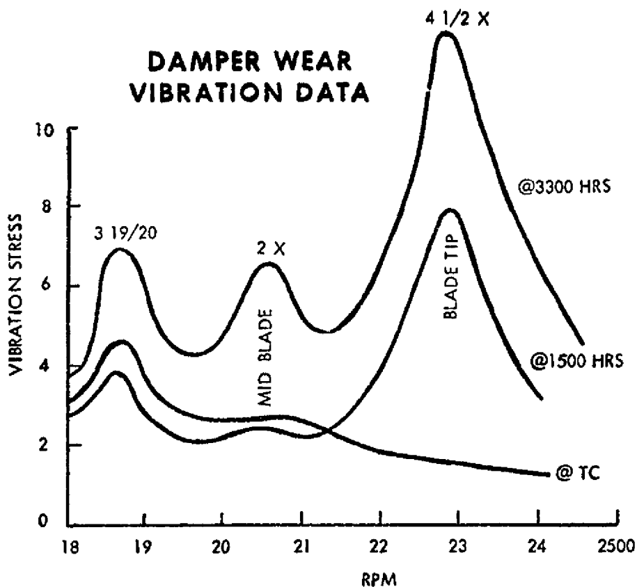
FIGURE 6. VIBRATION DATA - DAMPER WEAR VIBRATION DATA - FLAPS ON TAKEOFF
