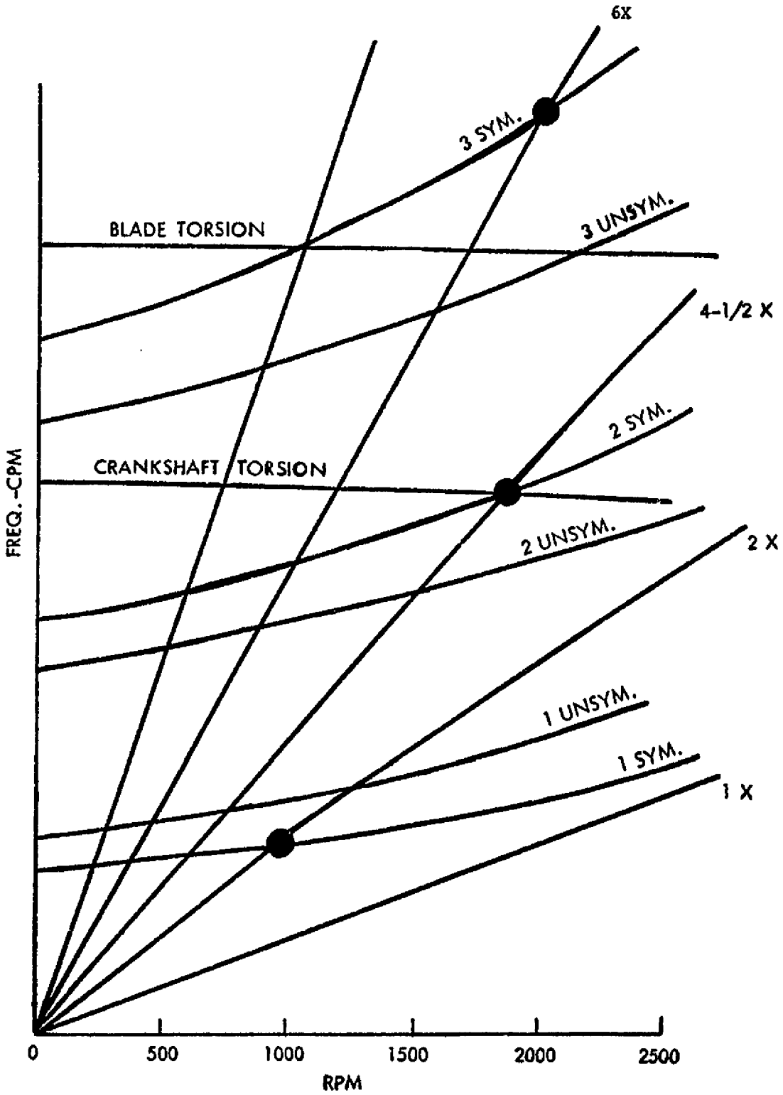
FIGURE 5. CAMPBELL DIAGRAM
