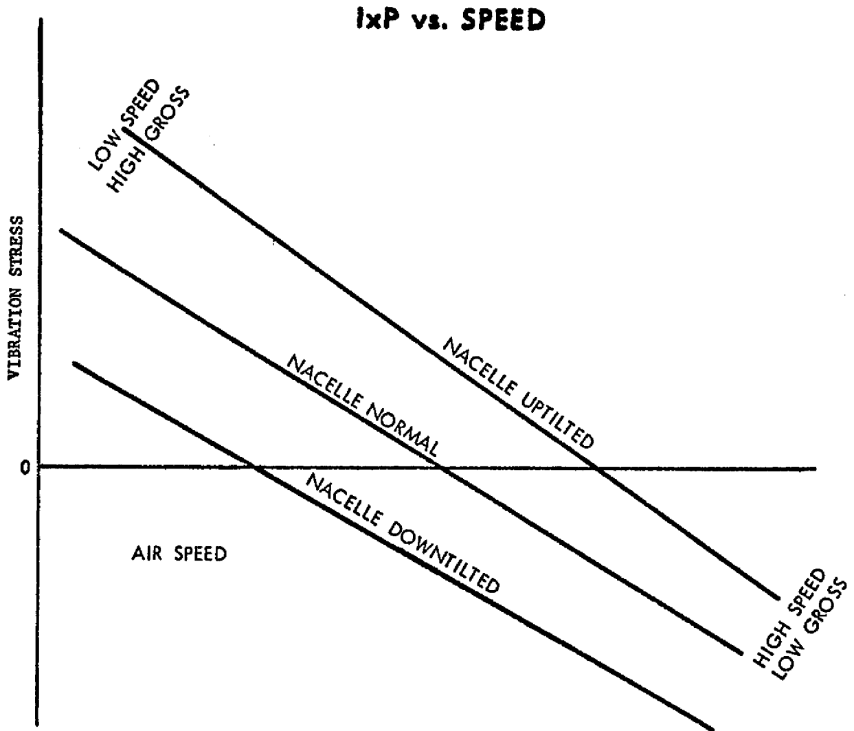
FIGURE 8. IXP STRESSES VERSUS SPEED
