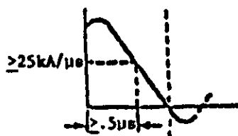
FIGURE 4 CURRENT WAVEFORMS
