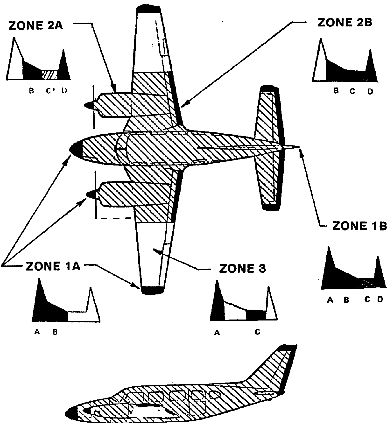
FIGURE 3 LIGHTNING STRIKE ZONES (TYPICAL) (See paragraph 10C)
