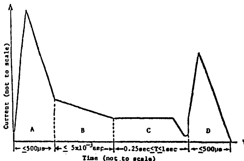
COMPONENTS A THROUGH D WAVEFORMS
