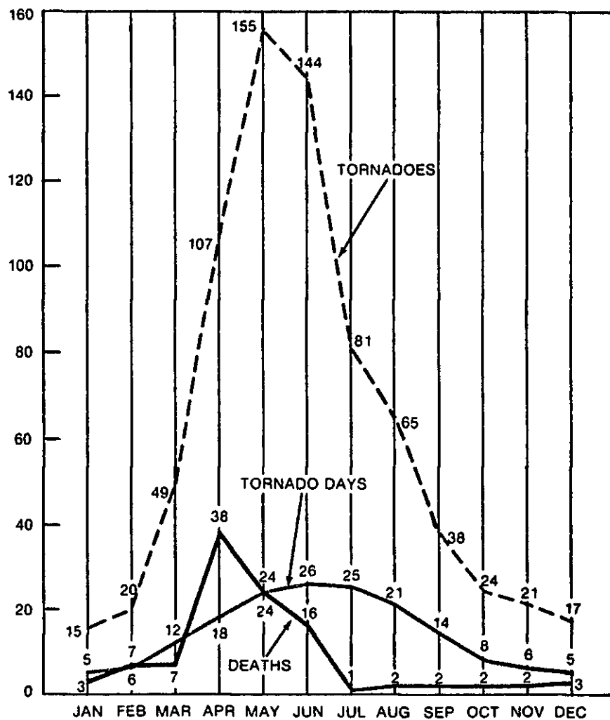
TORNADO INCIDENCE BY MONTH 1953-1980
