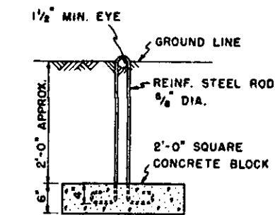
ROD AND BLOCK ANCHOR
