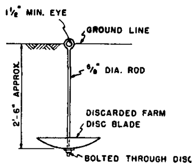
MUSHROOM TYPE ANCHOR
