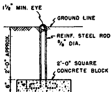
ROD AND BLOCK ANCHOR
