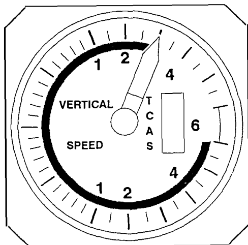
(a) Preventive MONITOR VERTICAL SPEED.
