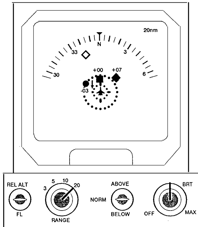
Figure 2: TCAS II - Traffic Display (Example).
