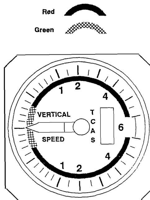
(b) Preventive MONITOR VERTICAL SPEED.
