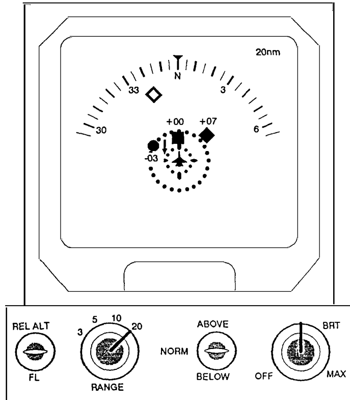
Figure 2: TCAS II - Traffic Display (Example) (Con't).
