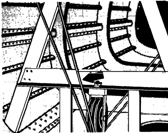
FIGURE 1-7. Proper cable routing.
