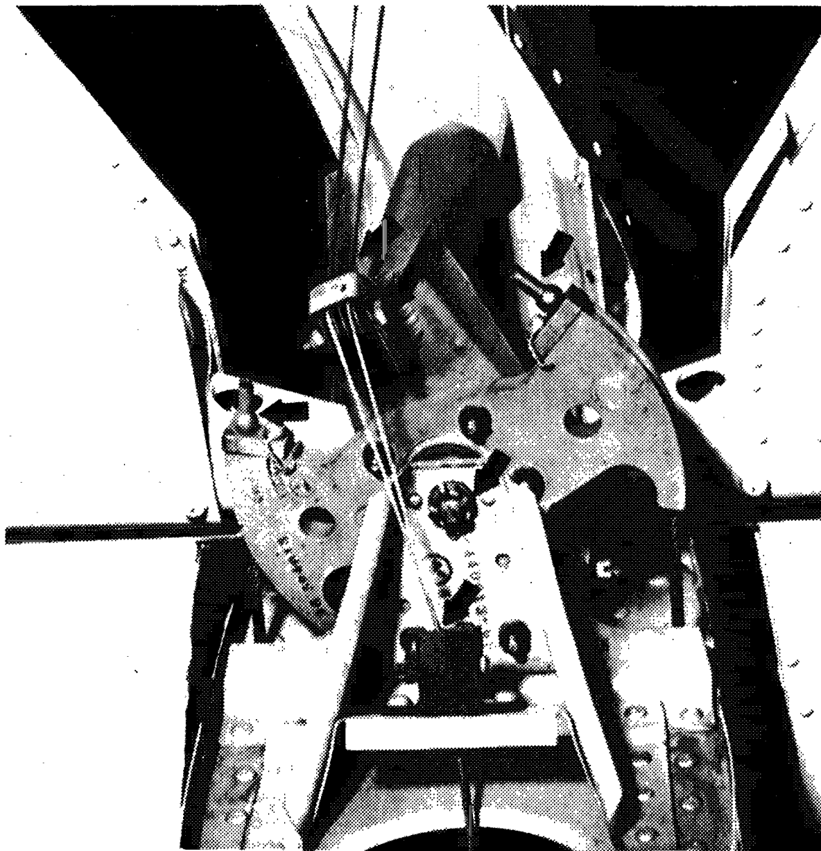
FIGURE 6-5. Rudder quadrant.
