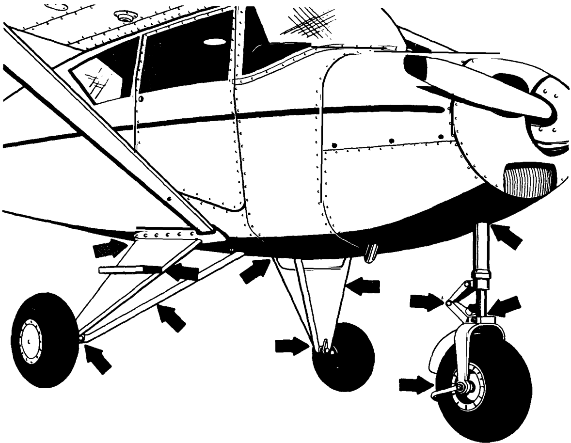
FIGURE 4-11. Wheel checkpoints.
