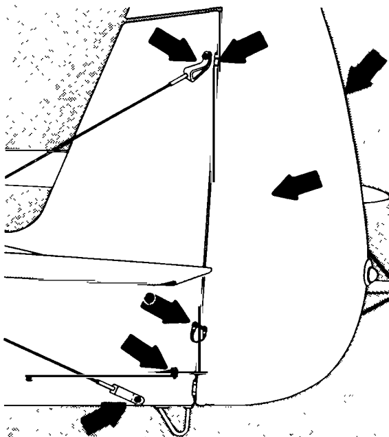
FIGURE 6-4. Rudder checkpoints.
