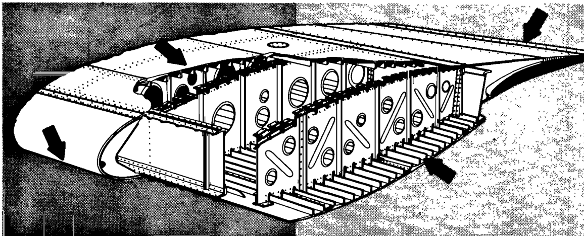
FIGURE 5-4. Metal structure inspection points.
