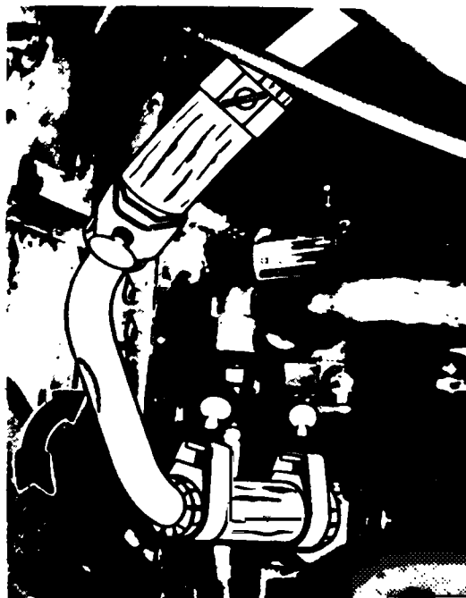
FIGURE 3-10. Unsatisfactory oil line installation.
