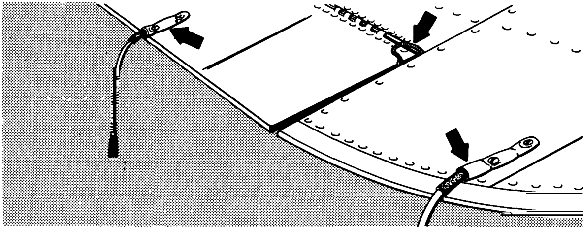
FIGURE 8-9. Bonding wires and trailing edge static wicks.
