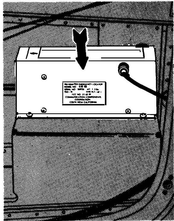
9-3. Emergency locator transmitter — remote mount.
