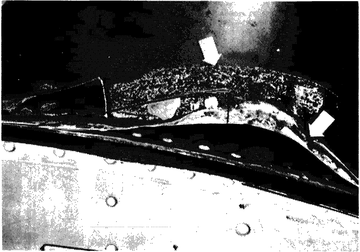
FIGURE 3-27. Evidence of chafing.
