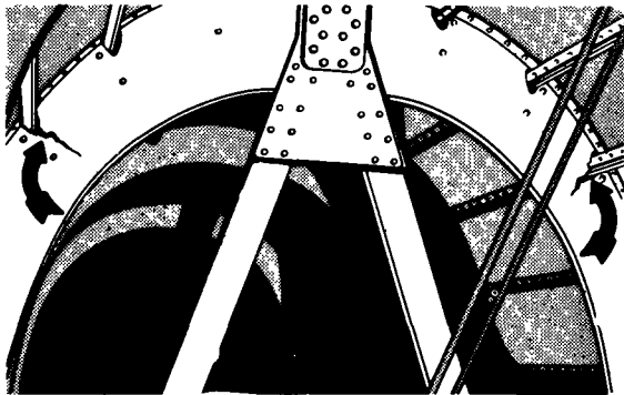
FIGURE 1-3. Cracked former.
