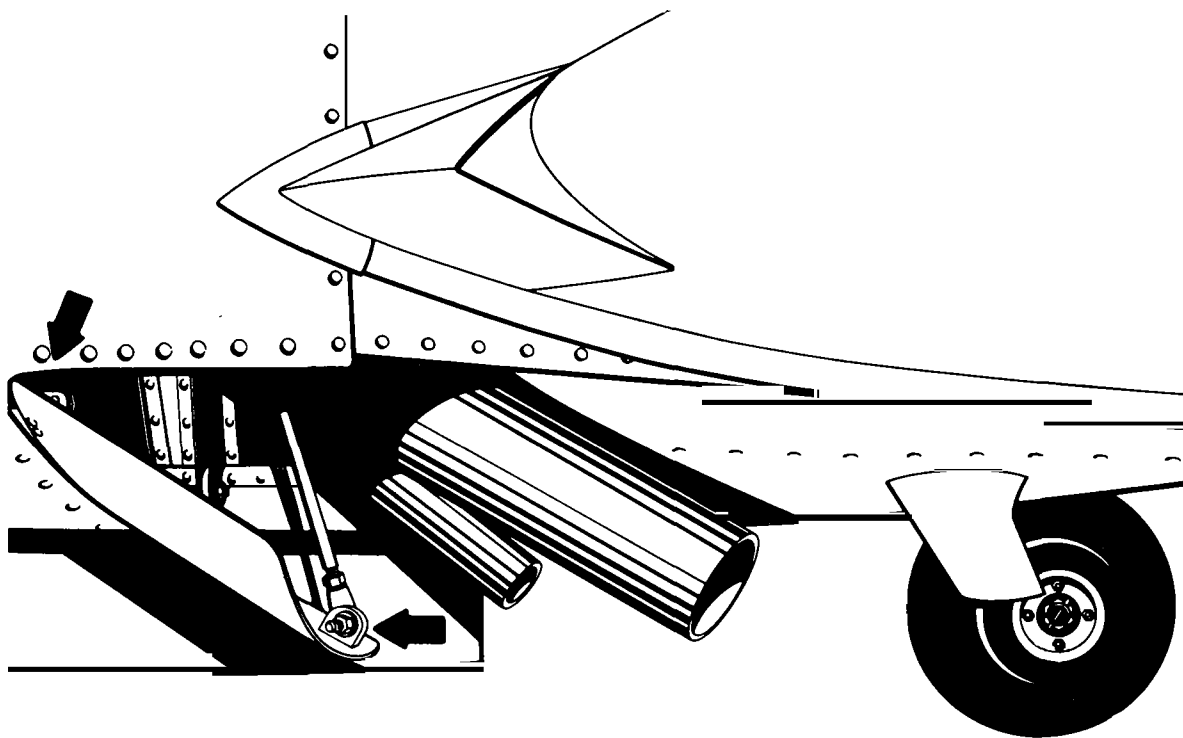
FIGURE 3-18. Cowl flap checkpoints.
