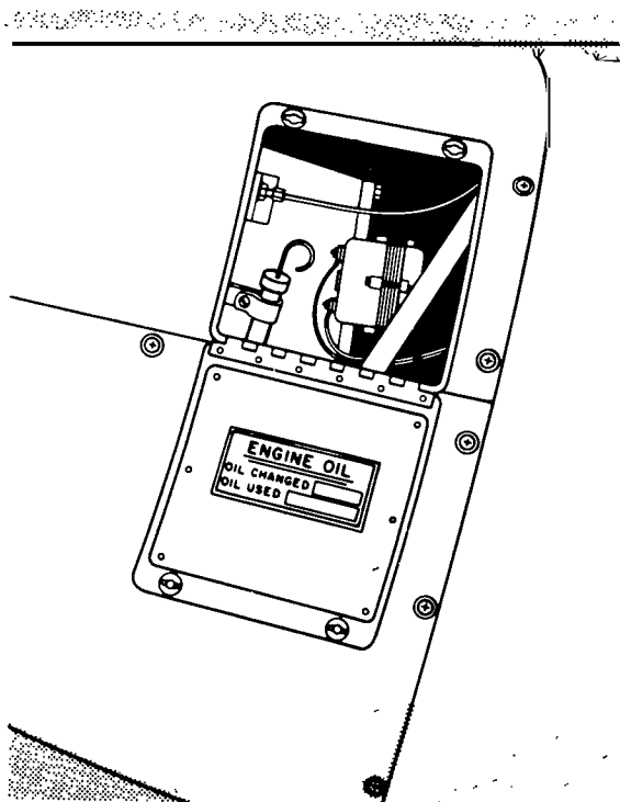
FIGURE 3-8. Oil quantity check.
