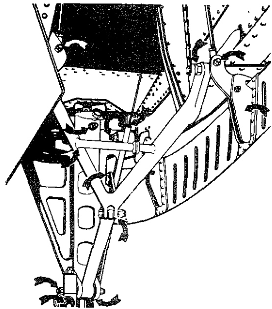
FIGURE 4-20 Retracting mechanism checkpoints
