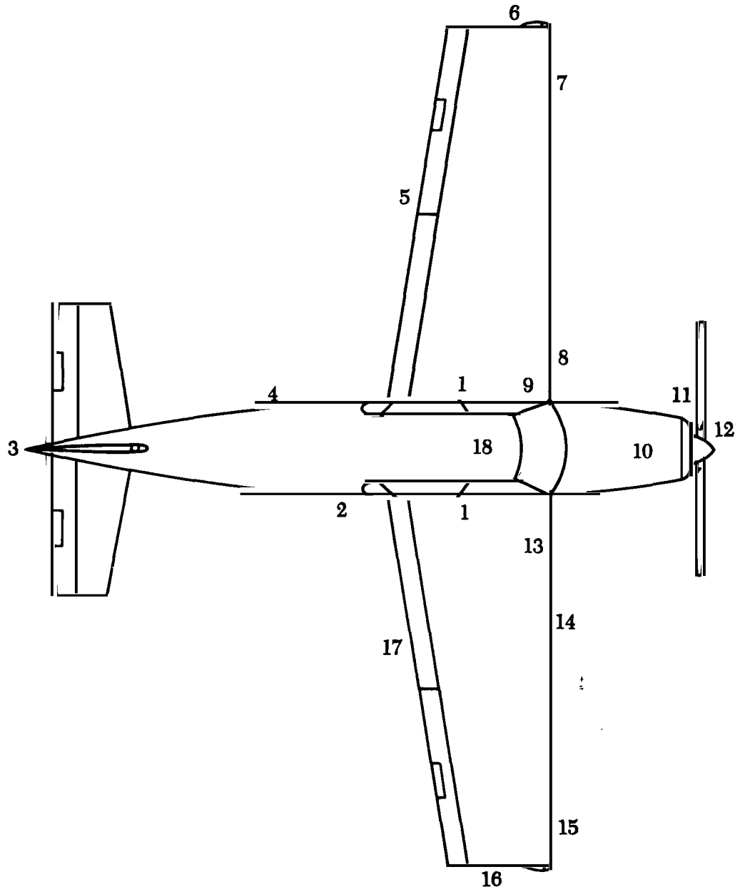
FIGURE 10-1. Inspection chart—preflight.
