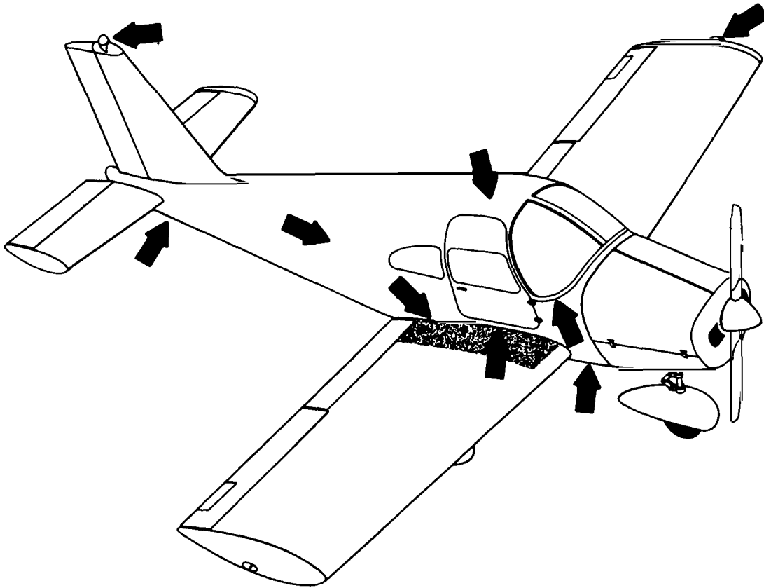
FIGURE 1-1. Inspection chart - fuselage.
