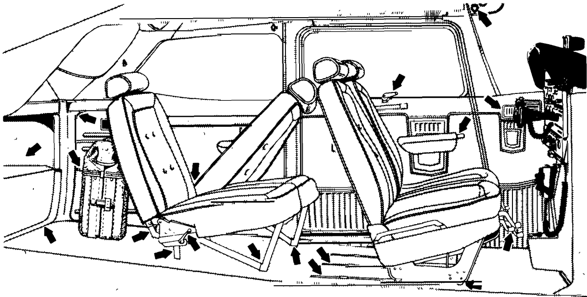
2-2. Inspection chart – cabin.
