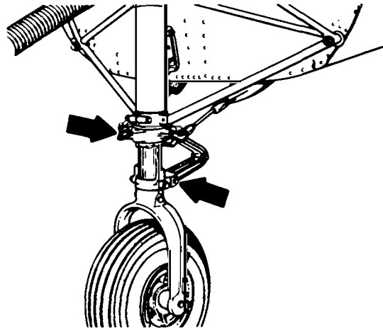
FIGURE 4-13. Fixed nose gear check points.
