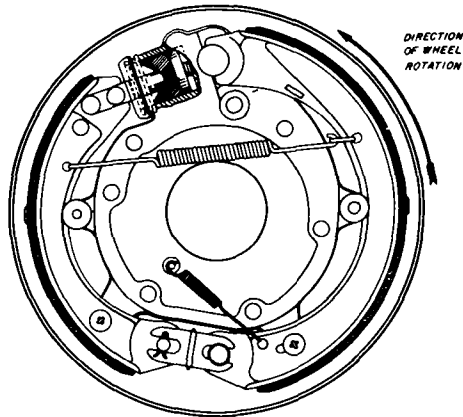
FIGURE 4-4. Shoe and drum-type brake.
