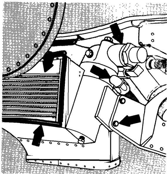
FIGURE 3-11. Oil-cooler checkpoints.
