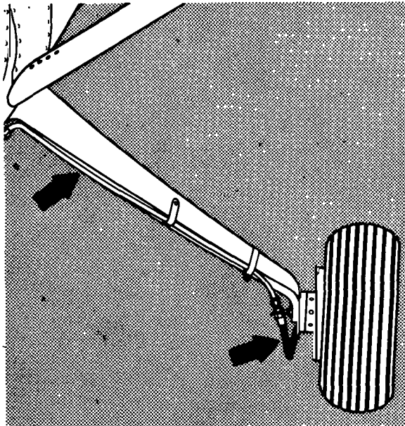
FIGURE 4-8. Hydraulic brake line checkpoints.
