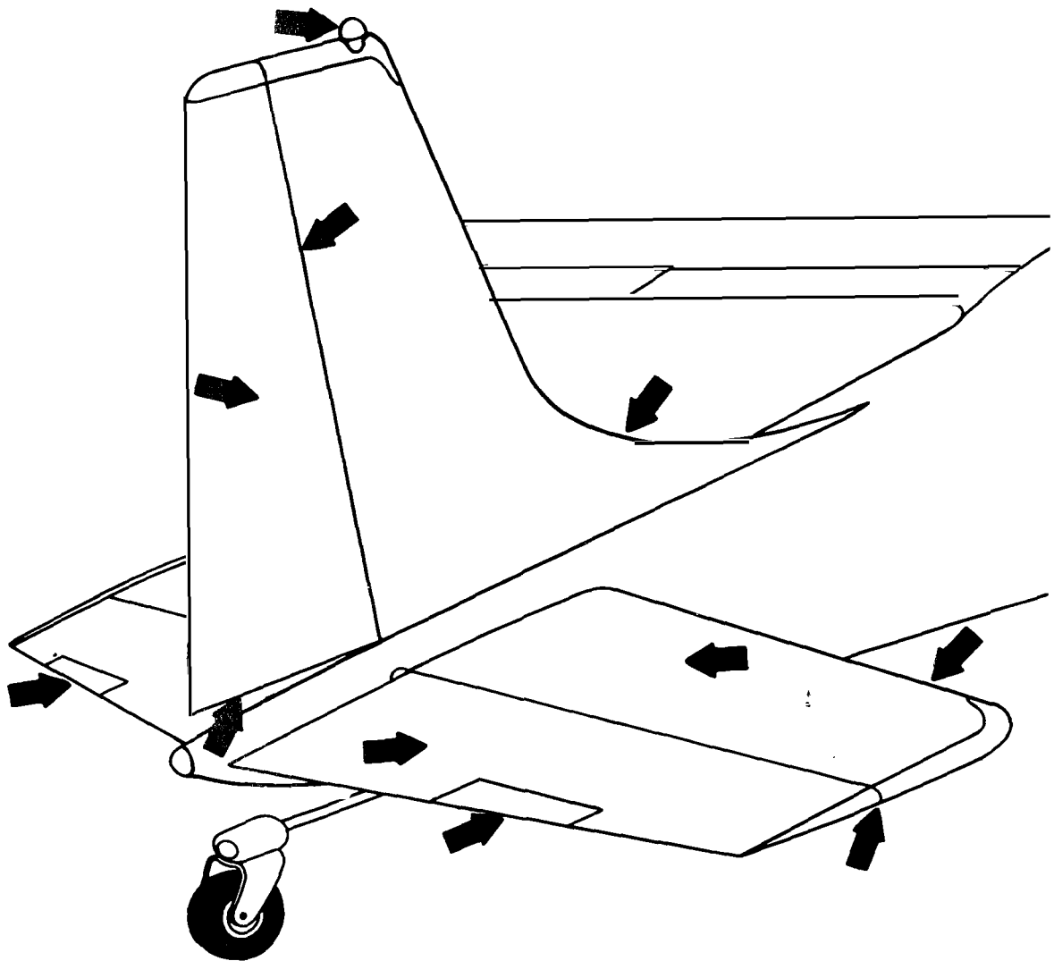
FIGURE 6-1. Inspection chart—empennage.
