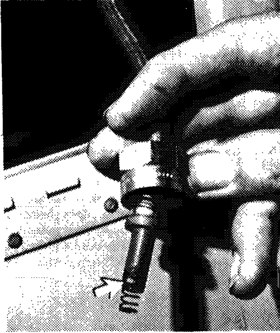
FIGURE 3-13. Unsatisfactory sparkplug cigarette.
