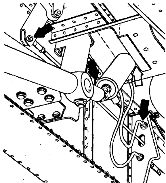
FIGURE 4-17. Retractable main gear checkpoints.
