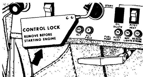
FIGURE 2-9. Gustlock.
