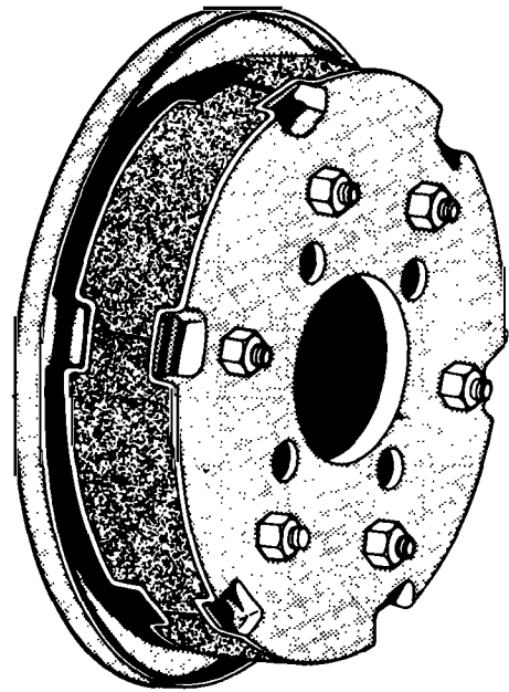
FIGURE 4-5. Expander block-type brake.
