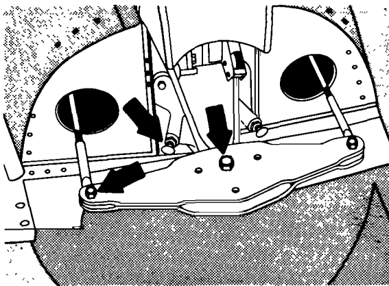
FIGURE 2-7. Bellcrank checkpoints.
