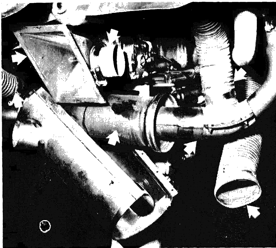
FIGURE 3-17. Heat exchanger—shroud removed.
