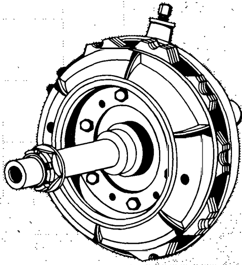
FIGURE 4-3. Multiple disc-type brake.
