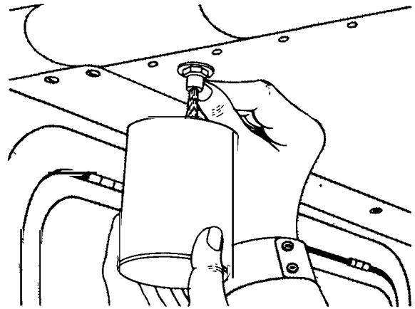
FIGURE 1-12. Draining fuel tank sump.
