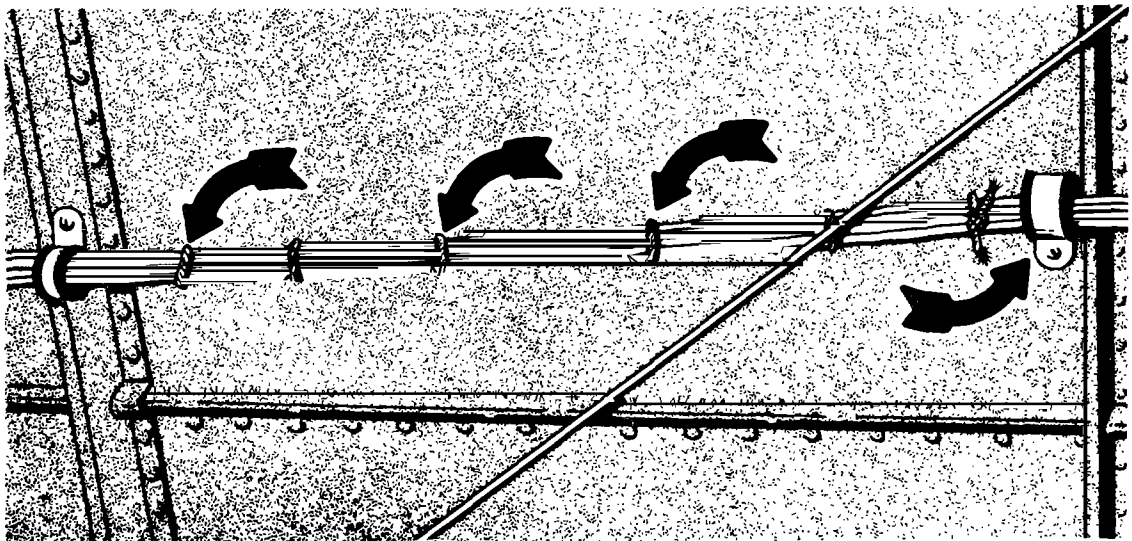
FIGURE 1-9. Proper routing of electrical wiring.
