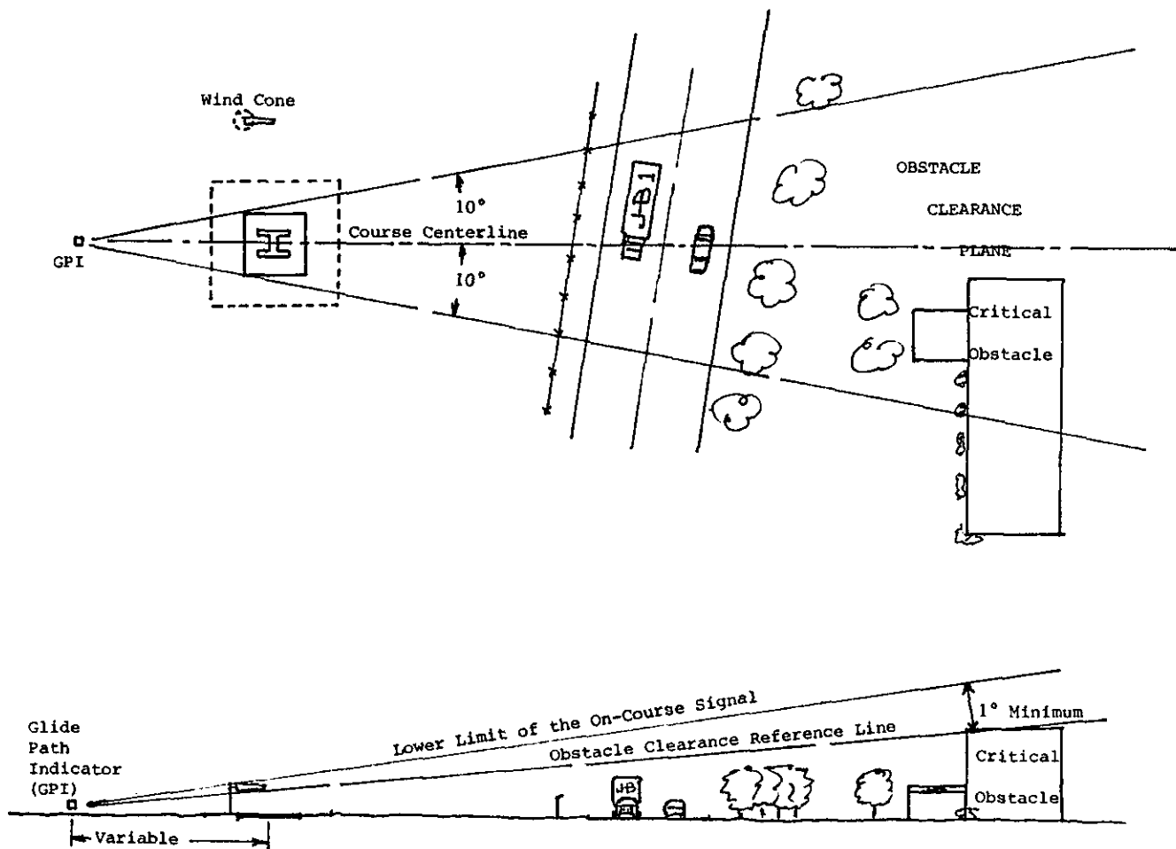
Figure 3-10. Visual Glide Path Indicator Siting and Clearance Criteria
