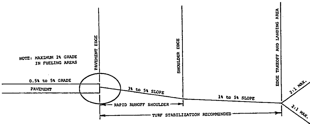
Figure 8-1. Heliport Gradients
