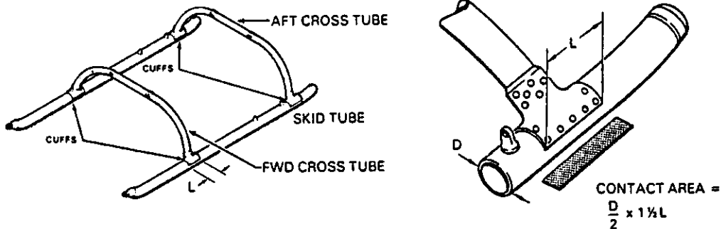
Figure 8-3. Helicopter Landing Gear Loading
