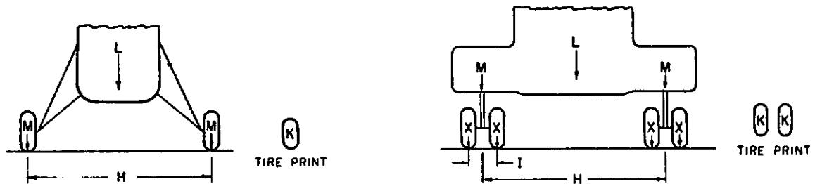
A. TYPICAL SINGLE-WHEELED CONFIGURATION (CONCEPT APPLIES TO SKID/FLOAT EQUIPPED HELICOPTERS)
