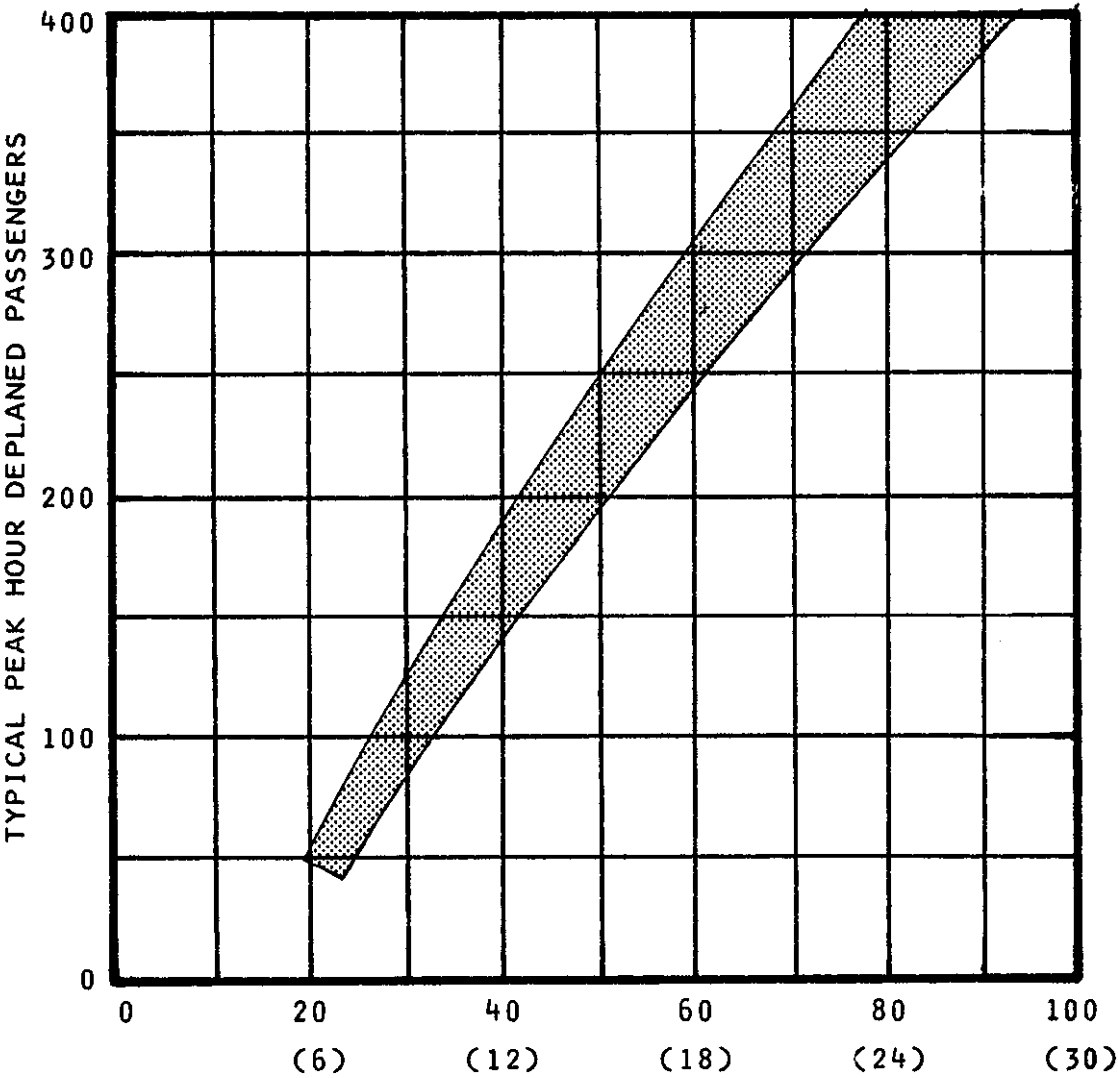
BAGGAGE CLAIM COUNTER OR DISPLAY LENGTH IN LINEAR FEET AND (LINEAR METERS)
