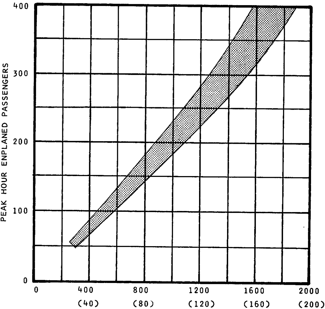
QUEUEING AREA IN FRONT OF AIRLINE TICKET COUNTERS IN SQUARE FEET AND (SQUARE METERS)
