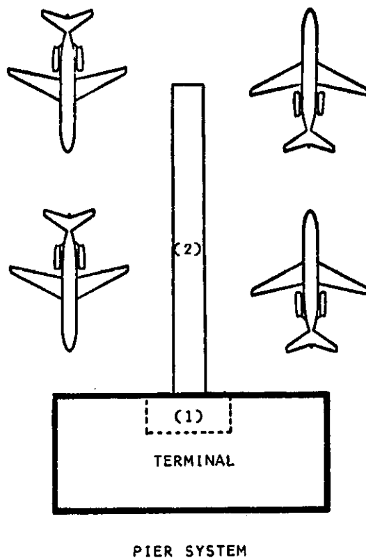
FIGURE 4-3. AIRCRAFT PARKING AND TERMINAL CONFIGURATIONS
