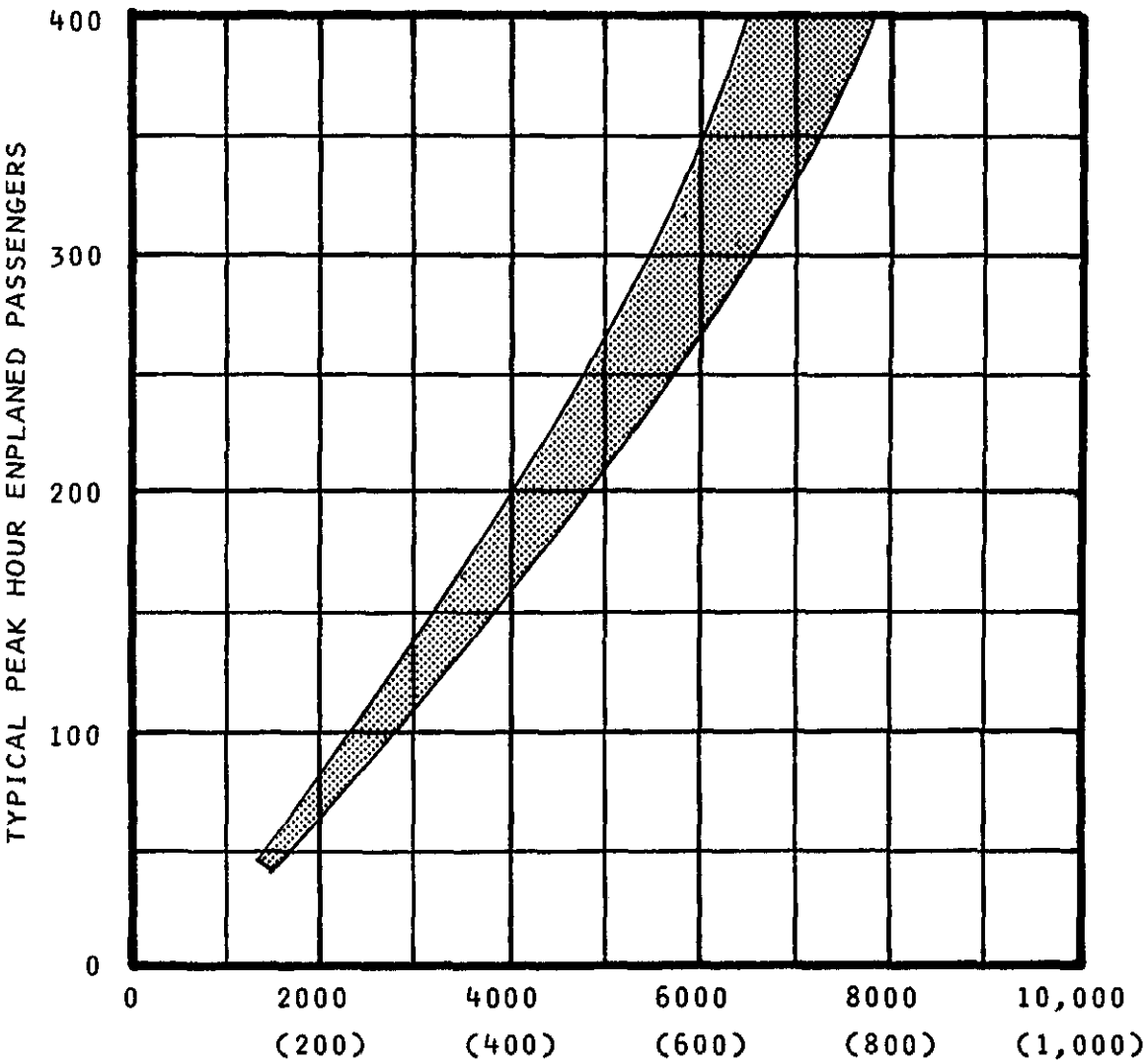
AIRLINE OFFICE, OUTBOUND BAGGAGE AND OPERATIONAL SPACE IN SQUARE FEET AND (SQUARE METERS)
