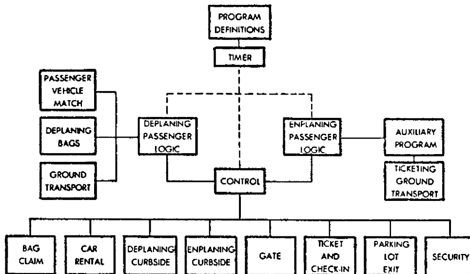
Figure 1. Flow Diagram of the Airport Landside Simulation Model Program
