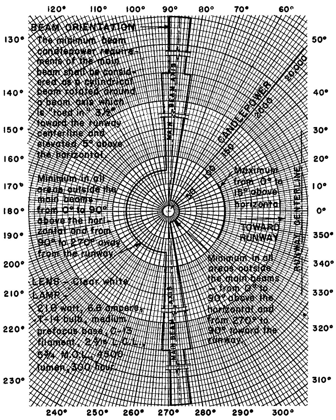
FIGURE 1. HORIZONTAL DISTRIBUTION AT 5° ABOVE THE HORIZONTAL
