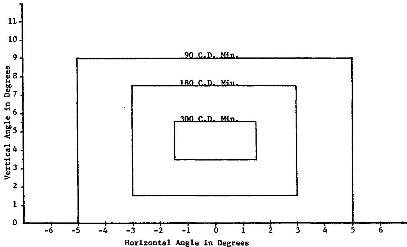
FIGURE 4. ISOCANDELA CURVE FOR MINIMUM OUTPUT IN GREEN LIGHT FOR L-861-E MEDIUM INTENSITY THRESHOLD LIGHT.
