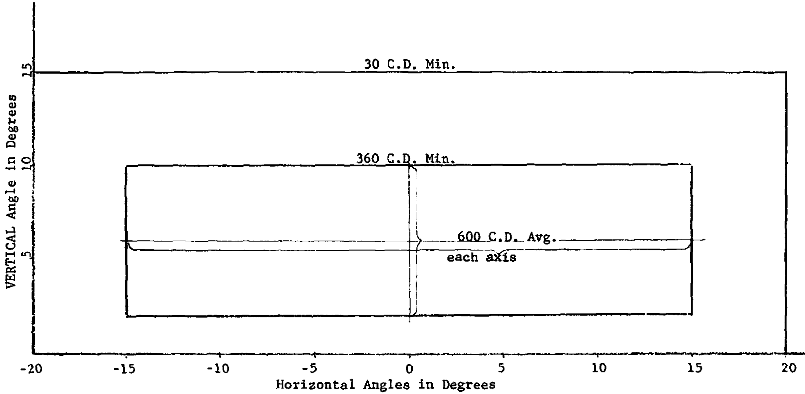
FIGURE 3. Isocandela Curve for Minimum Output in Green Light for L-861-ES Medium Intensity Threshold Light.
