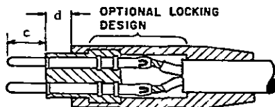
PLUG, e&f Assembled, Style 5
