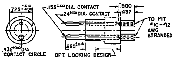
a - INSERT ASSEMBLY
