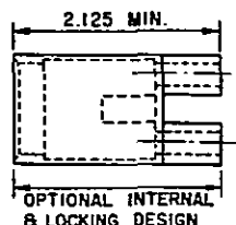
b - HOUSING
