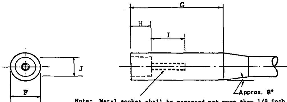
(b) RECEPTACLE, Type I, Class A, Style 9
