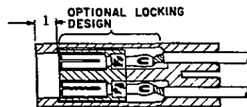
RECEPTACLE, c&d Assembled, Style 11
