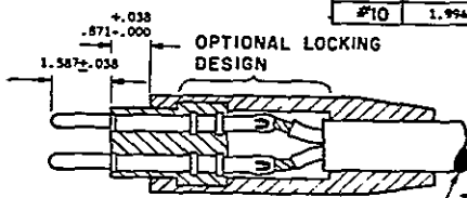
PLUG, e&f Assembled, Style 5 RECEPTACLE, g&h Assembled, Style 12
