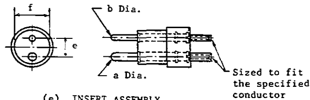
(e) INSERT ASSEMBLY
