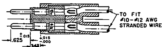
PLUG, a&amp;b Assembled, Style 4
