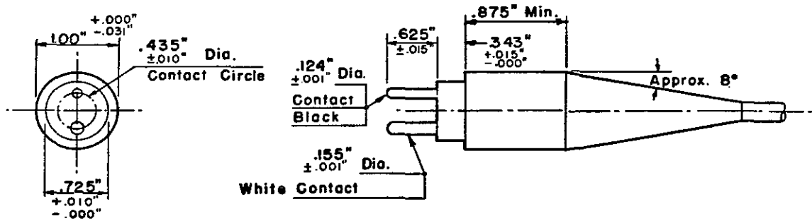
(a) PLUG, Type II, Class A, Style 1
