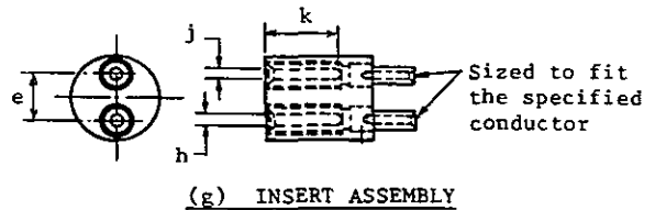
(g) INSERT ASSEMBLY
