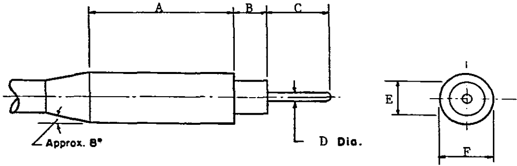
(a) PLUG, Type I, Class A, Style 2
