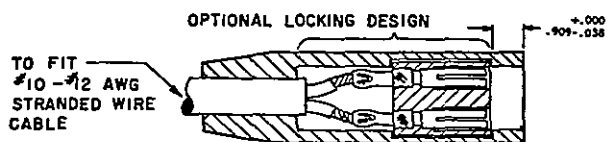
PLUG, e&f Assembled, Style 5 RECEPTACLE, g&h Assembled, Style 12
