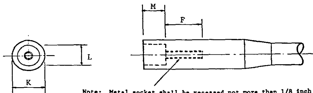
RECEPTACLE, Type I, Class A, Style 9
