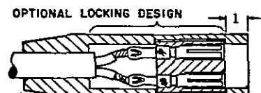
RECEPTACLE, g&h Assembled, Style 12
