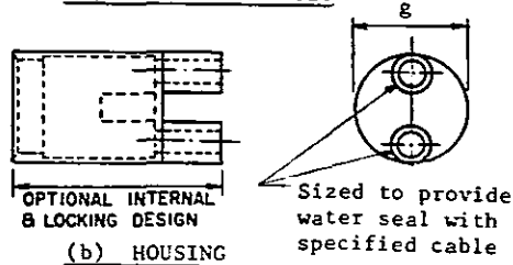
(b) HOUSING
