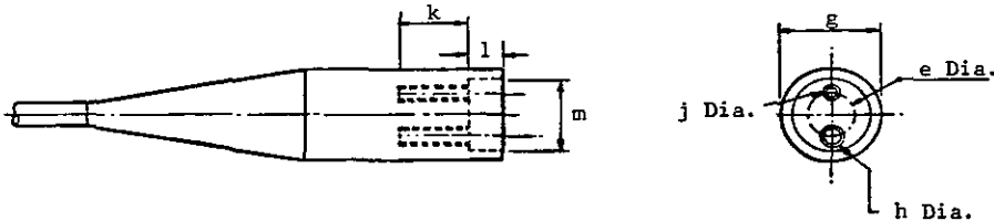
(b) RECEPTACLE, Type II, Class A, Style 7
