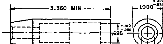
h - HOUSING
