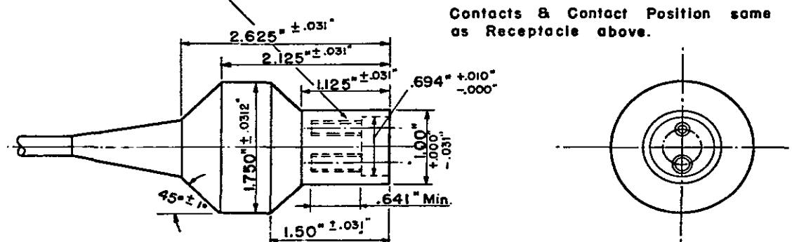
(c) RECEPTACLE, Type II, Class A, Style 8
