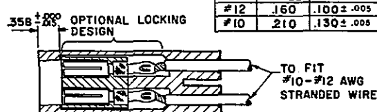
RECEPTACLE, c&amp;d Assembled, Style 11
