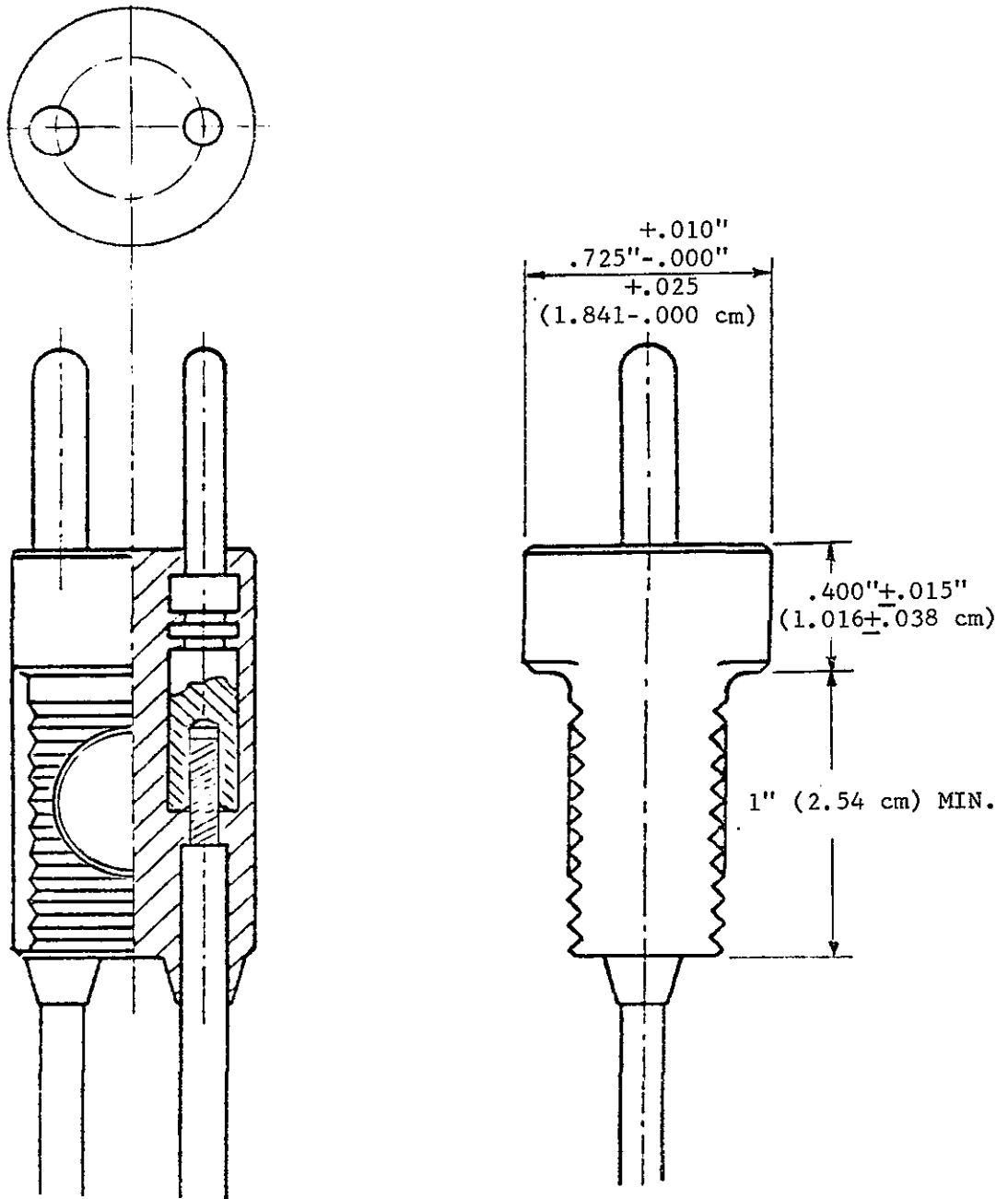
Figure 5. Plug, Two Single Conductors, 20 Ampere, 600 Volts Between Contacts, 1500 Volts to Ground, Type II, Class A, Style 6.
