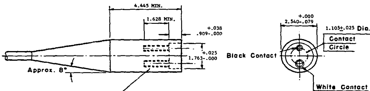
(b) RECEPTACLE, Type II, Class A, Style 7
