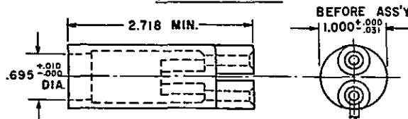
d - HOUSING
