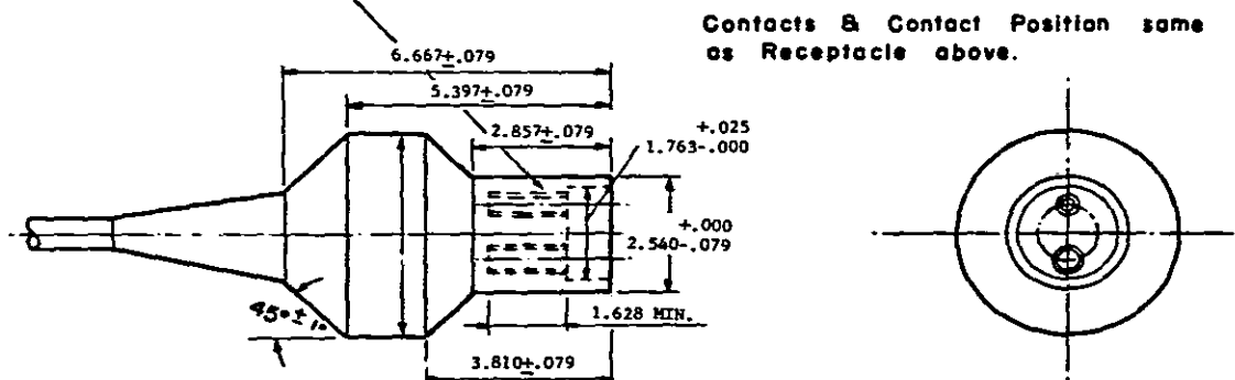
(c) RECEPTACLE, Type II, Class A, Style 8
