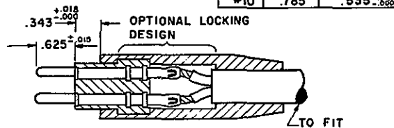
PLUG, e&amp;f Assembled, Style 5
