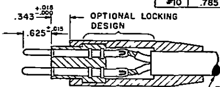
PLUG, e&amp;f Assembled, Style 5
