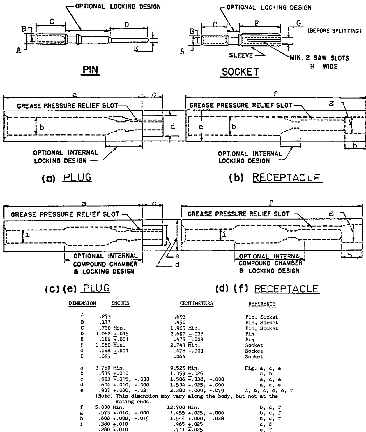
Figure 3. Plug, Type I, Class B, Style 3, and Receptacle, Type I, Class B, Style 10, Single Conductor, 5000 Volt, 25 Ampere.
