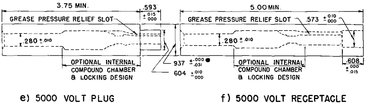
FIGURE 14. PLUG AND RECEPTACLE KIT (SINGLE CONDUCTOR, 25 AMPERE).
