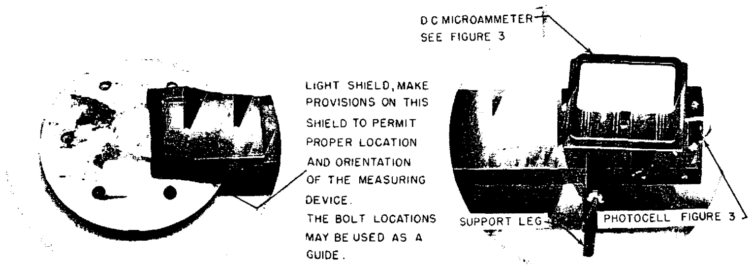
FIGURE 4. MEASUREMENT DEVICE
