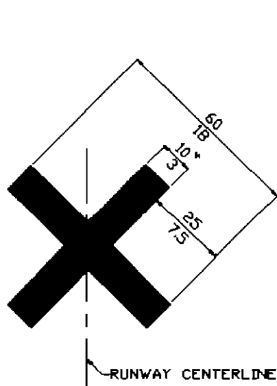
(A) CLOSED RUNWAY
