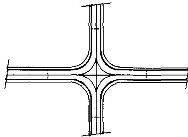
B. EXAMPLE OF TAXIWAY CENTERLINE MARKING AT INTERSECTION HAVING STANDARD FILLETS WHICH PERMITS COCKPIT-OVER-CENTERLINE STEERING
