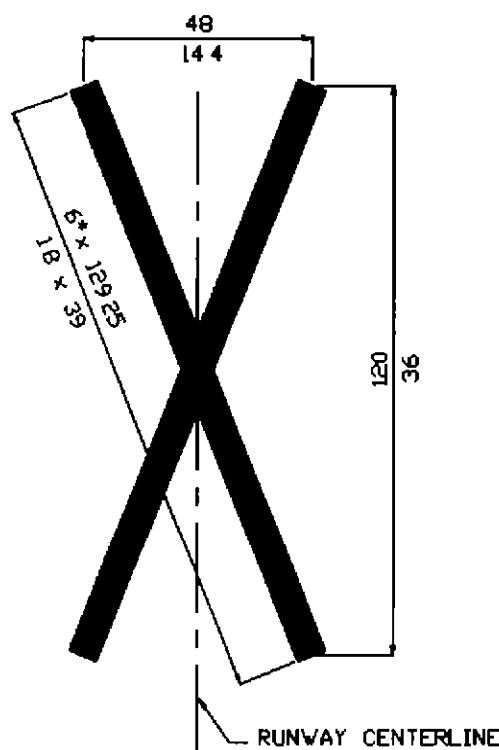
(B) ALTERNATE CLOSED RUNWAY
