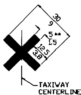
(C) CLOSED TAXIWAY
