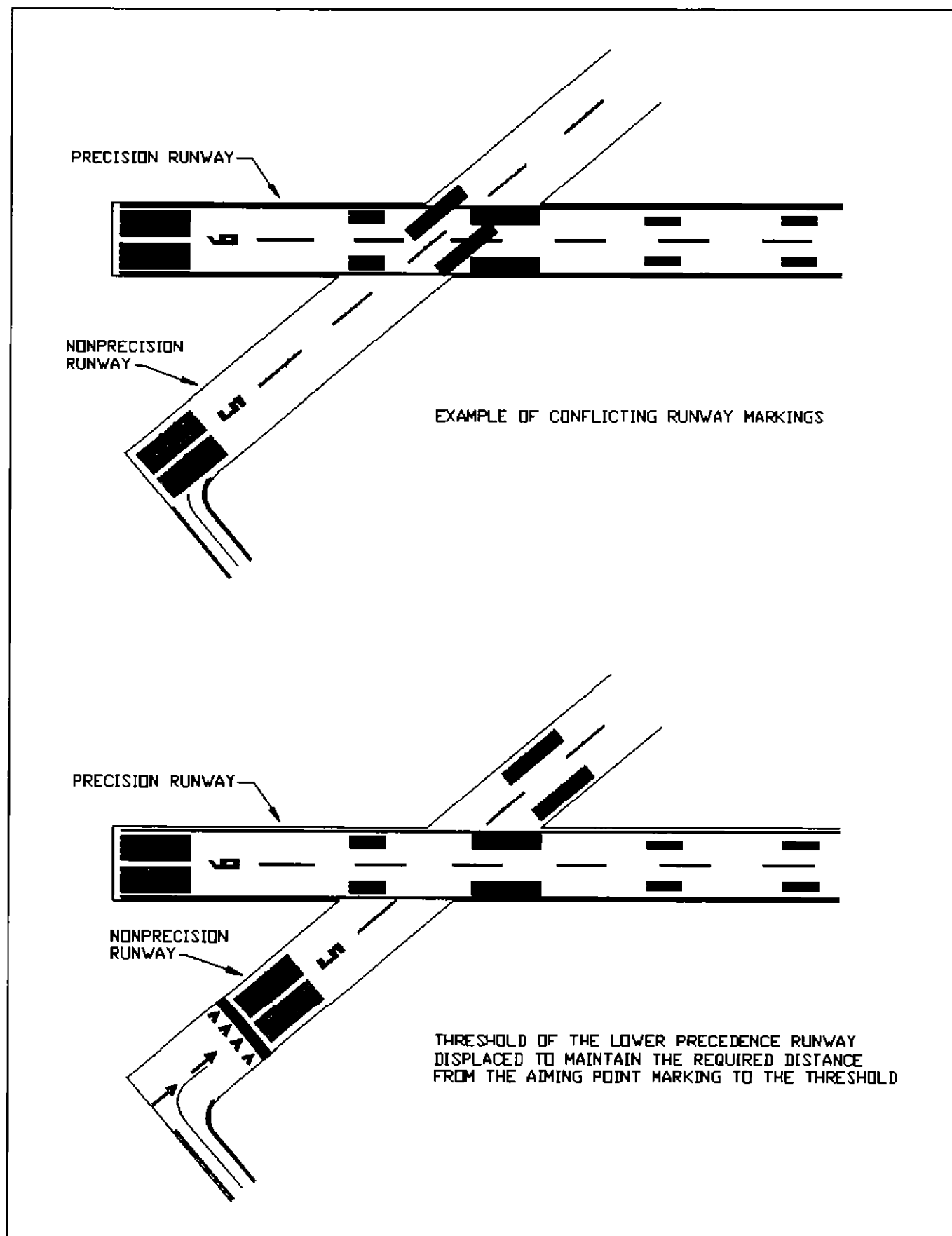
Figure 3 Example of Markings on Crossing Runways
