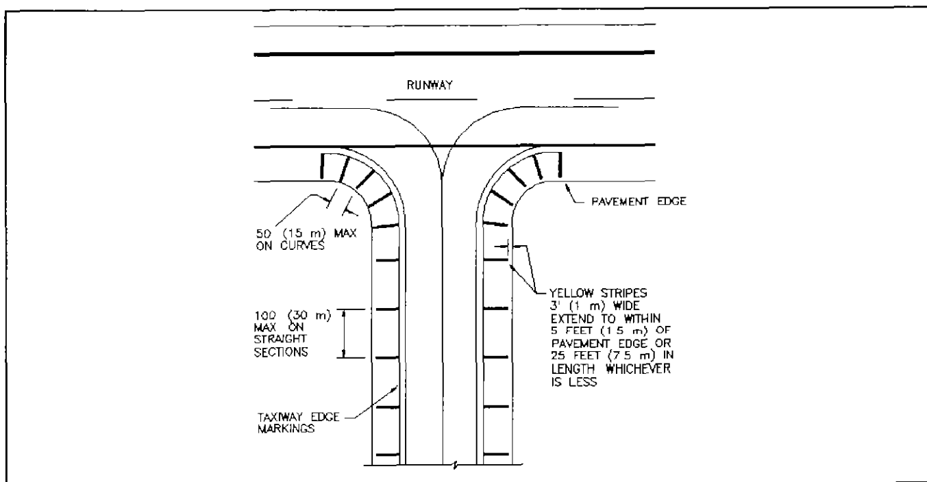
Figure 14 Taxiway Shoulder Markings
