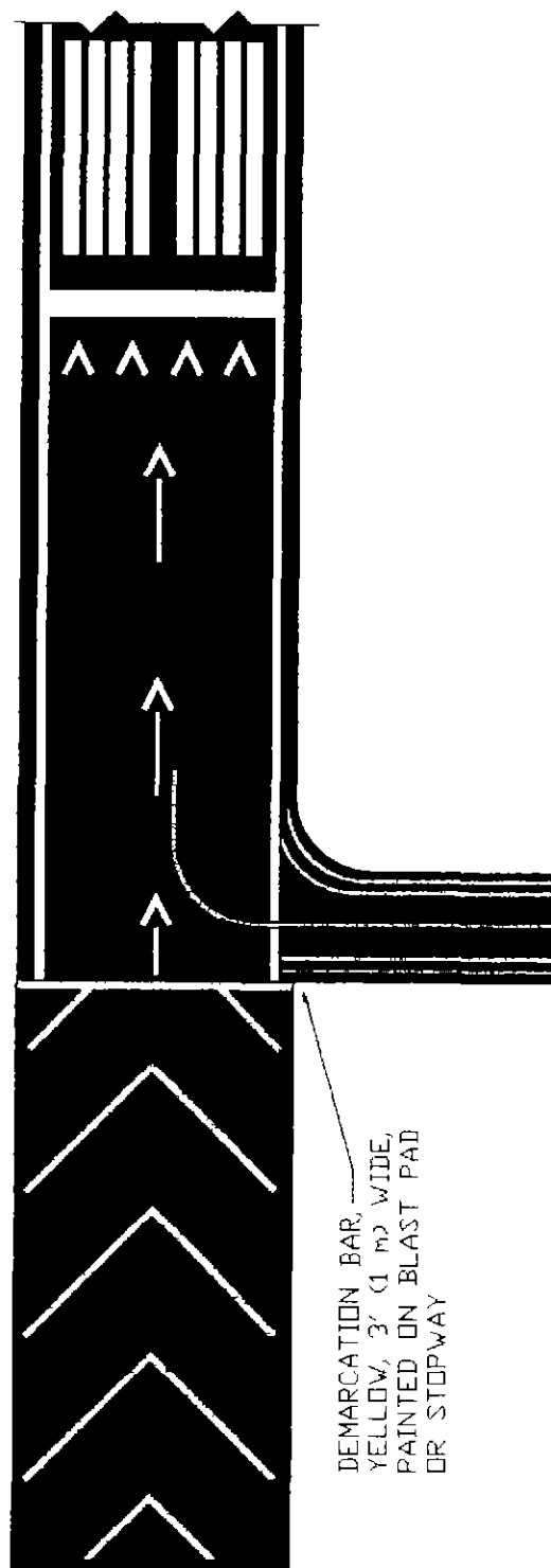
BLAST PAD OR STOPWAY AND DISPLACED THRESHOLD PRECEDING A RUNWAY
