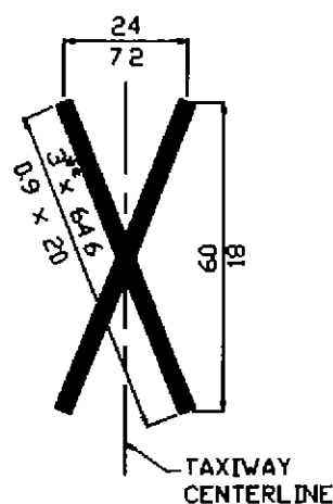
(D) ALTERNATE CLOSED TAXIWAY
