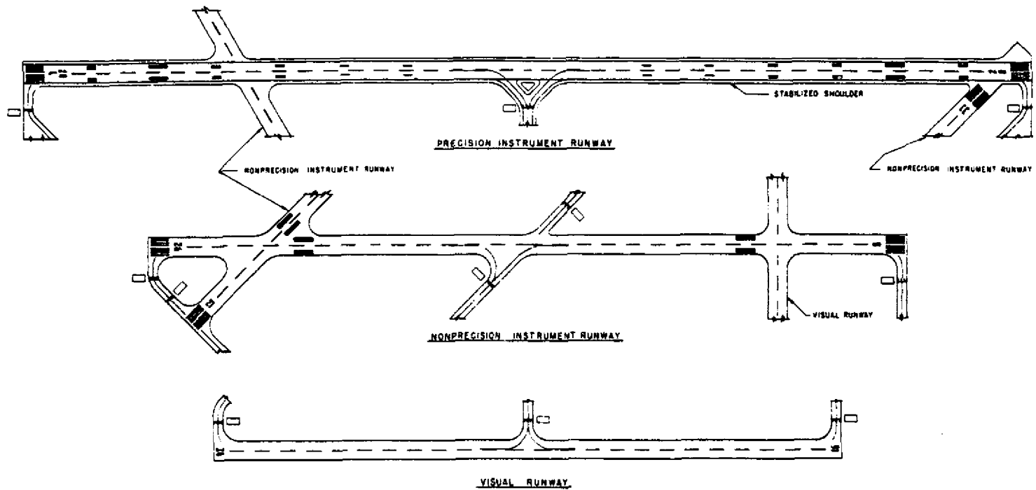
FIGURE 1 RUNWAY MARKINGS
