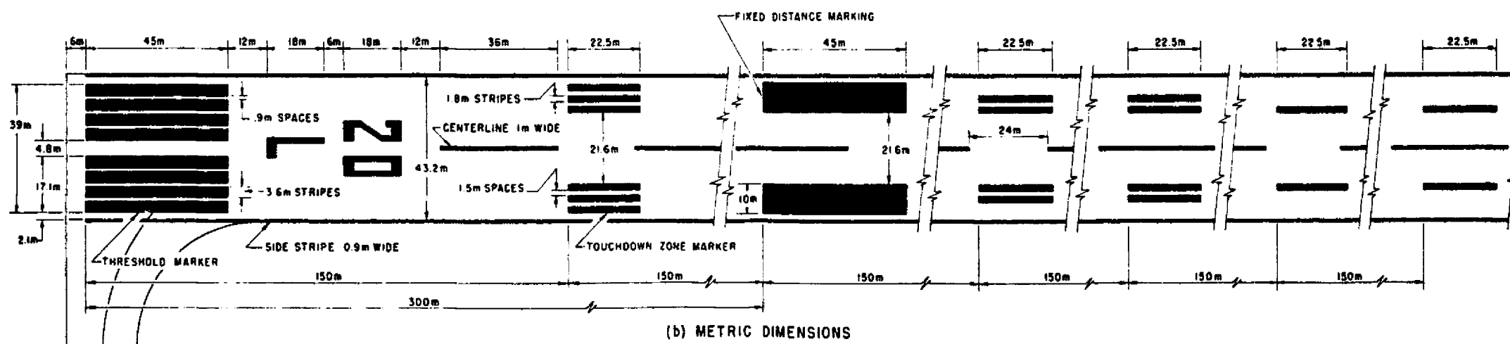
FIGURE 2 PRECISION INSTRUMENT RUNWAY MARKINGS
