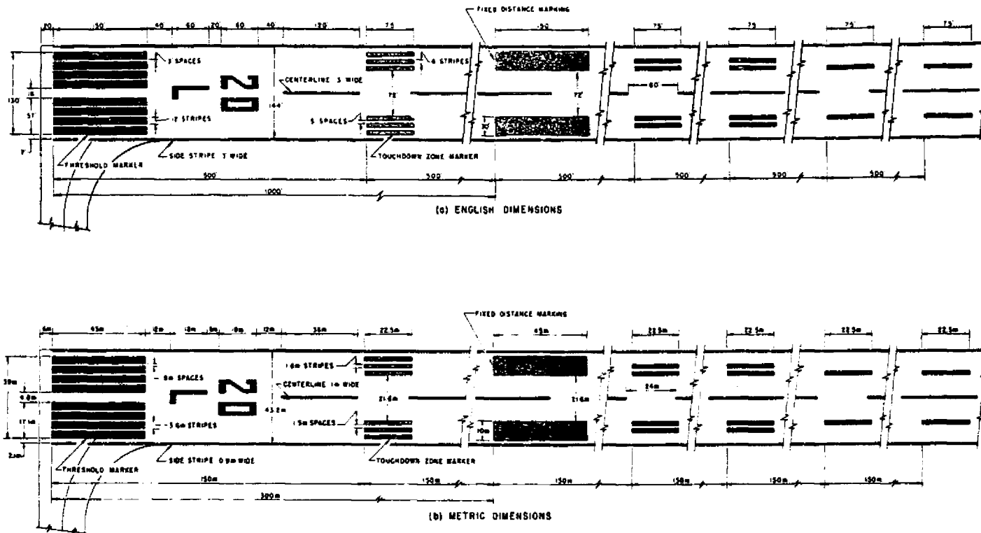
FIGURE 2. PRECISION INSTRUMENT RUNWAY MARKINGS.
