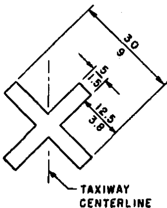
(c) CLOSED TAXIWAY
