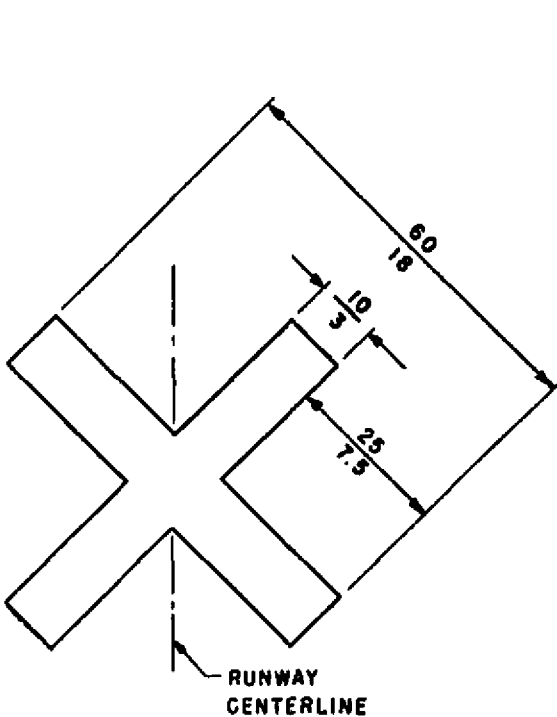
(a) CLOSED RUNWAY
