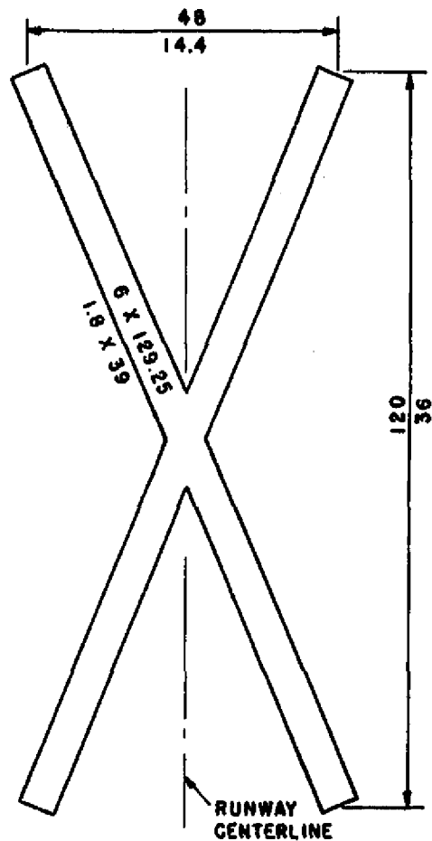
(b) ALTERNATE CLOSED RUNWAY
