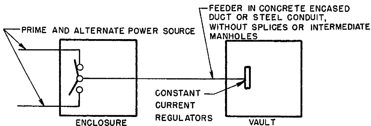
B-2 TRANSFER SWITCH ADJACENT TO VAULT
