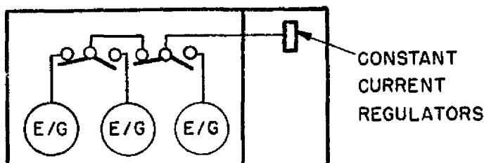
FIGURE 1A. CONFIGURATION "A" ELECTRICAL POWER
