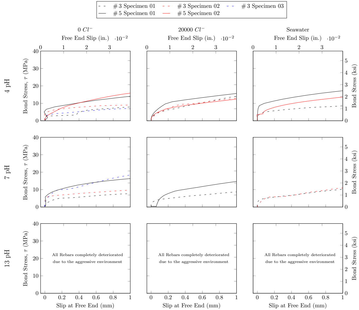
Figure 8.121: Bond stress - slippage behavior of rebar Type C Lot 2 rebars
