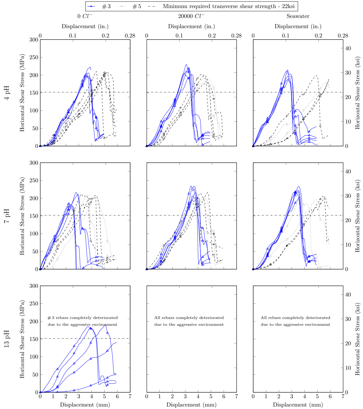
Figure 7.84: 300Day Transverse shear stress - displacement behavior of Type A Lot1 tested rebars
