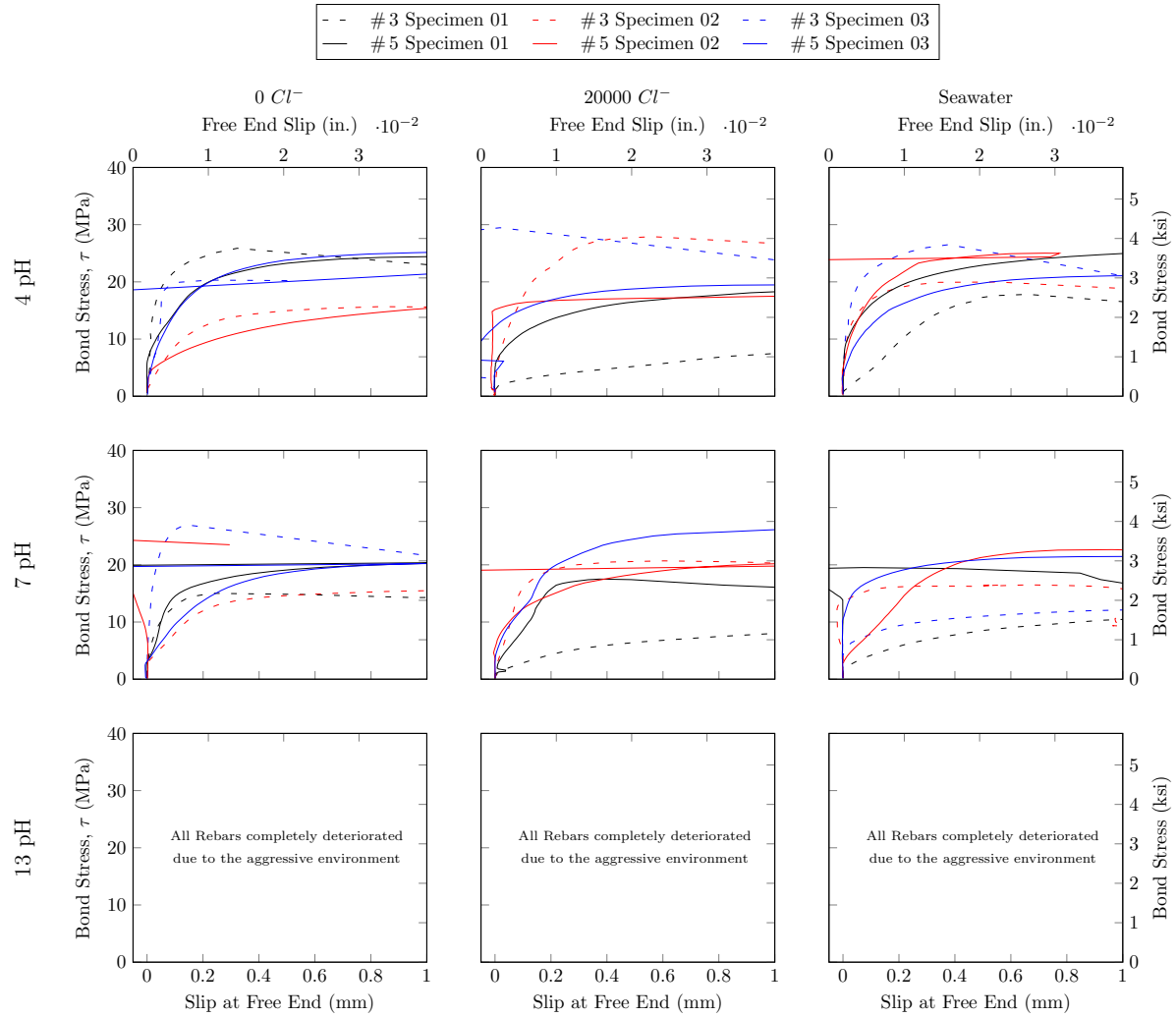
Figure 7.114: Bond stress - slippage behavior of rebar Type A Lot 1 rebars
