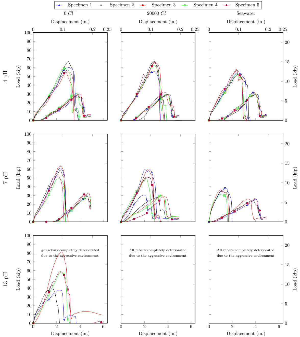
Figure 7.83: 300Day Transverse shear force - displacement behavior of Type C Lot2 tested rebars
