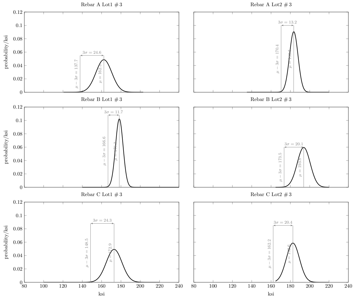
Figure 9.2: Gaussian distribution for tensile strength of #3 rebars
