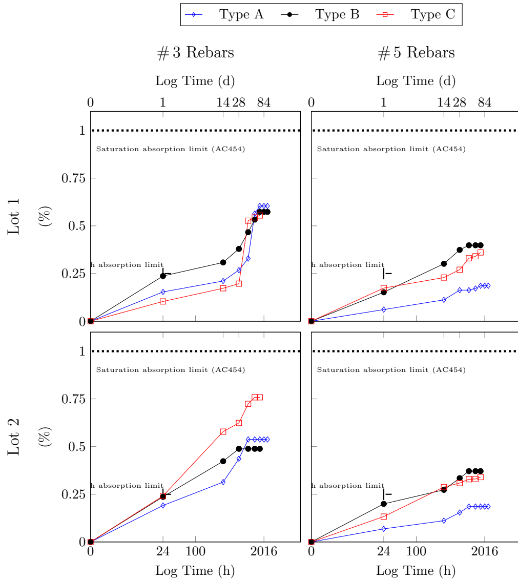
Figure 6.7: Moisture absorption results of rebar from all manufacturers
