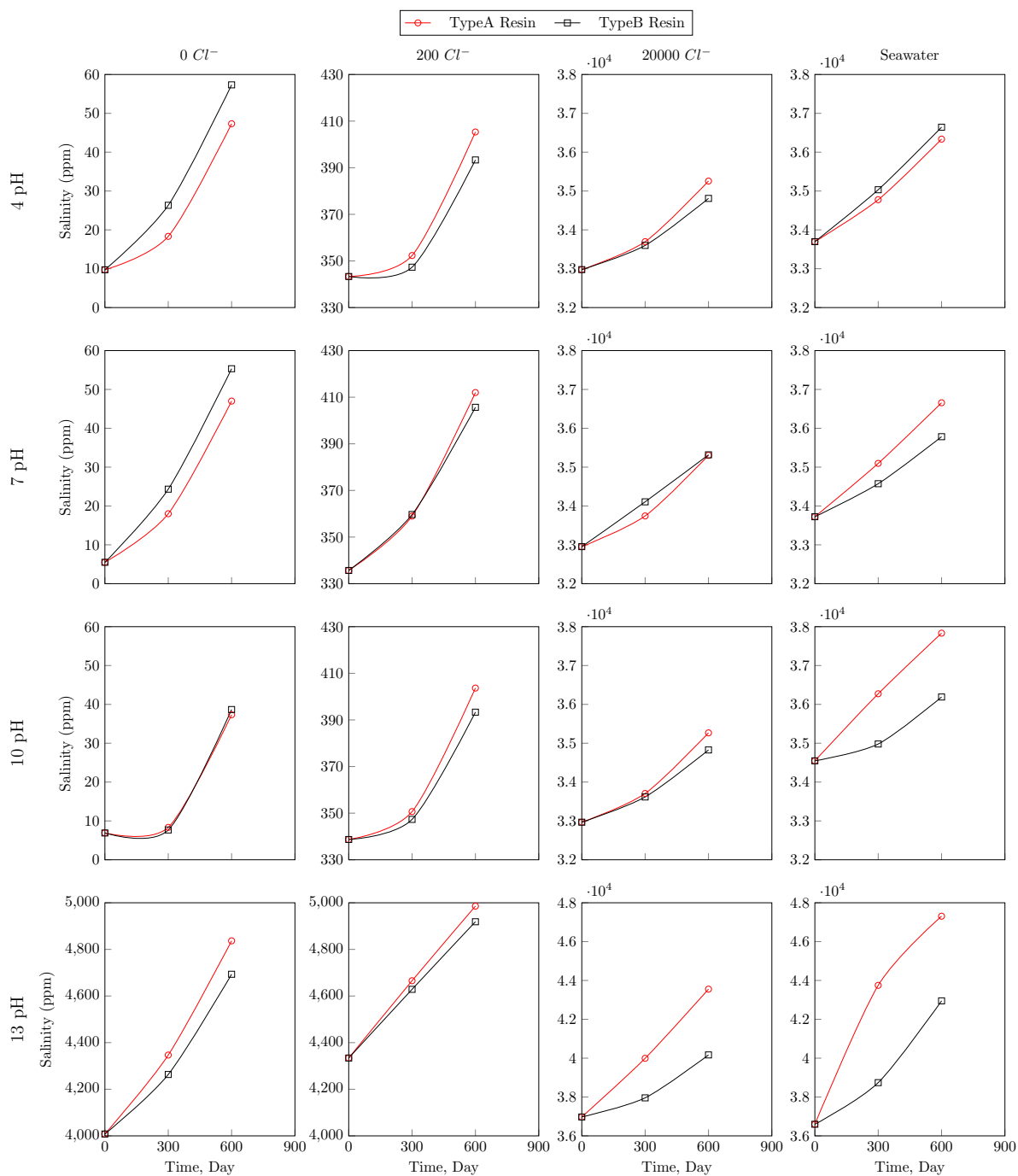
Figure 7.5: Salinity of environments after exposure of resins
