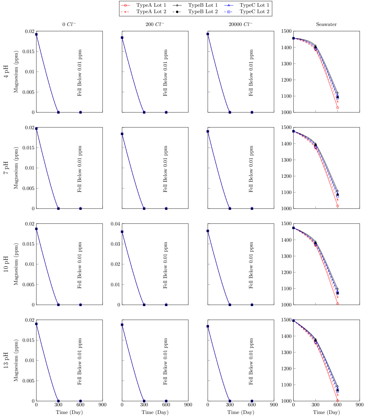
Figure 7.31: Magnesium concentration of all environments after exposure of rebars
