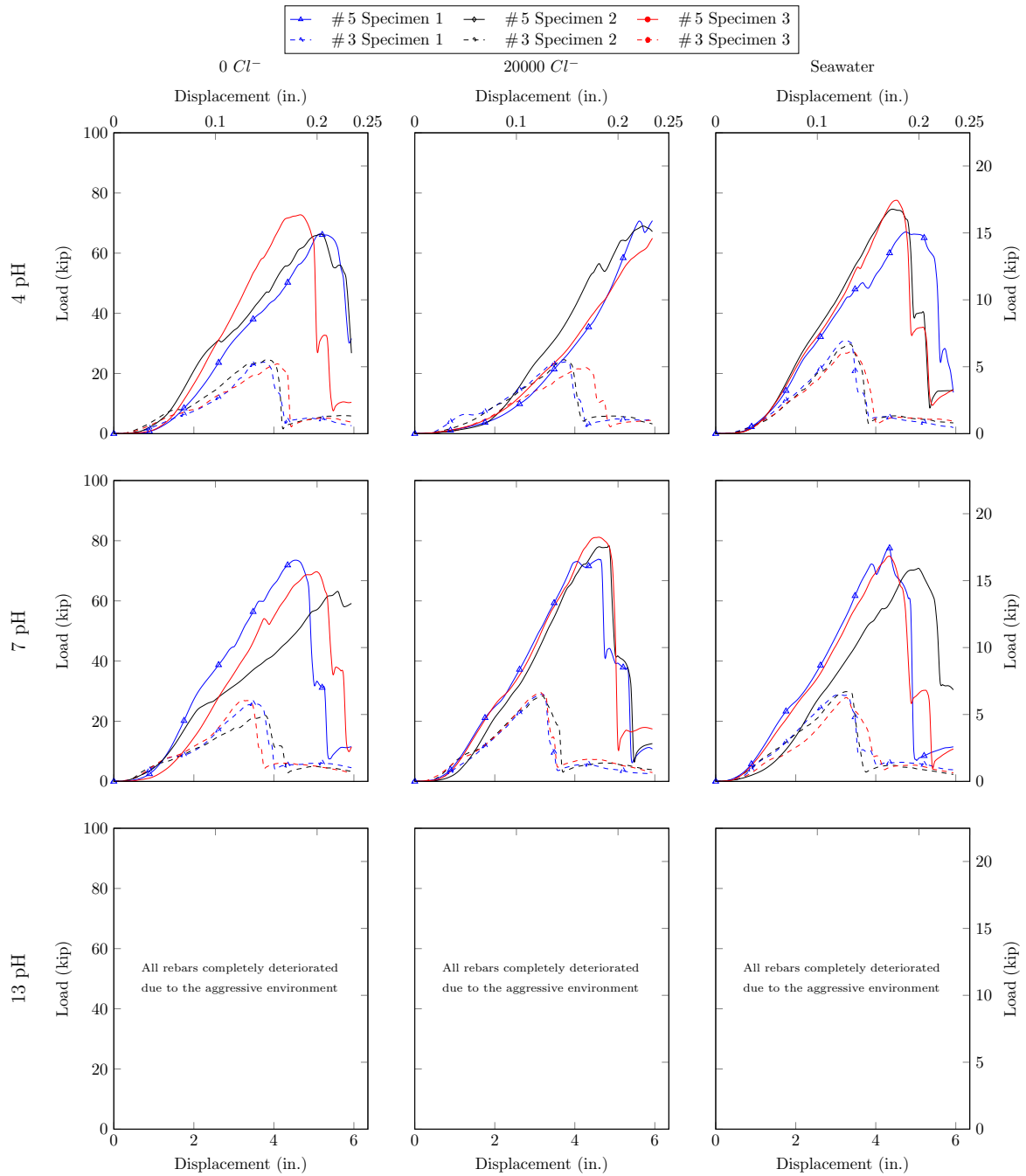
Figure 8.82: 600Day Transverse shear force - displacement behavior of Type C Lot1 tested rebar
