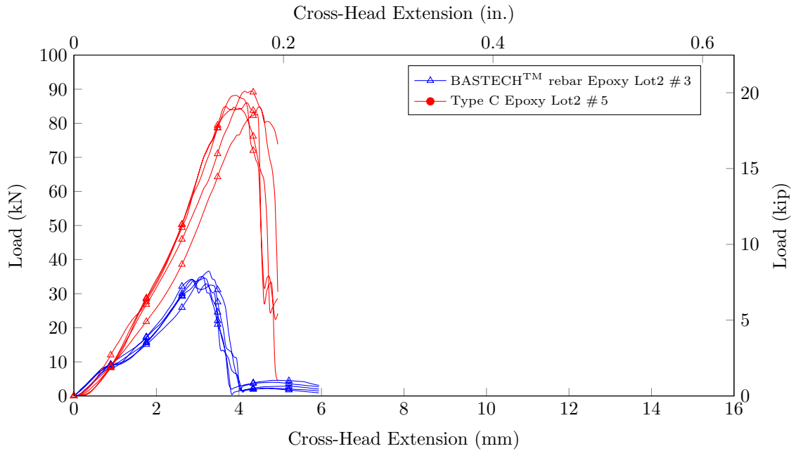
Figure 6.13: Extension-transverse shear load behavior of Type C rebars Lot 2 size 3 and 5
