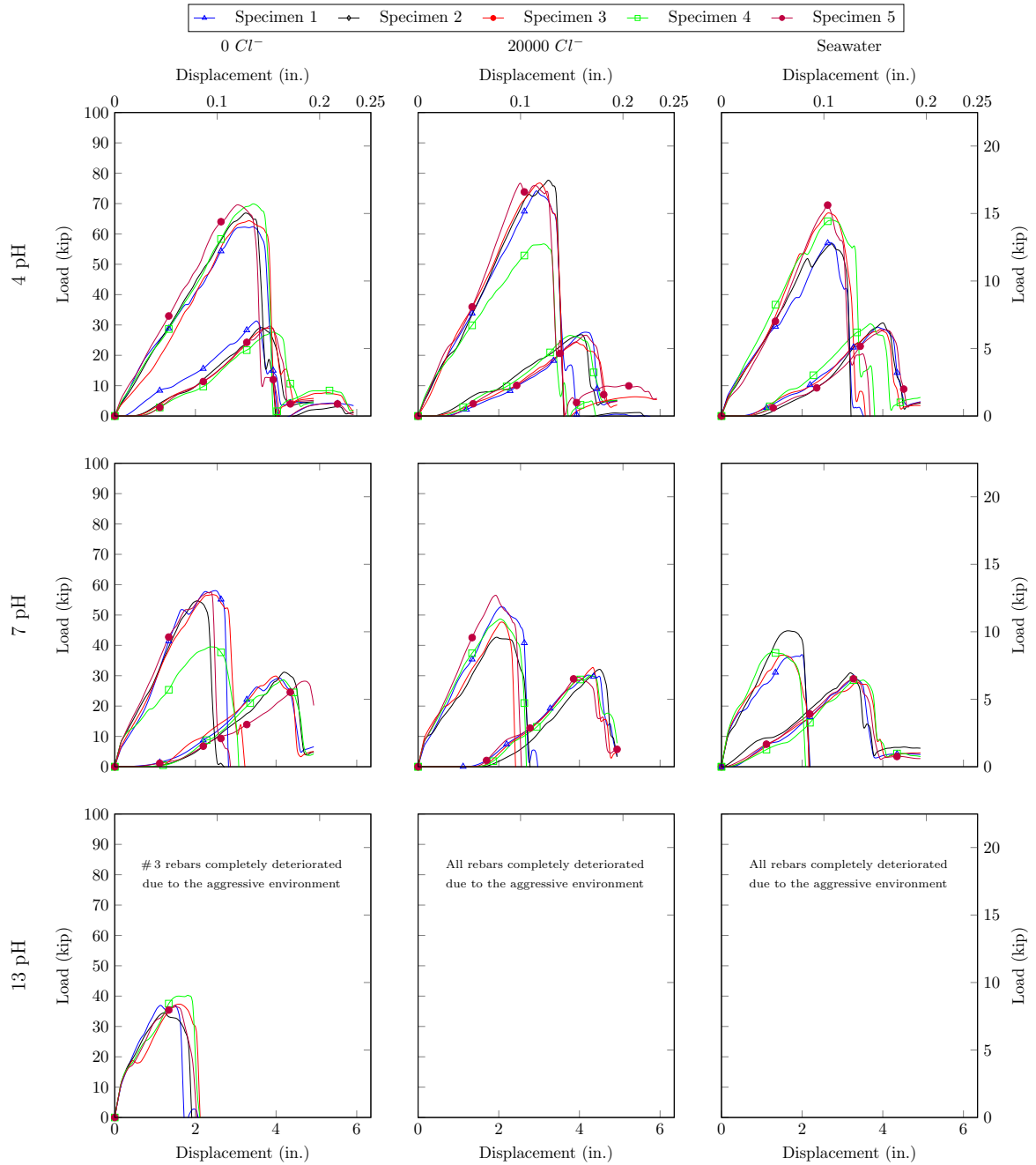
Figure 7.80: 300Day Transverse shear force - displacement behavior of Type C Lot1 tested rebars
