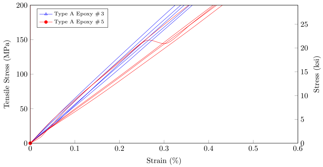
Figure 6.43: Tensile stress-strain behavior of rebar Type A Lot 2 rebar size 3 and 5
