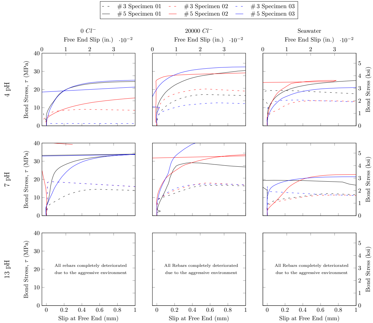
Figure 8.117: Bond stress - slippage behavior of rebar Type B Lot 1 rebars
