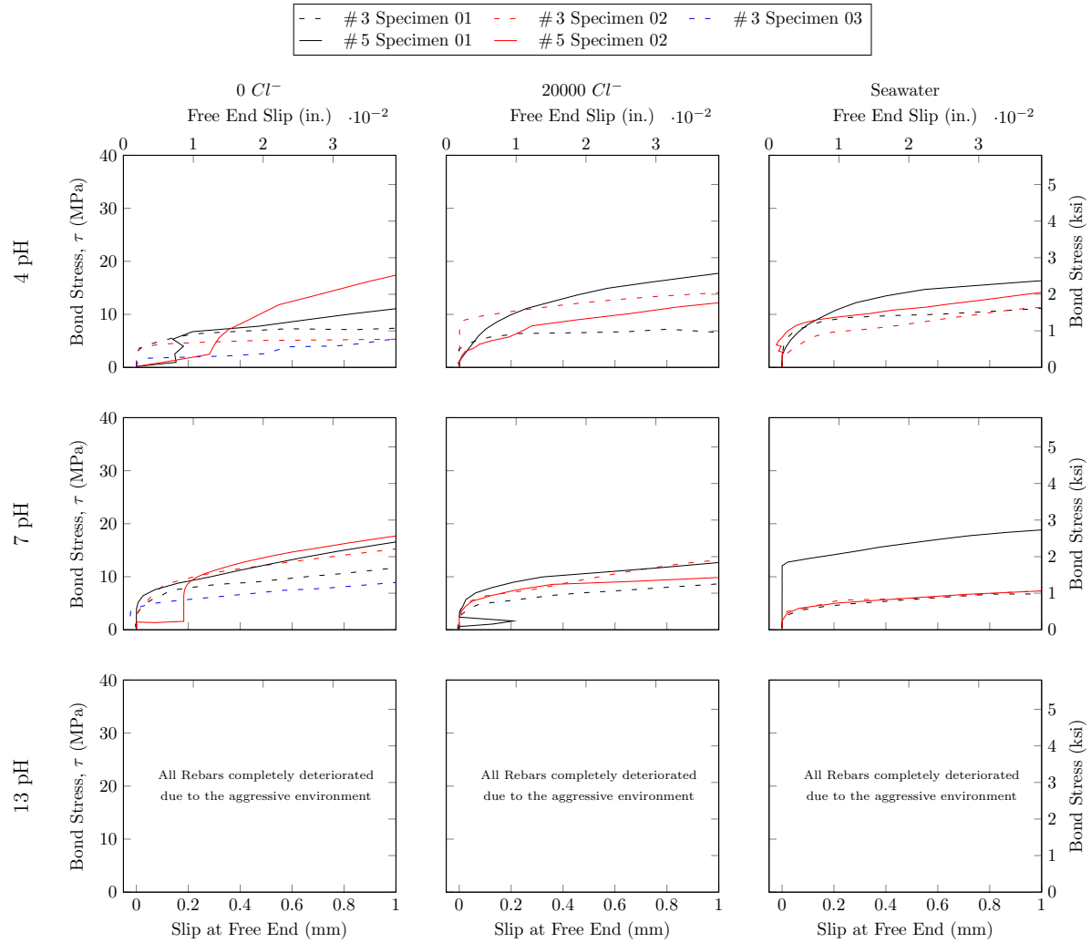
Figure 8.118: Bond stress - slippage behavior of rebar Type C Lot 1 rebars
