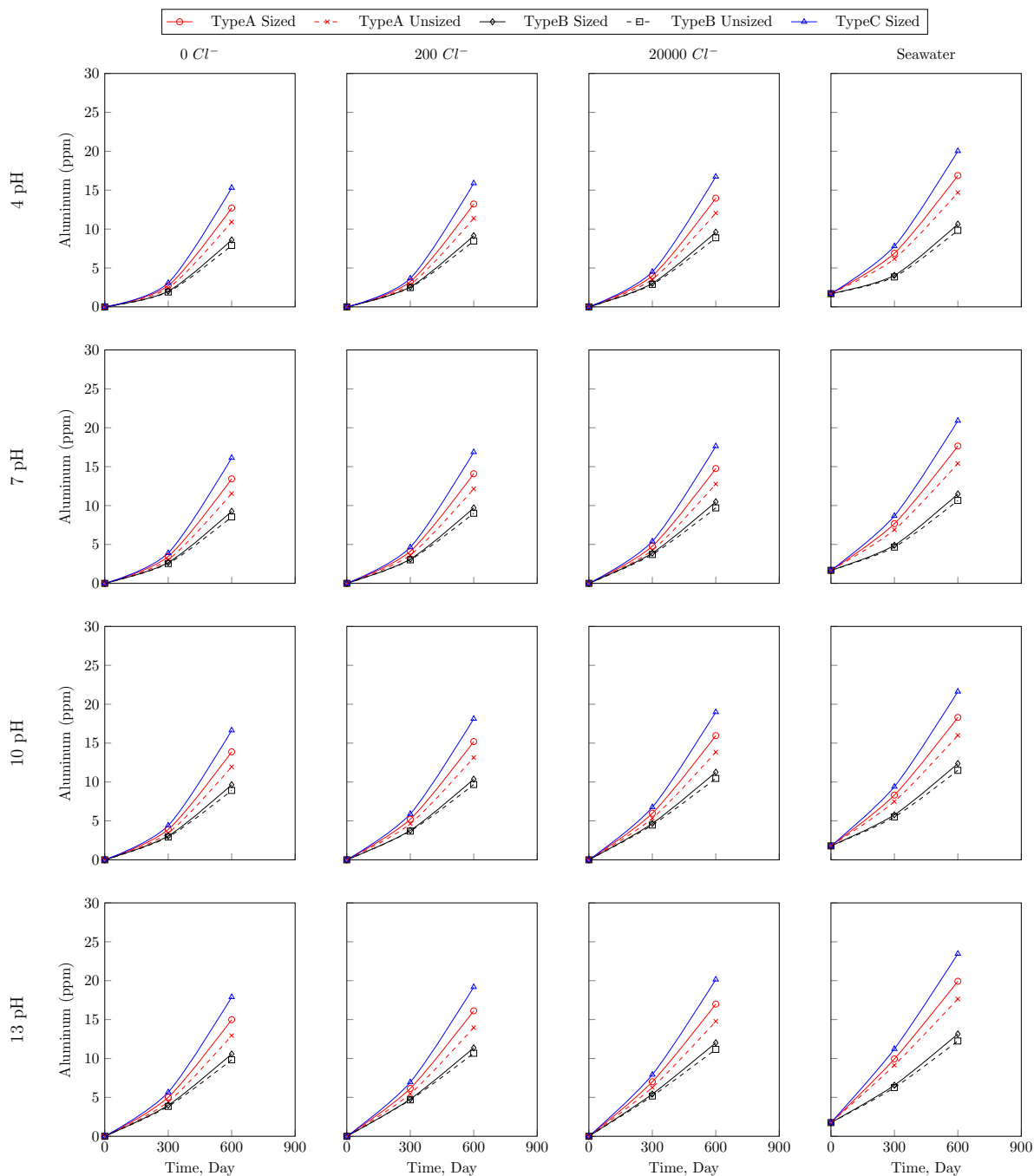
Figure 7.21: Aluminum concentration of all environments after exposure of sized and unsized fibers
