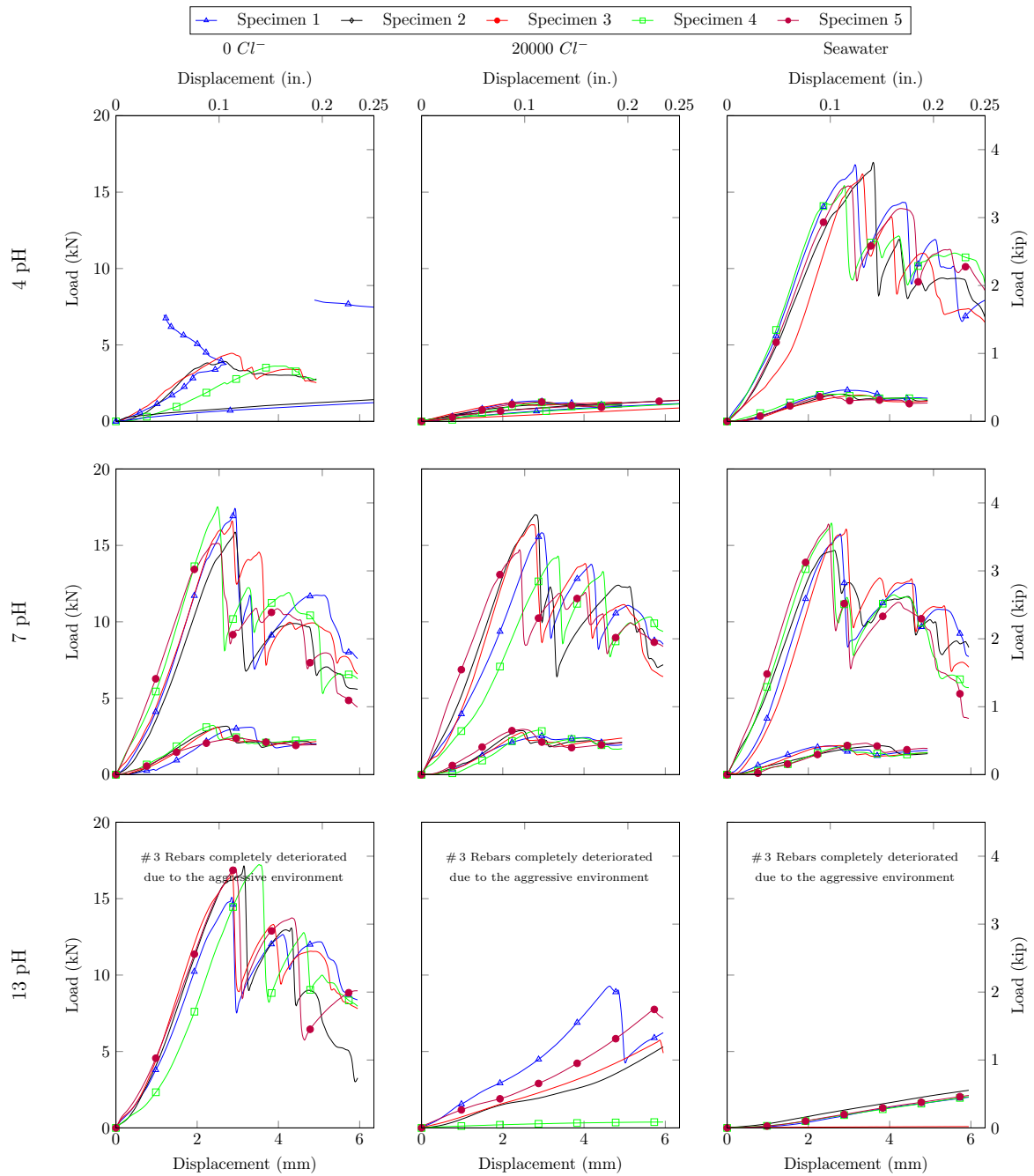
Figure 7.93: 300Day Horizontal shear force - displacement behavior of Type A Lot2 tested rebars
