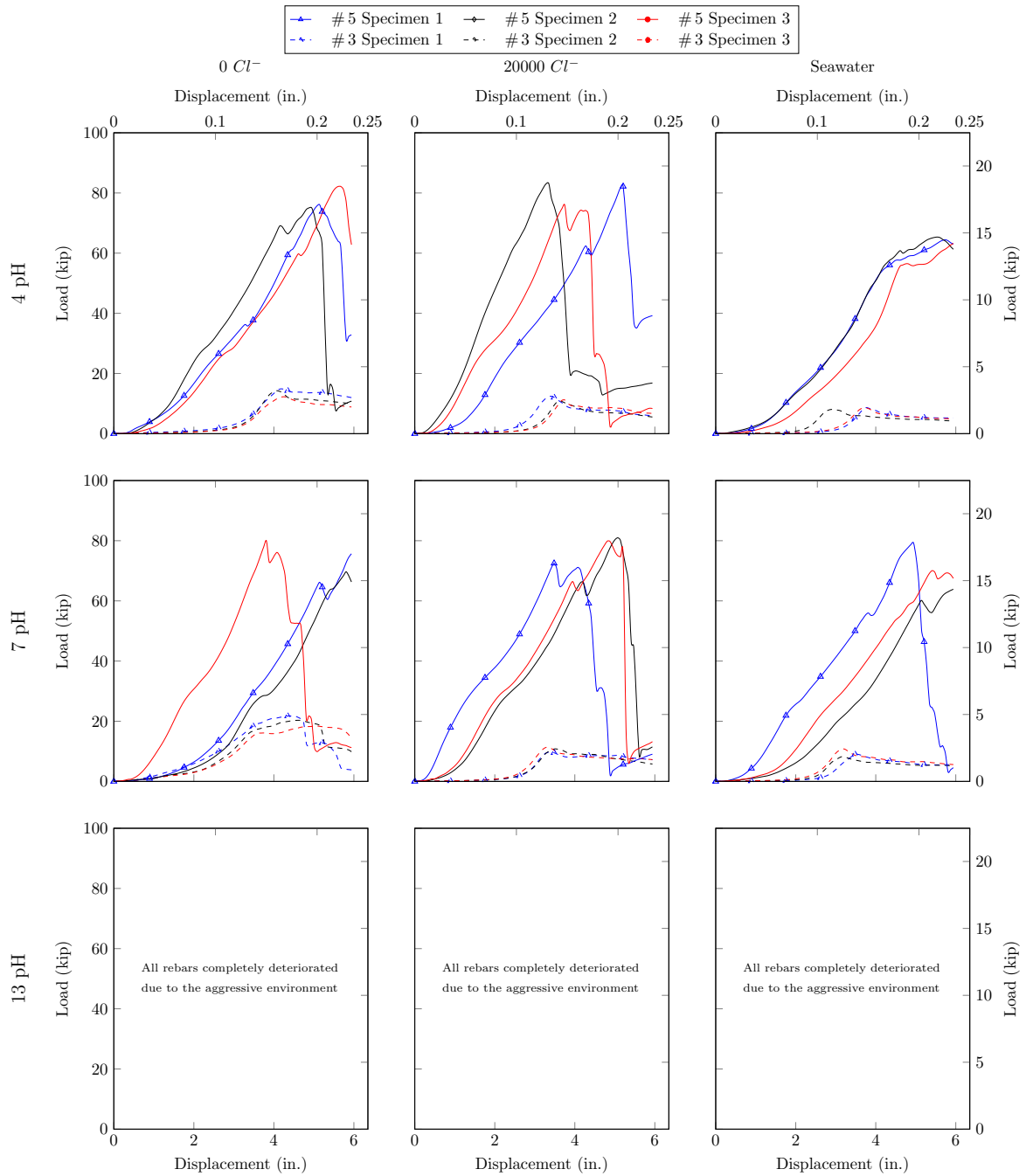
Figure 8.83: 600Day Transverse shear force - displacement behavior of Type A Lot2 tested rebar
