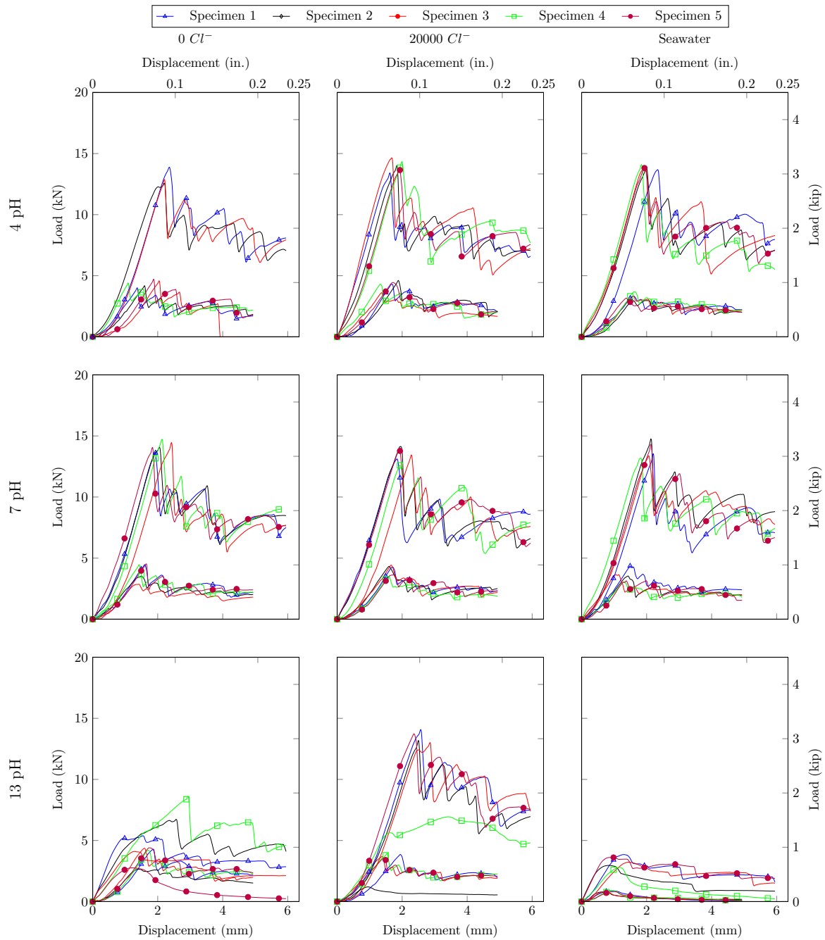
Figure 7.91: 300Day Horizontal shear force - displacement behavior of Type B Lot1 tested rebars
