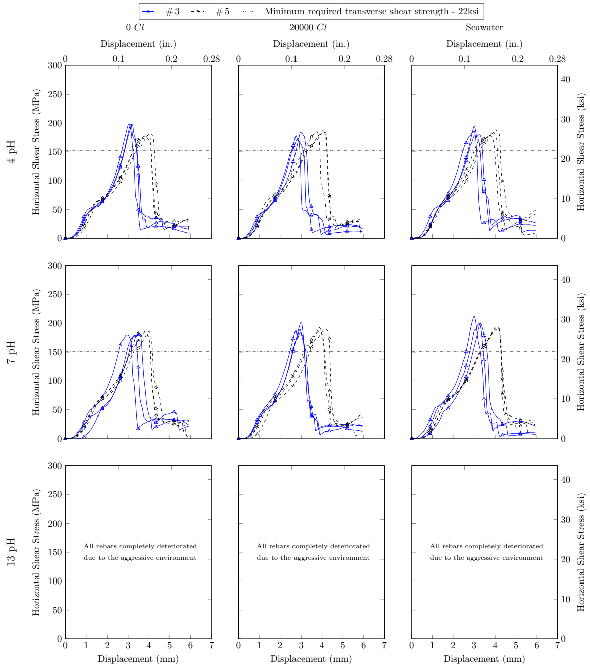
Figure 8.87: 600Day Transverse shear stress - displacement behavior of Type B Lot1 tested rebars
