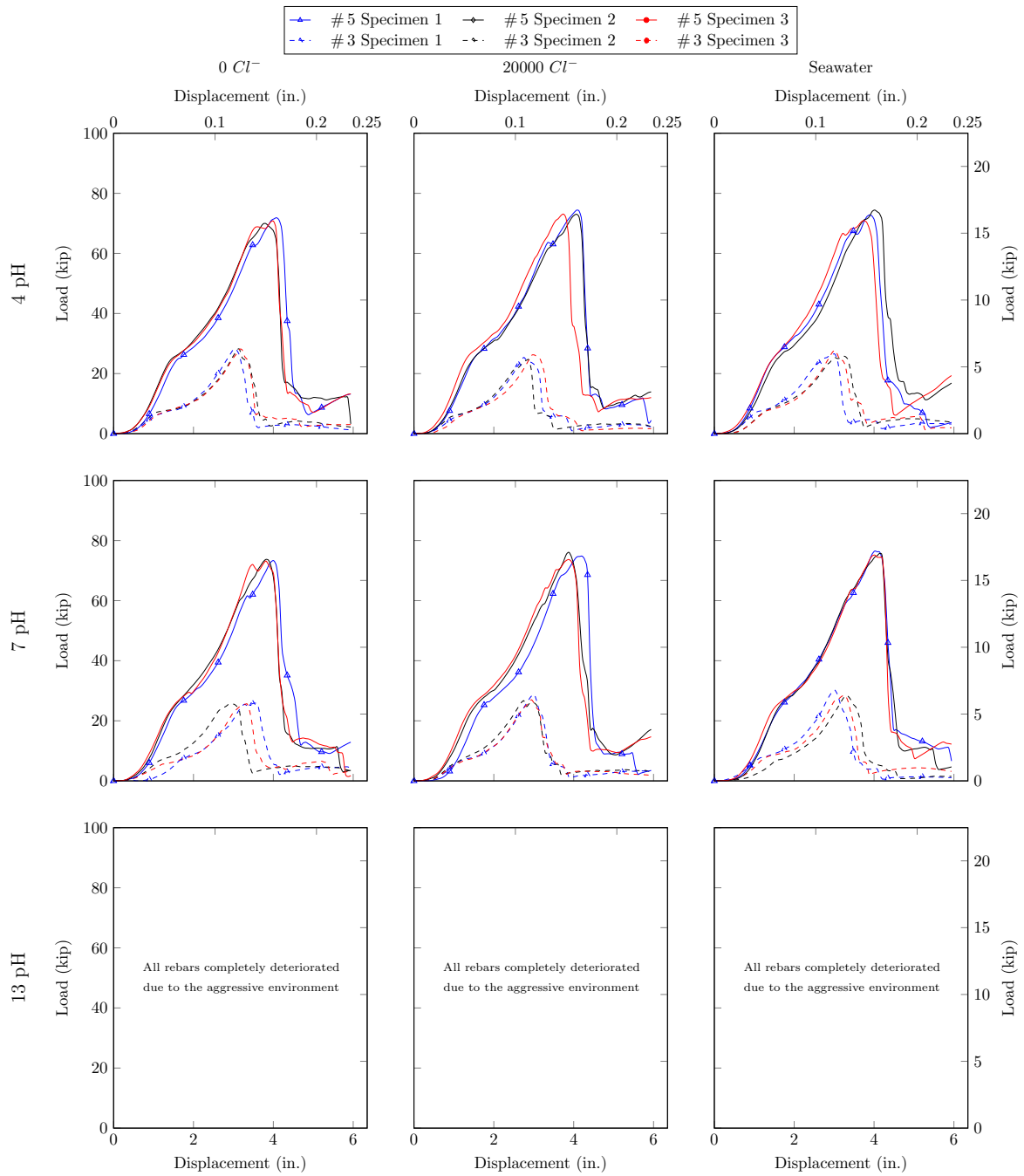
Figure 8.81: 600Day Transverse shear force - displacement behavior of Type B Lot1 tested rebars
