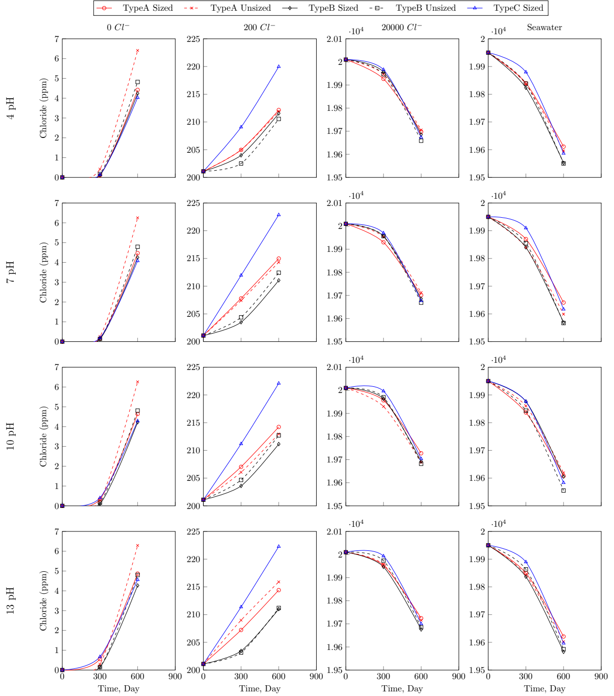
Figure 7.15: Chloride concentration of all environments after exposure of sized and unsized fibers
