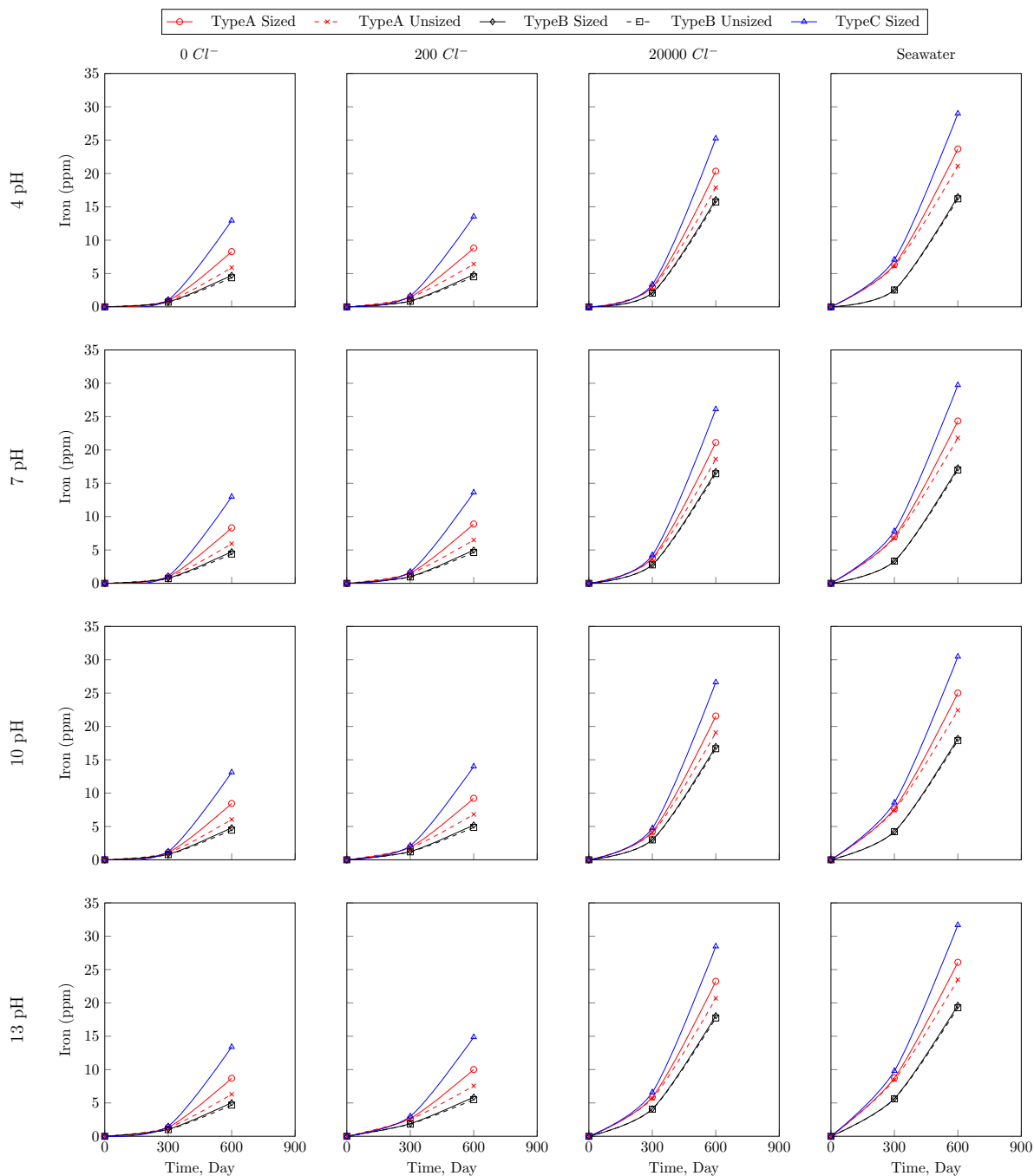
Figure 8.30: Iron concentration of all environments after exposure of sized and unsized fibers
