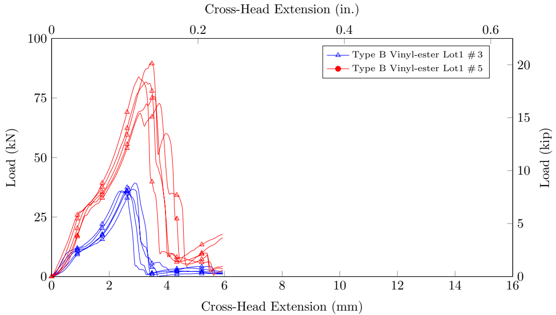
Figure 6.9: Extension-transverse shear load behavior of Type B rebars Lot 1 size 3 and 5
