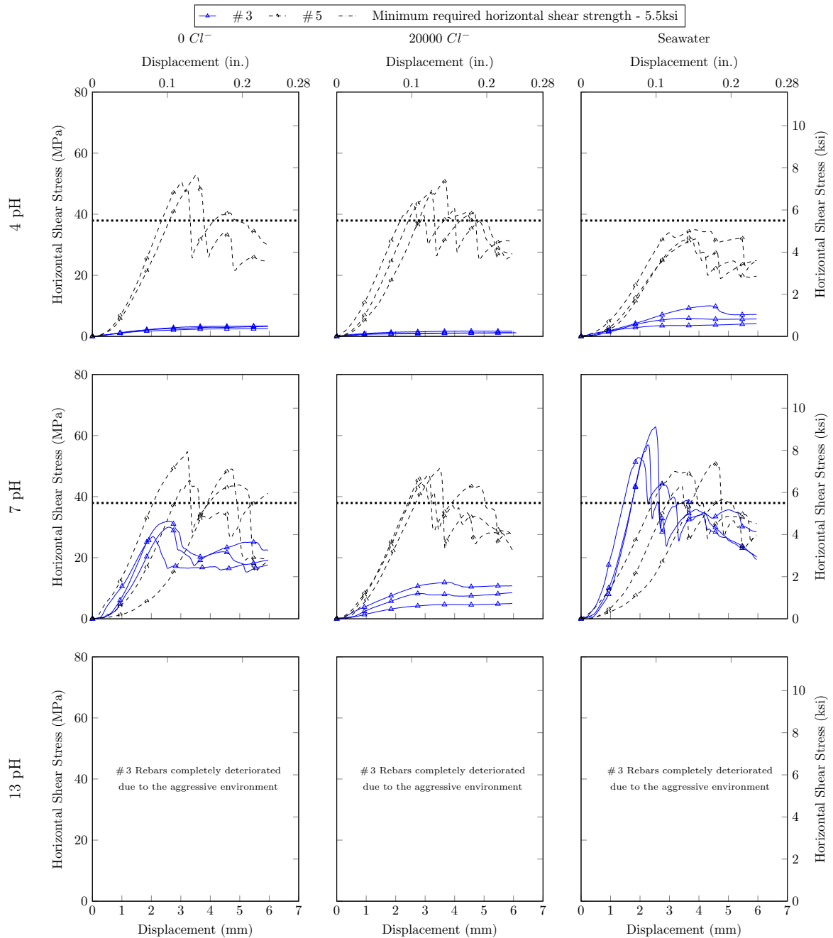
Figure 8.101: 600Day Horizontal shear stress - displacement behavior of Type A Lot2 tested rebars
