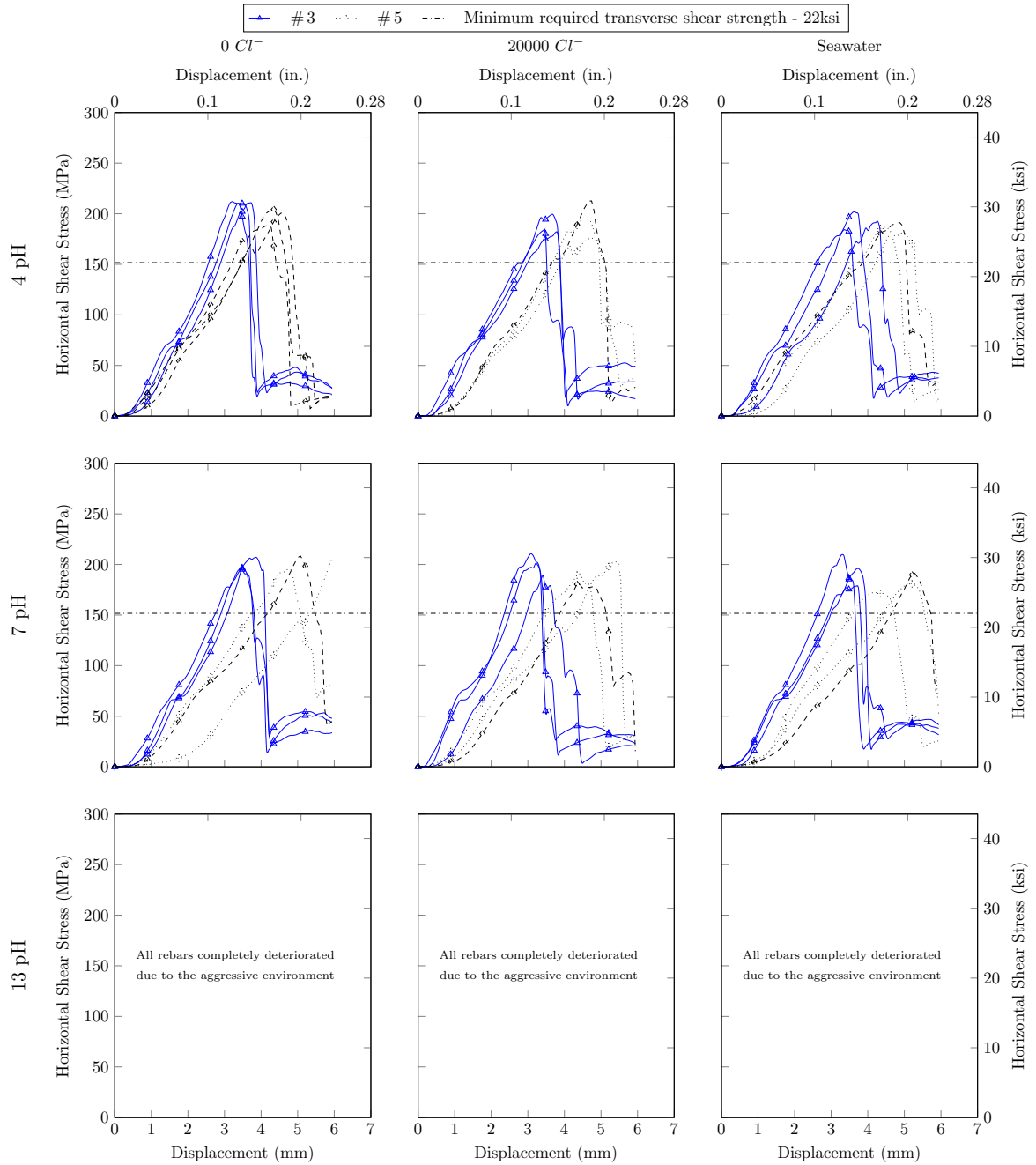
Figure 8.86: 600Day Transverse shear stress - displacement behavior of Type A Lot1 tested rebars
