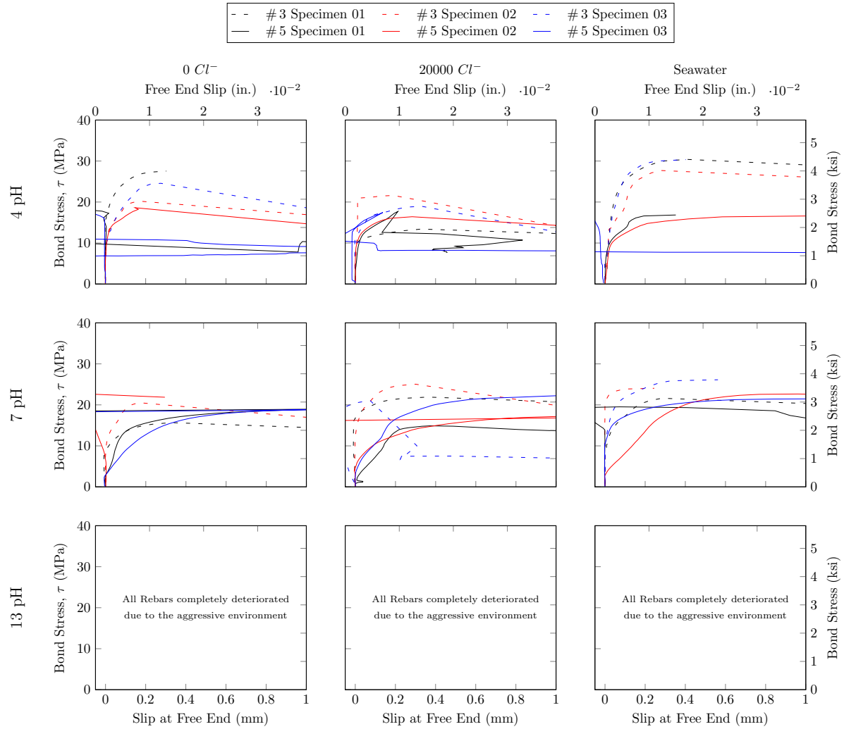
Figure 7.118: Bond stress - slippage behavior of rebar Type B Lot 2 rebars
