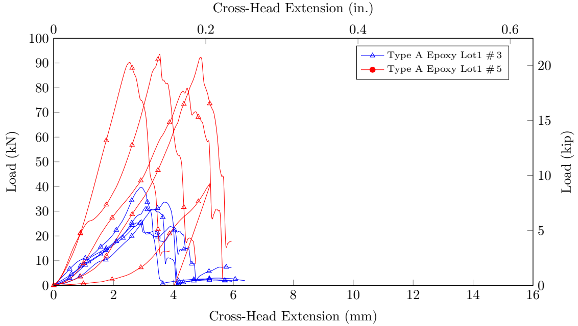
Figure 6.8: Extension-transverse shear load behavior of Type A rebars Lot 1 size 3 and 5
