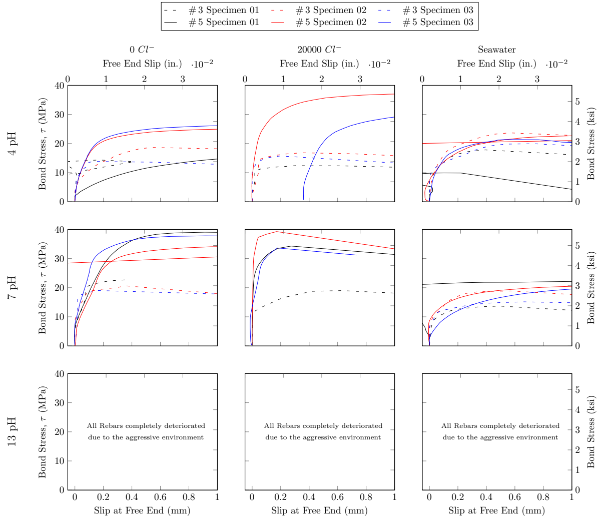
Figure 8.120: Bond stress - slippage behavior of rebar Type B Lot 2 rebars
