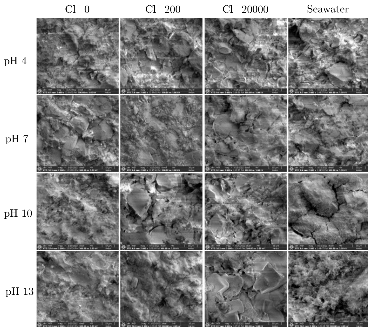
Figure 8.49: Type B Lot 1 rebars at day 600 under 2000x magnification
