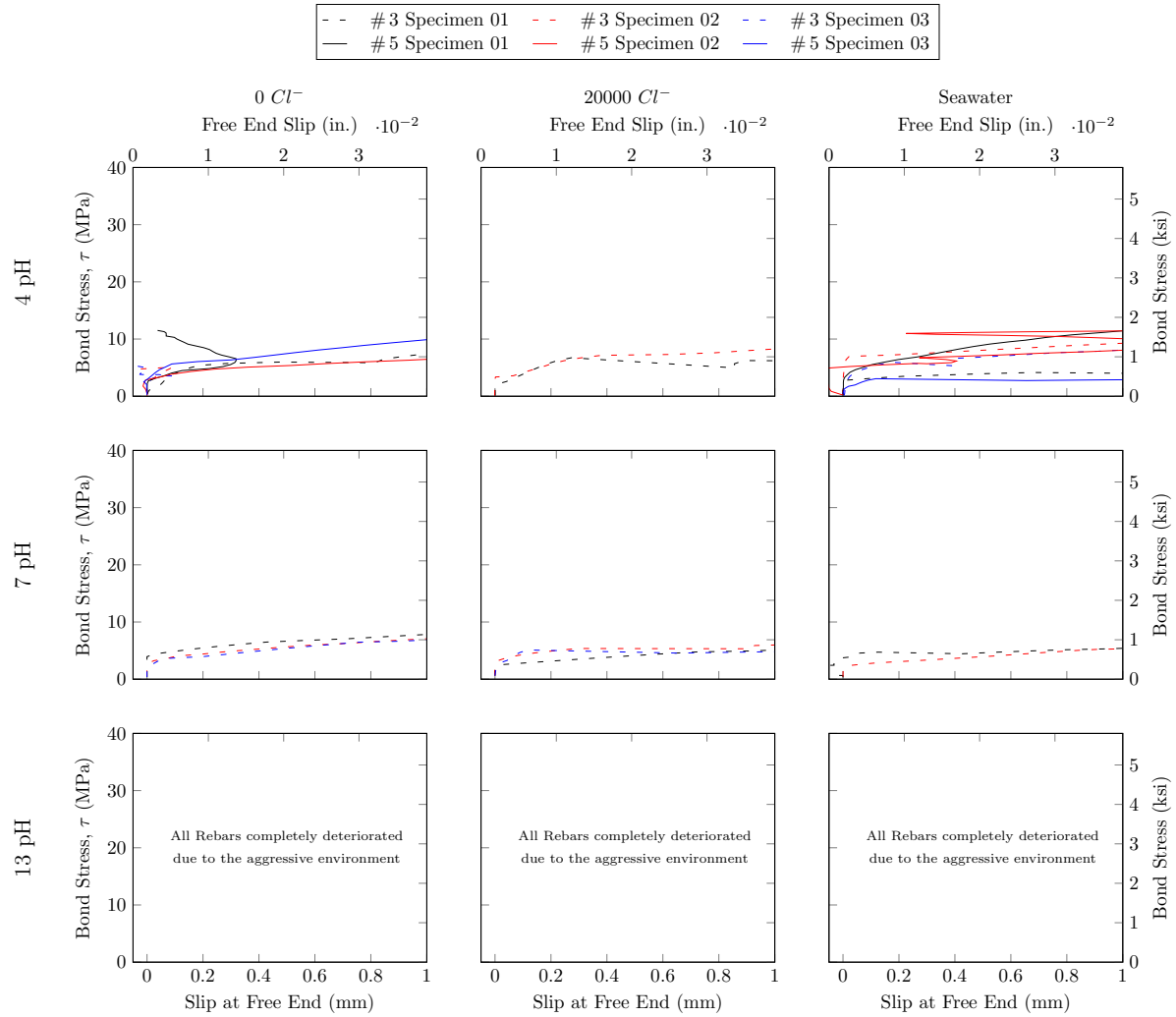
Figure 7.116: Bond stress - slippage behavior of rebar Type C Lot 1 rebars
