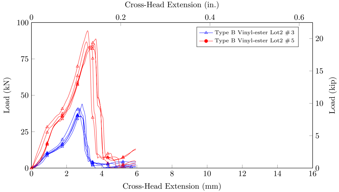
Figure 6.12: Extension-transverse shear load behavior of Type B rebars Lot 2 size 3 and 5
