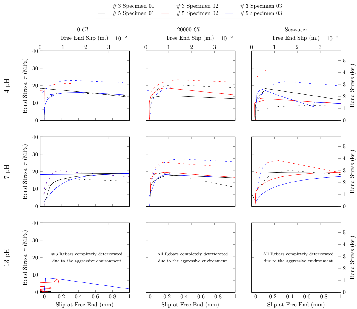
Figure 7.115: Bond stress - slippage behavior of rebar Type B Lot 1 rebar
