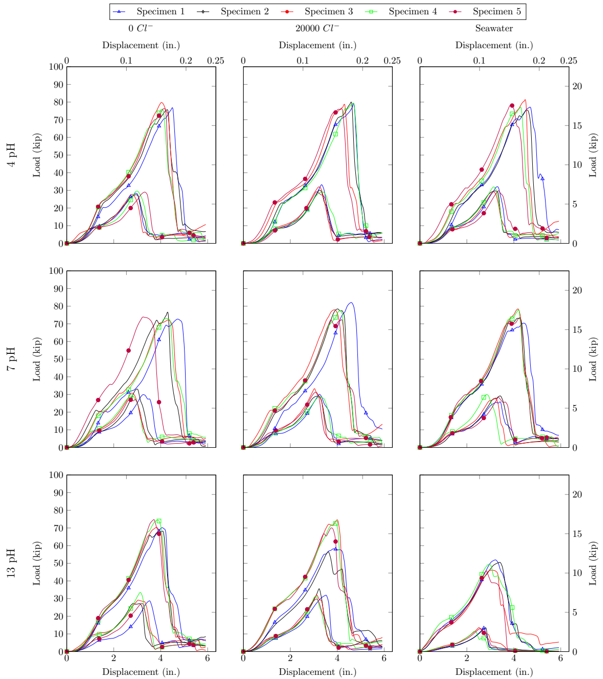
Figure 7.79: 300Day Transverse shear force - displacement behavior of Type B Lot1 tested rebar
