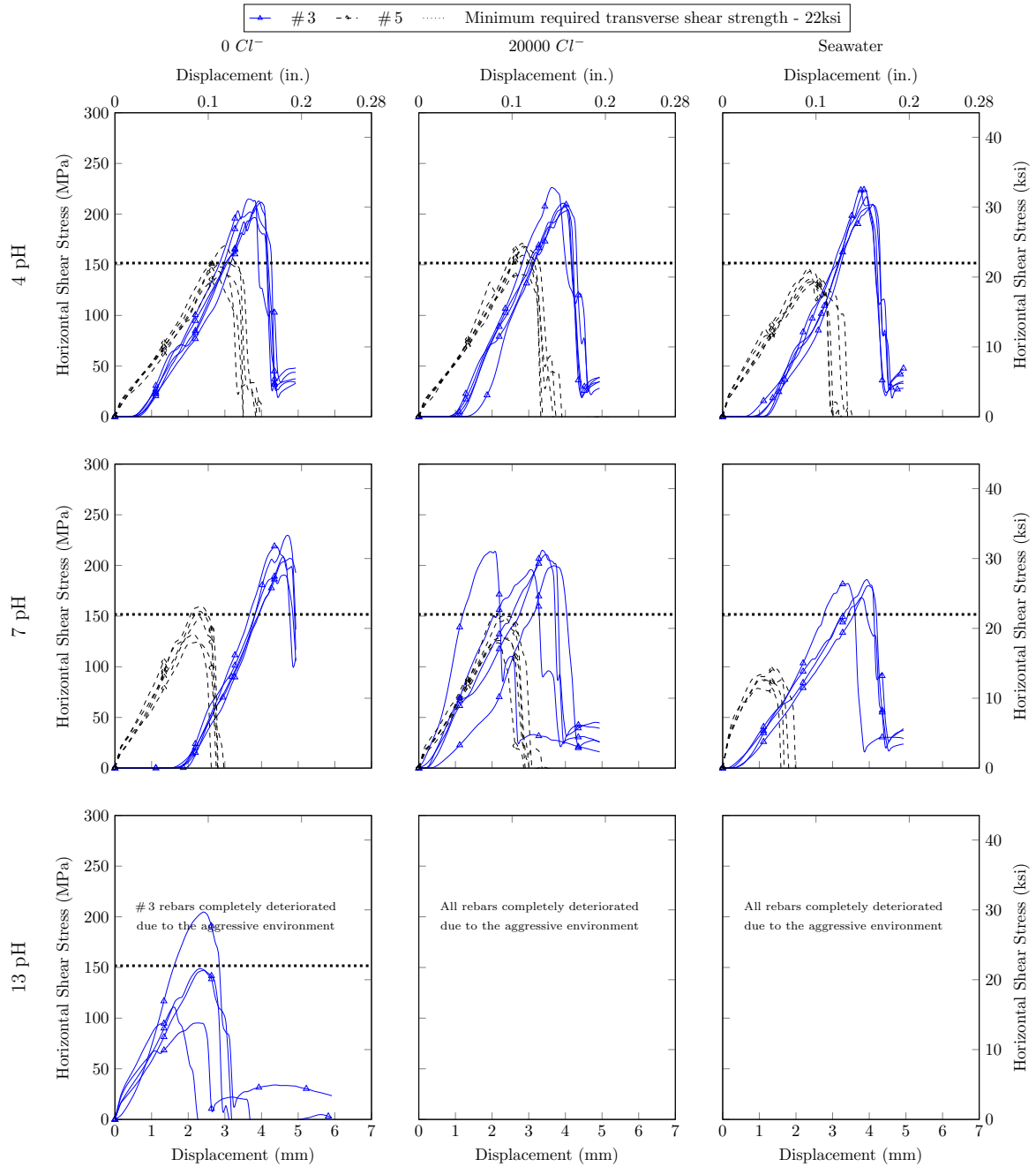
Figure 7.89: 300Day Transverse shear stress - displacement behavior of Type C Lot2 tested rebars
