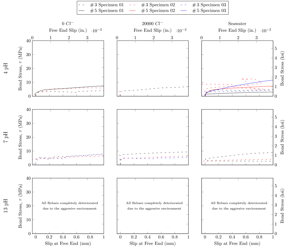
Figure 7.119: Bond stress - slippage behavior of rebar Type C Lot 2 rebars
