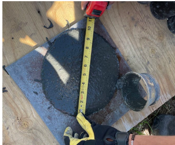
Figure 32: Flow test of MT-UHPC during mockup
