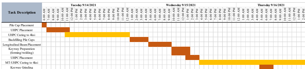
Figure 70: Timeline of UHPC related activities on the second bridge
