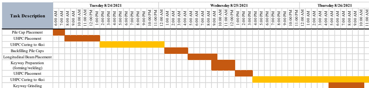
Figure 69: Timeline of UHPC related activities on the first bridge
