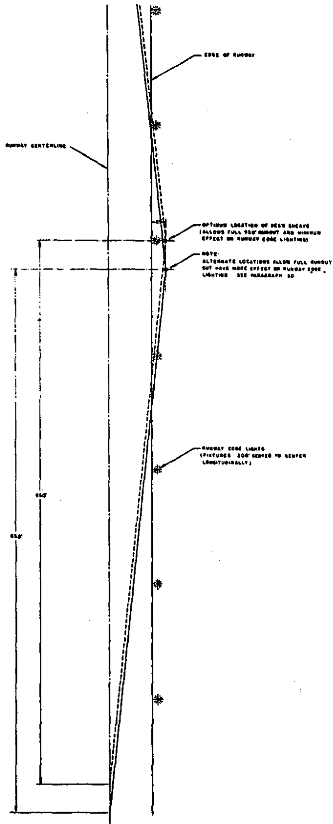
FIGURE 4. PLAN VIEW OF RUNWAY SHOWING OPTIMUM AND A TYPICAL ALTERNATE LOCATION OF DECK SHEAVE WHERE NECESSARY TO INSTALL ACROSS RUNWAY
