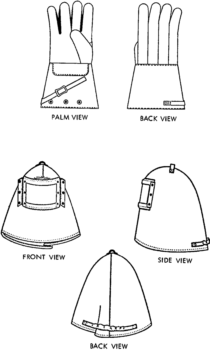
FIGURE 2. Illustration of Aluminized Proximity Gloves and Hood (shoulder length type) indicating suggested designs
