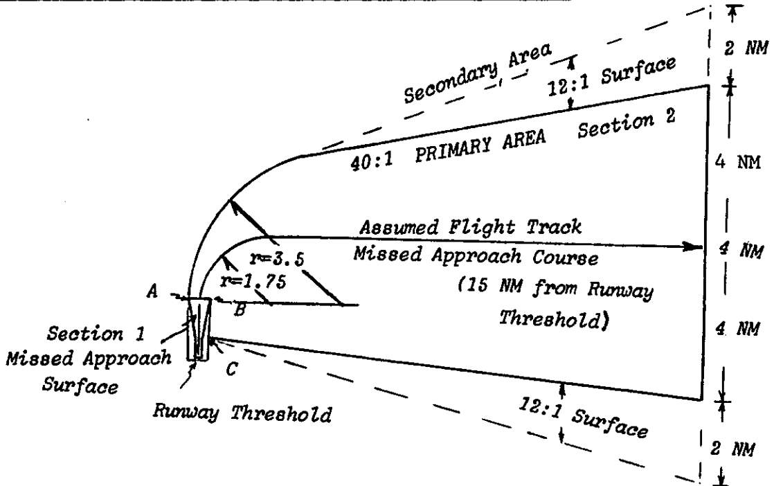
FIGURE 5. TURNING MISSED APPROACH AREA Section 2
