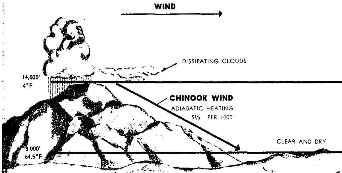
FIGURE 59. Changes in an air mass by passing over a mountainous barrier.
