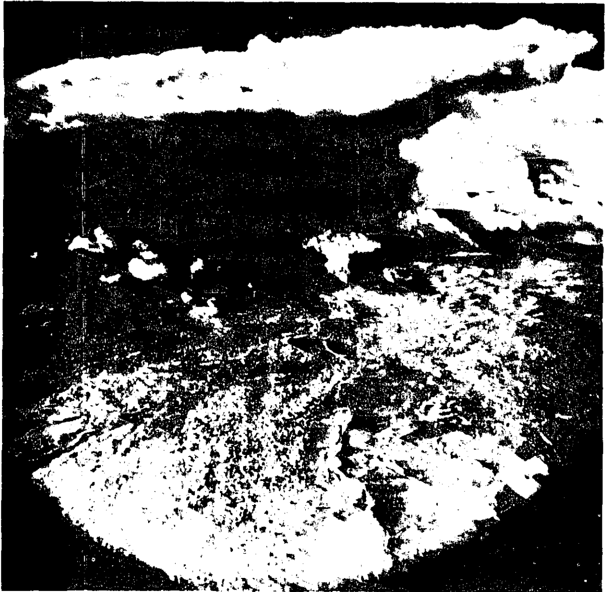
FIGURE 66. An aerial view of a portion of a squall line.
