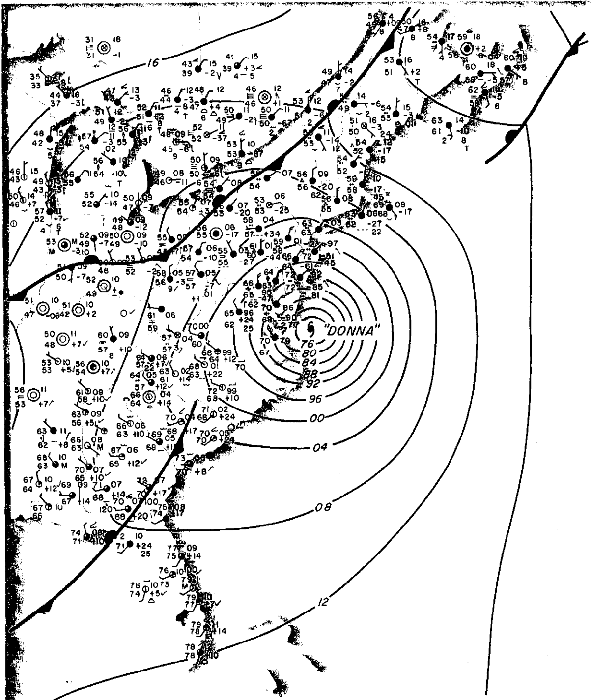
FIGURE 179. Hurricane "Donna" on the surface weather chart, 1200 GMT, September 12, 1960.
