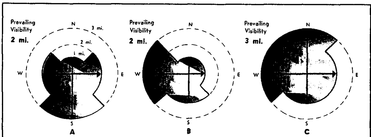
FIGURE 138. Determination of prevailing visibility.
