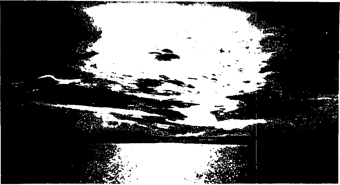
FIGURE 43. Cirrostratus: thin transparent, whitish cloud layer appearing as a sheet or veil; diffuse, or sometimes partly fibrous; generally produces halo phenomena.
