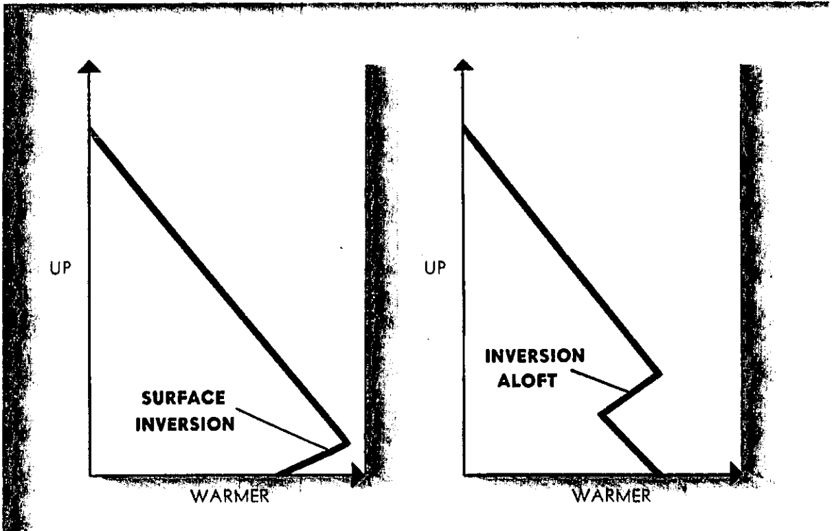
FIGURE 4. Temperature inversions.
