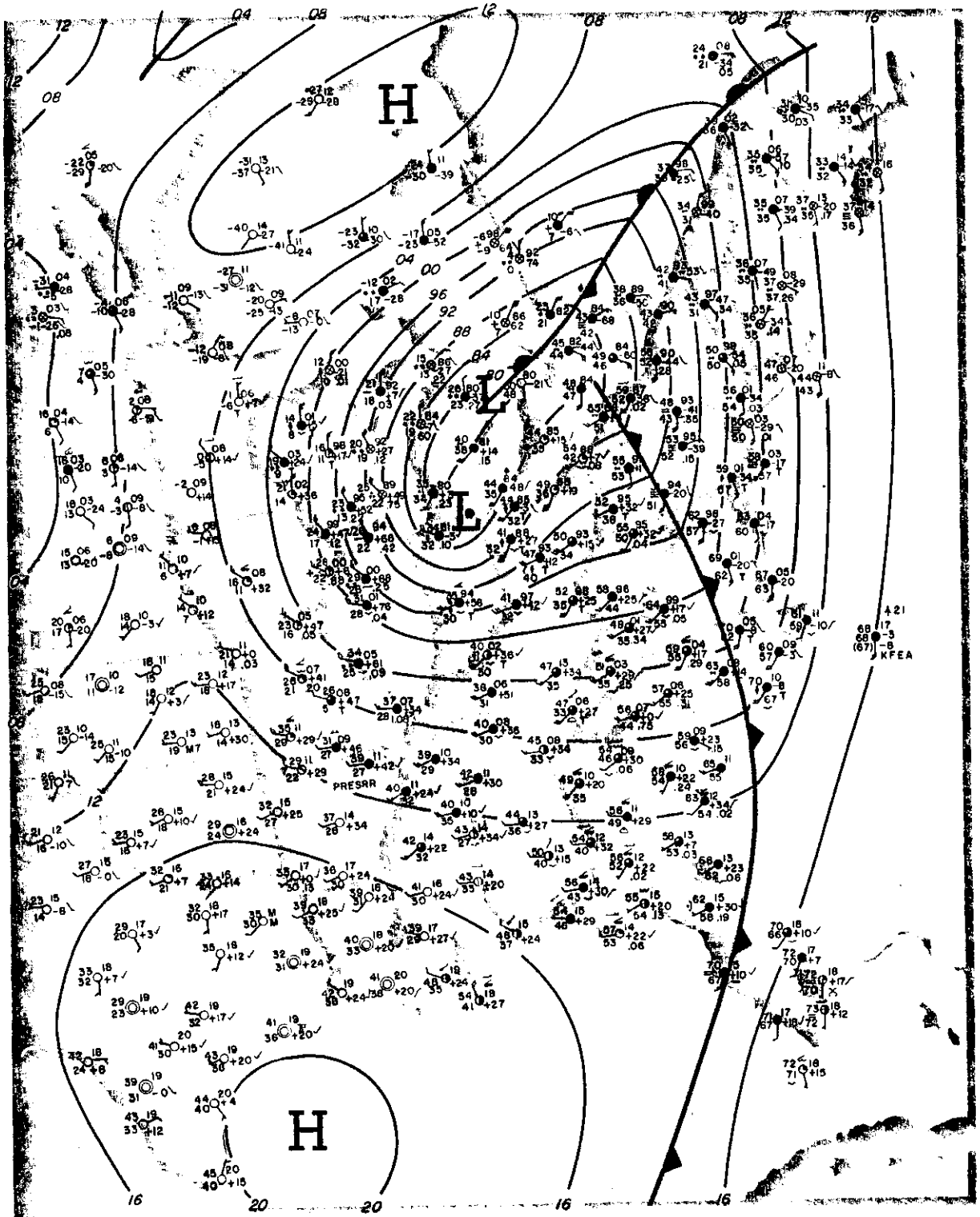
FIGURE 146. Surface weather chart, 1200 GMT, March 5, 1964.
