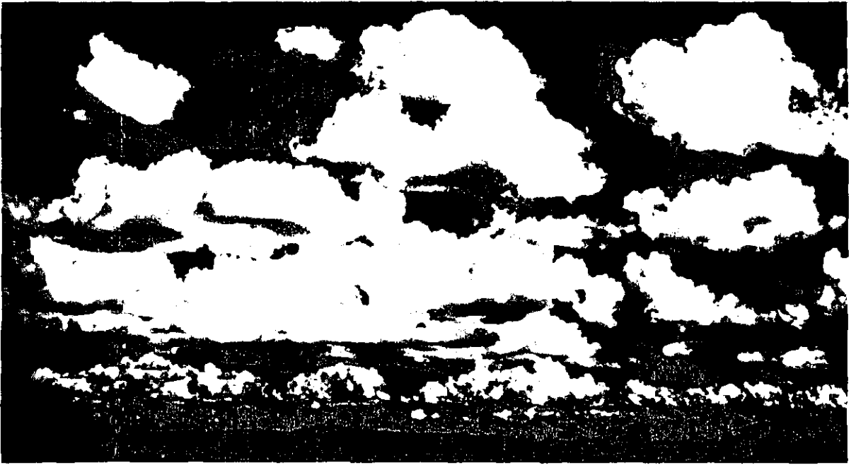
FIGURE 49. Cumulus: detached domes or towers which are usually dense and well defined; develops vertically in the form of rising mounds of which the bulging upper part often resembles a cauliflower; often referred to by pilots as "cu" (pronounced "cue"); composed of a great density of small water droplets, frequently supercooled; larger drops often develop within the cloud and fall from the bases as trails of evaporating rain (virga); ice crystals sometime form in the upper portion and grow larger by taking water from the water droplets; maximum frequency and development in the afternoon over land and during the night over water.
