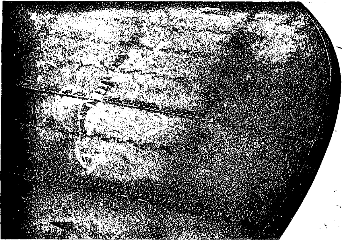
FIGURE 102. Frost.
