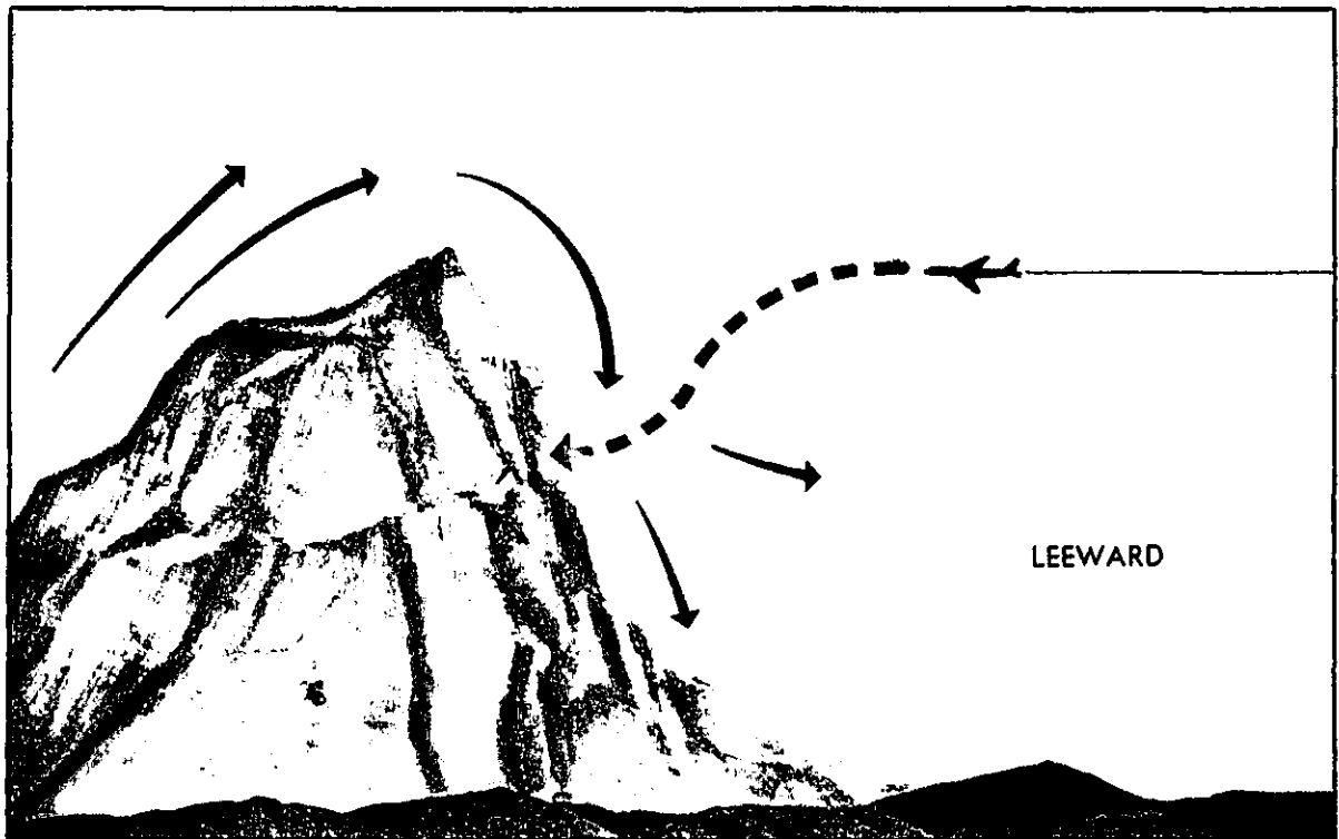
FIGURE 36. Wind flow near mountains.
