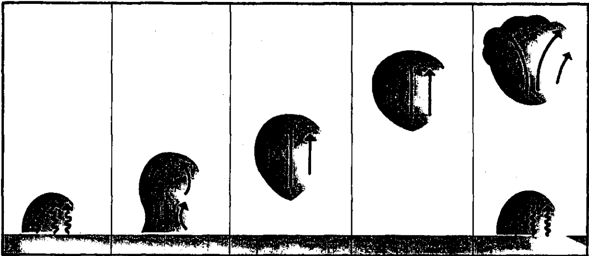
FIGURE 182. Progressive stages of a thermal bubble.
