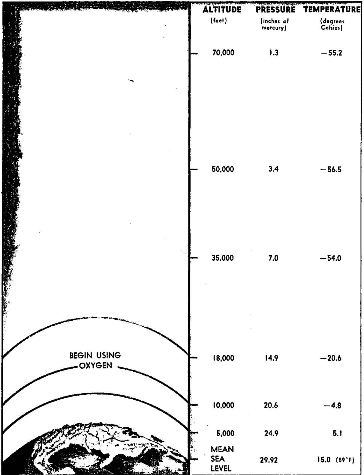
FIGURE 15. The Standard Atmosphere.
