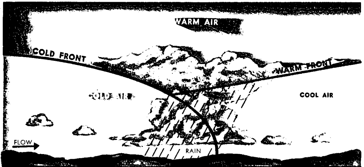
FIGURE 76. A cold-front occlusion in vertical cross section.
