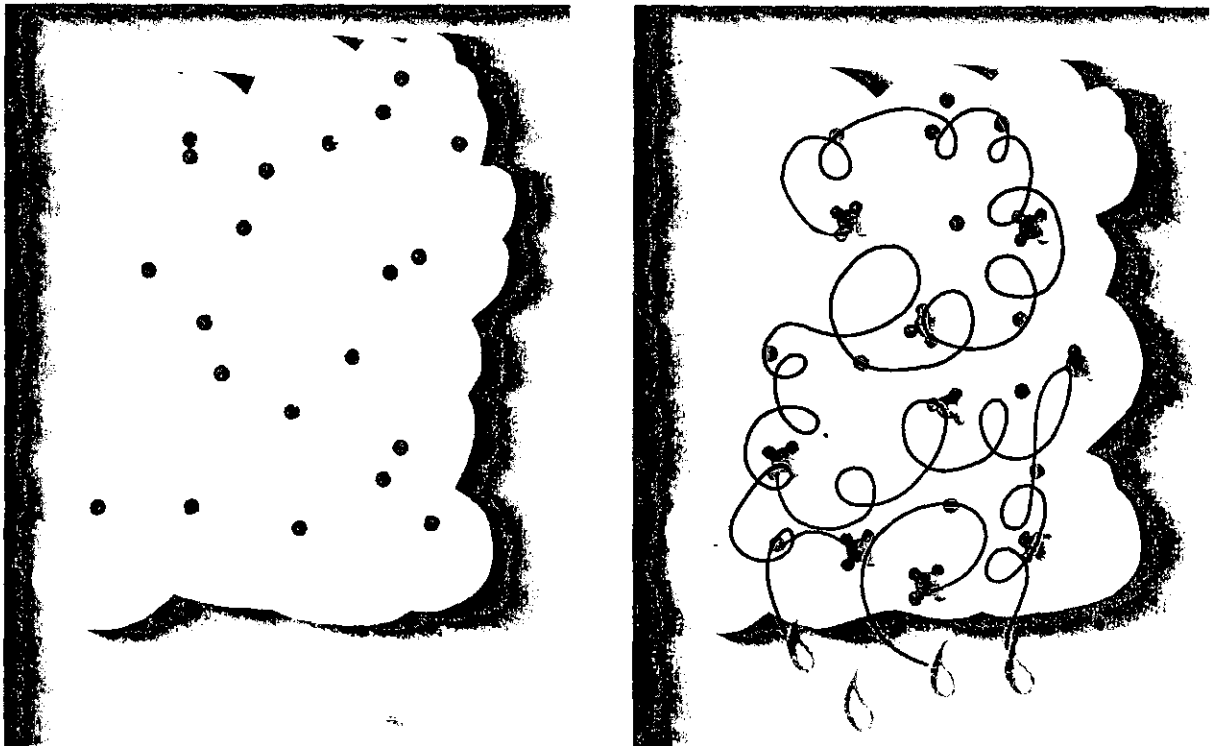
FIGURE 25. Growth of raindrops by collision of cloud droplets.
