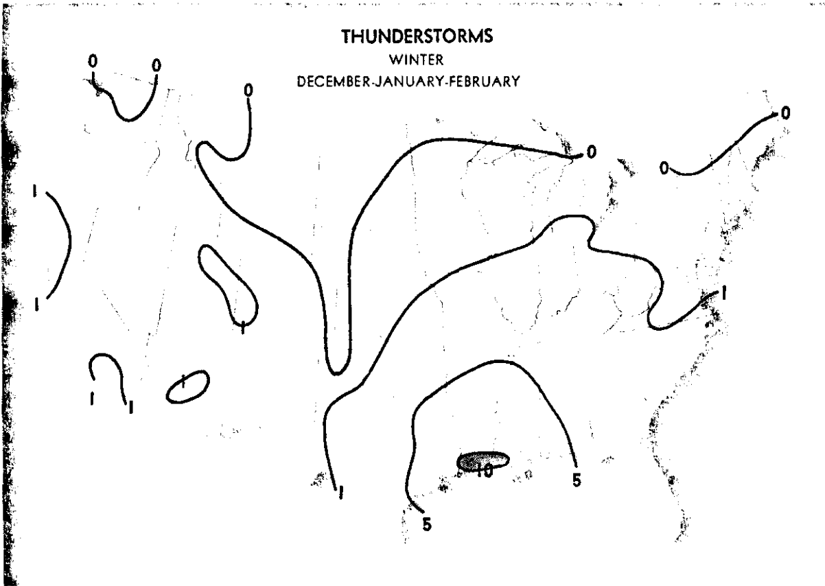
FIGURE 86. The average number of days during winter with thunderstorms.
