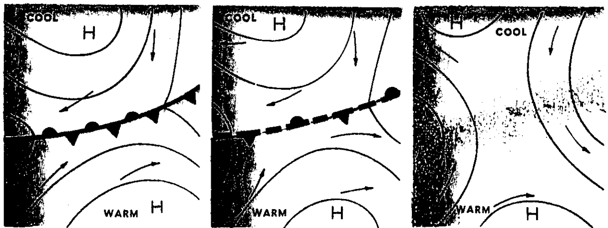
FIGURE 80. Frontolysis.
