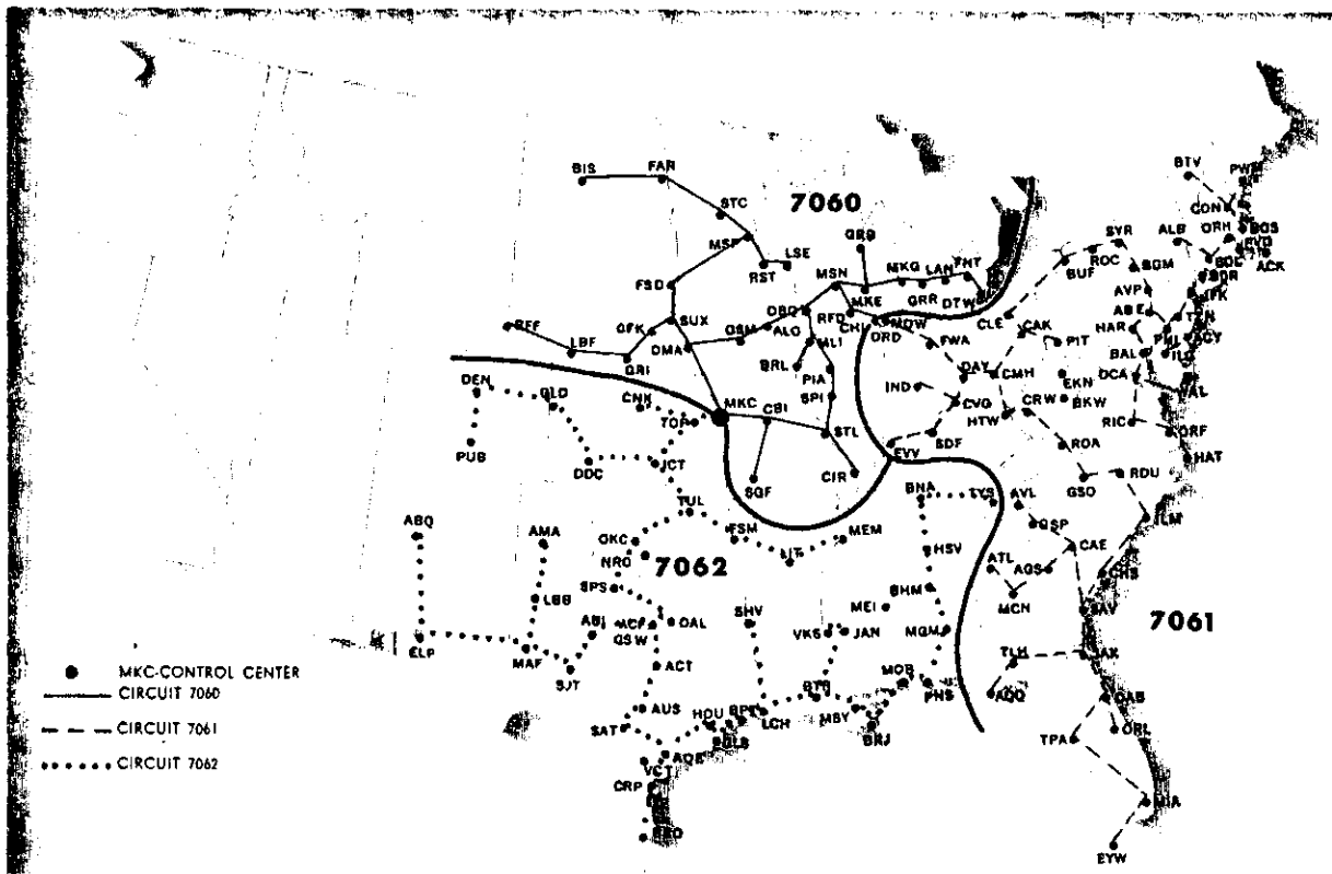
FIGURE 123. Radar warning circuits (RAWARC).
