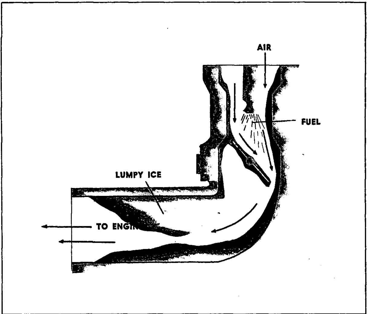
FIGURE 107. Carburetor icing.
