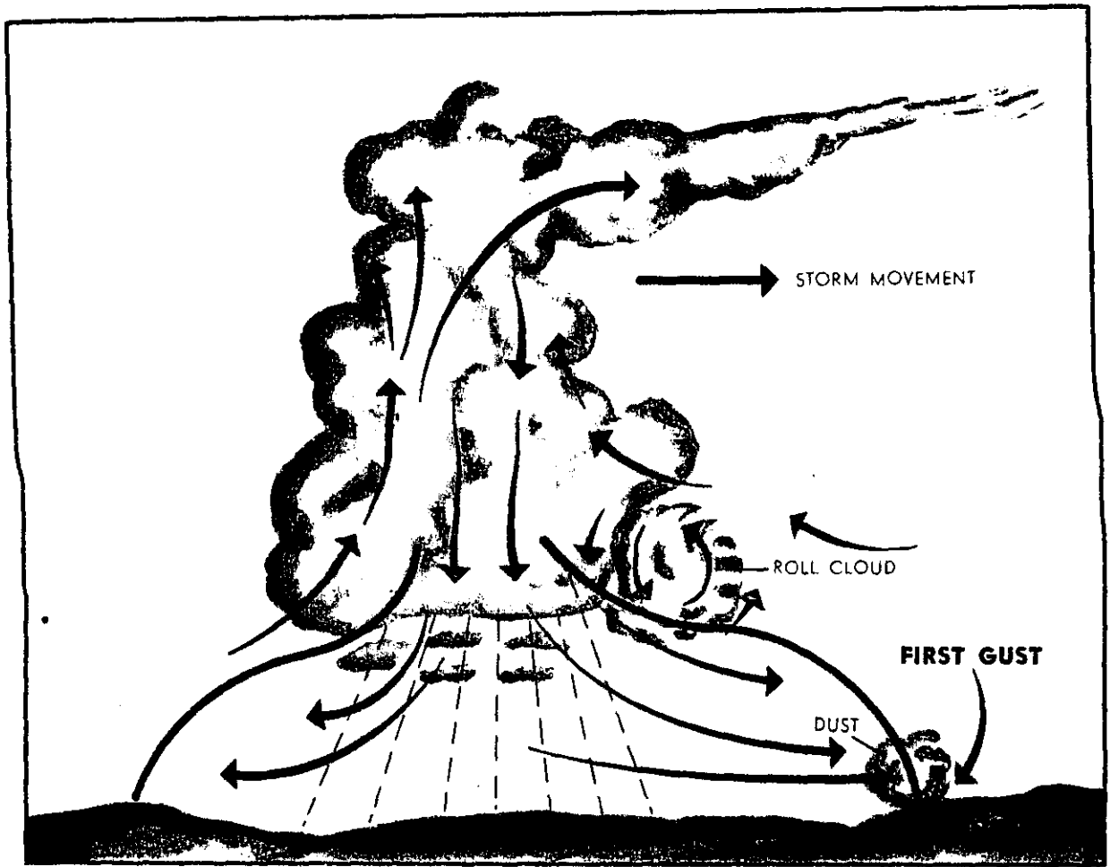
FIGURE 90. Air currents leading to the thunderstorm's first gust.
