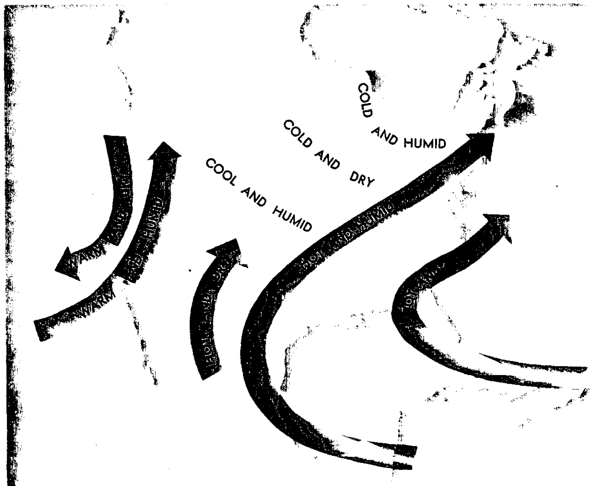
FIGURE 54. Typical paths of air masses. Note the FOHN effect in the western United States.
