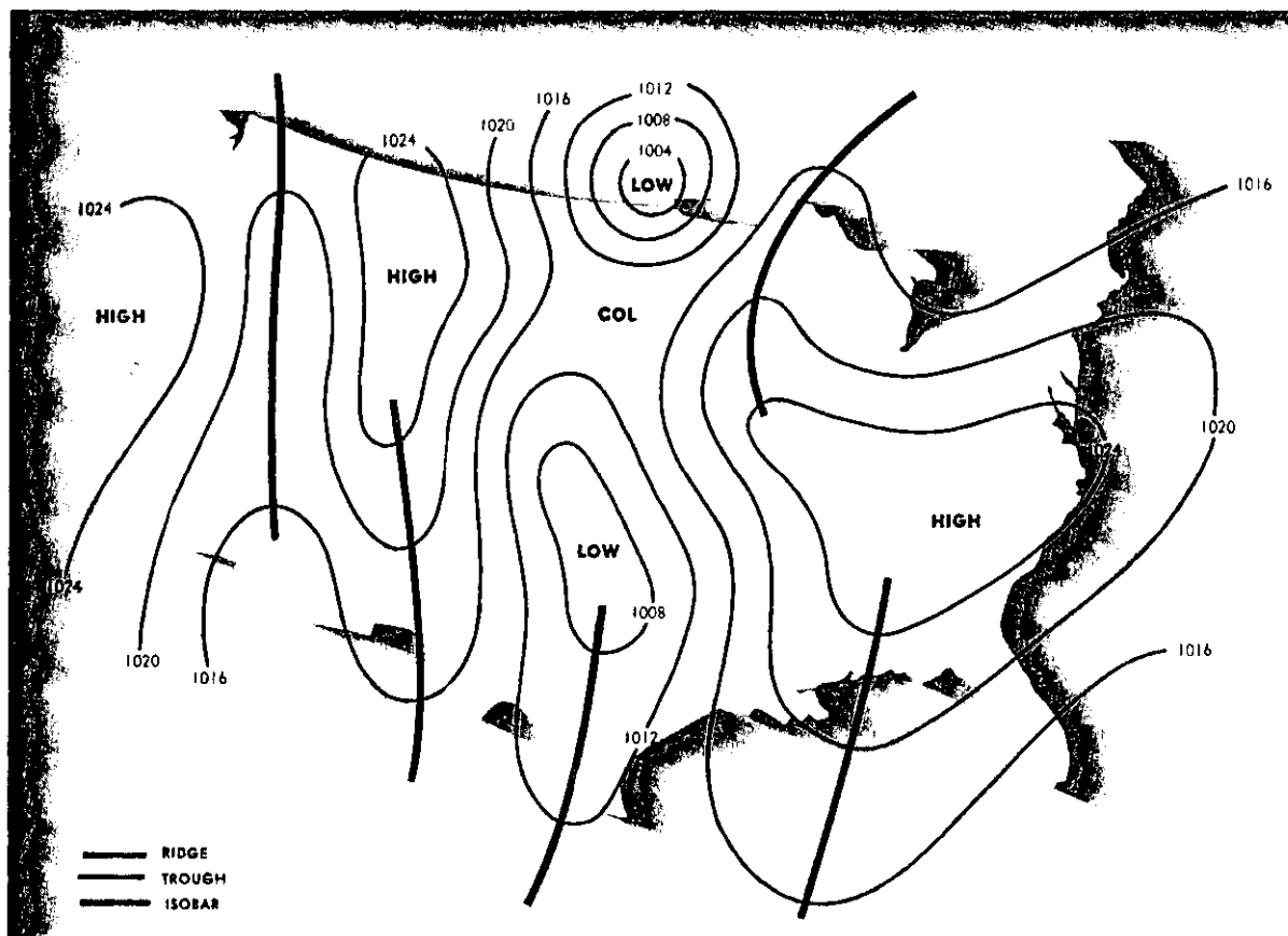
FIGURE 10. Pressure systems.
