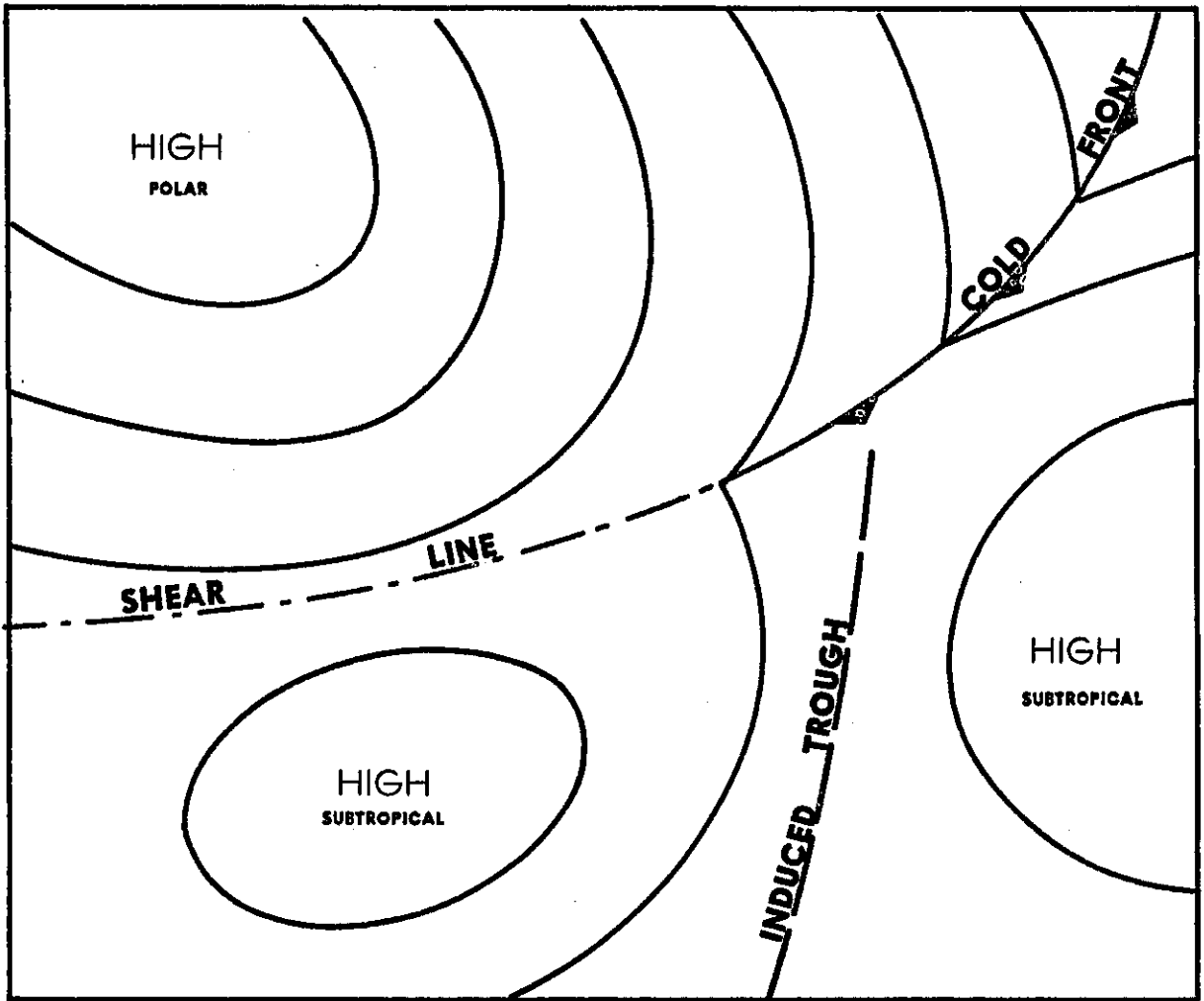
FIGURE 174. A shear line and an induced trough.
