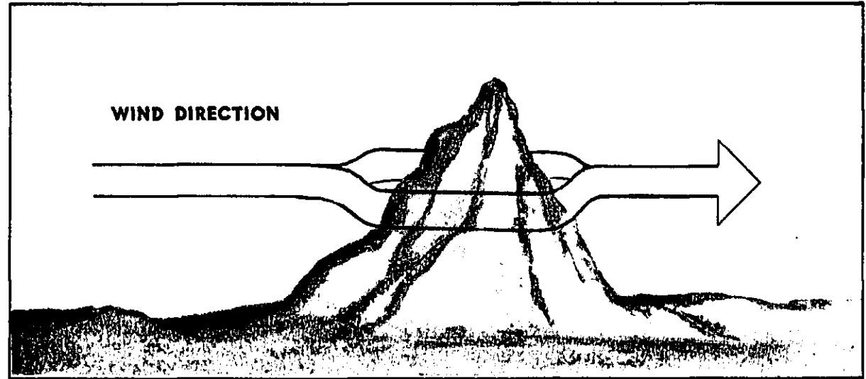
FIGURE 186. Flow of wind around a mountain peak.
