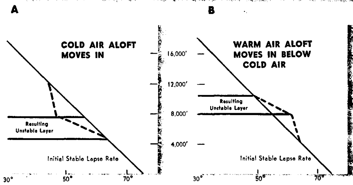
FIGURE 185. Instability aloft.
