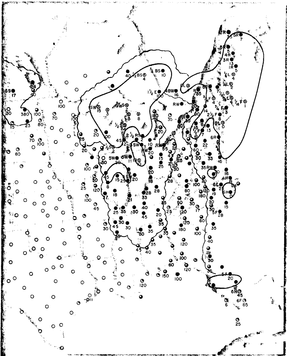
FIGURE 145. Weather depiction chart, 1800 GMT, March 5, 1964.
