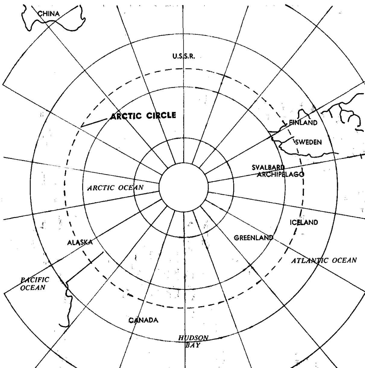
FIGURE 162. The Arctic.
