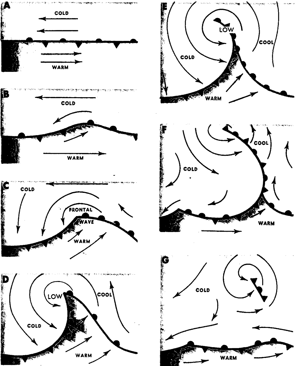
FIGURE 75. The life cycle of a frontal wave.
