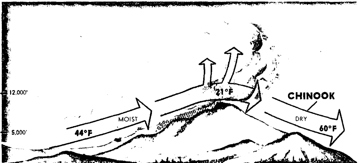
FIGURE 27. Forced air flow over mountains results in the "chinook".
