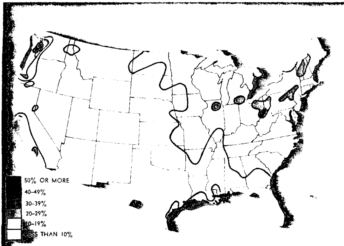
FIGURE 110. Percentage of hours in fall when the ceiling is below 1,000 feet and the visibility is less than 3 miles.
