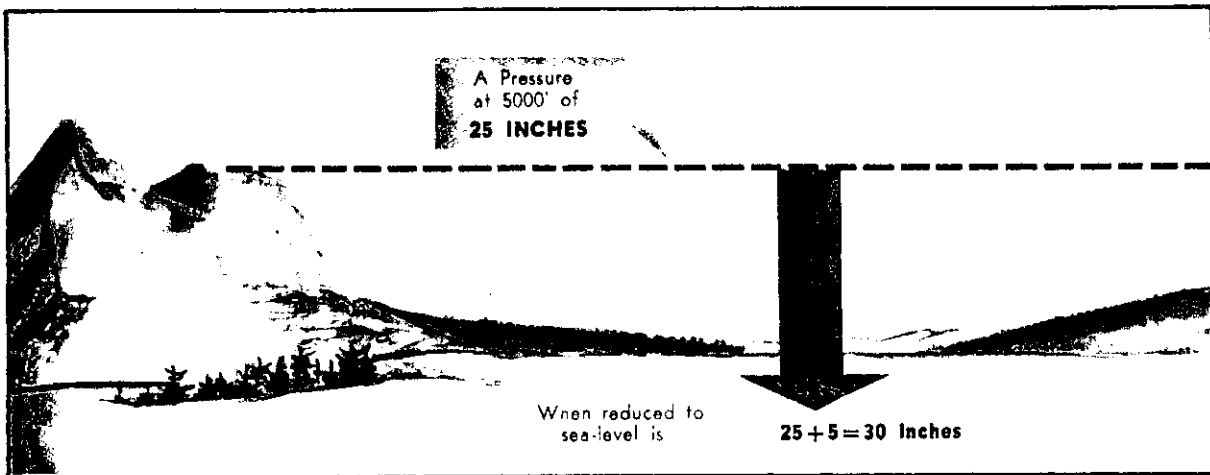
FIGURE 9. Reduction of station pressure to sea level.
