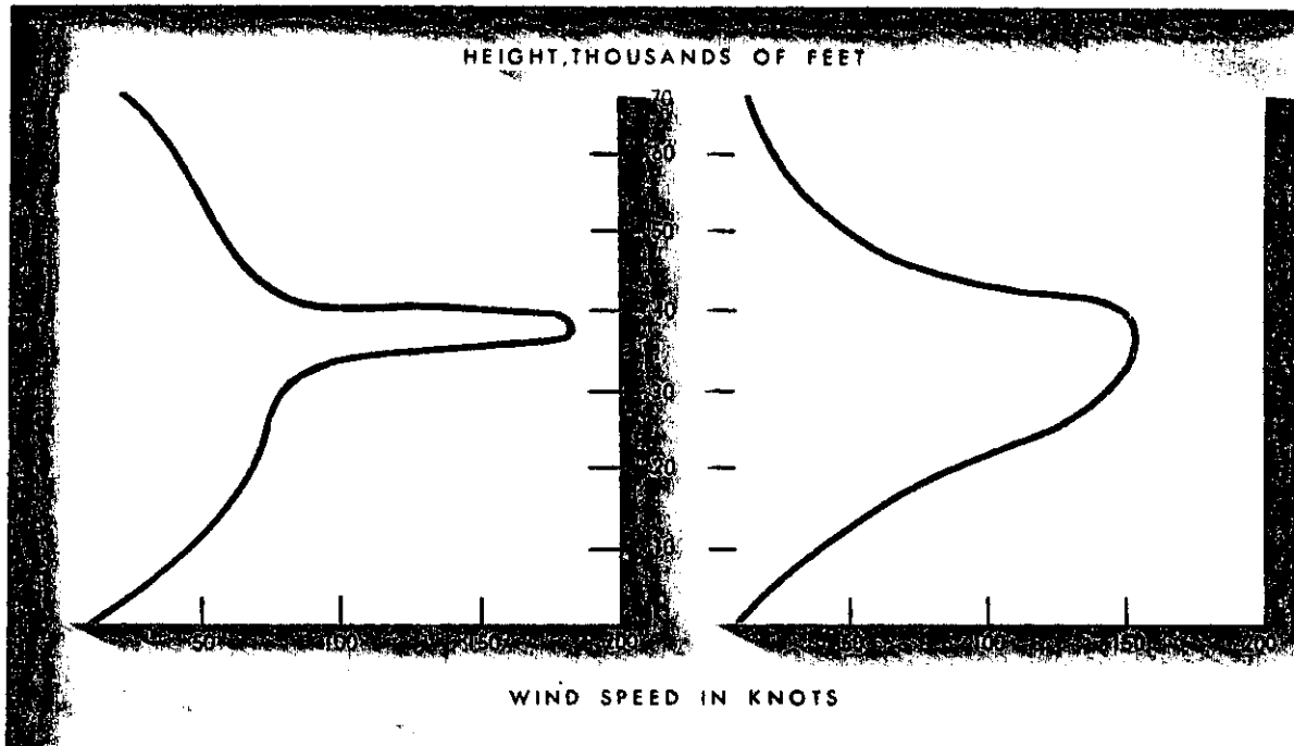
FIGURE 160. Vertical profiles of wind speeds.
