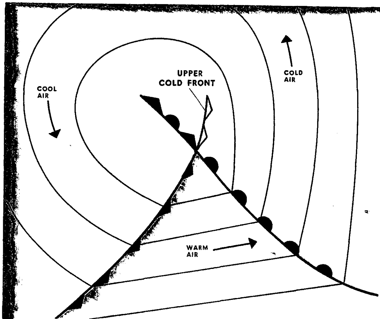
FIGURE 77. The structure of a warm-frontal occlusion on the surface weather chart.
