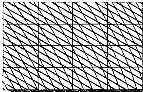
FIGURE 29. The adiabatic chart.
