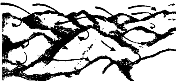
FIGURE 187. Flow of wind over various types of terrain.
