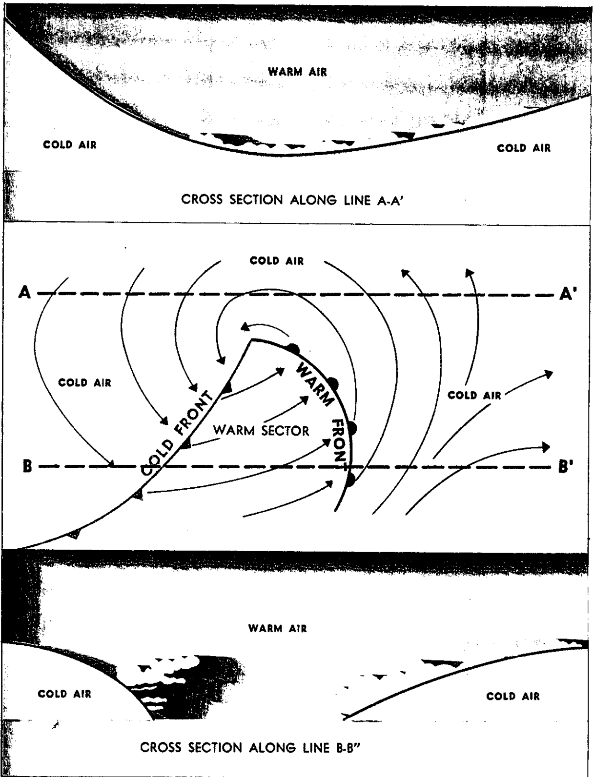
FIGURE 74. A frontal wave on a surface weather chart, with cross sections along two lines.
