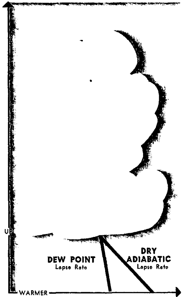
FIGURE 28. Cloud base determination.
