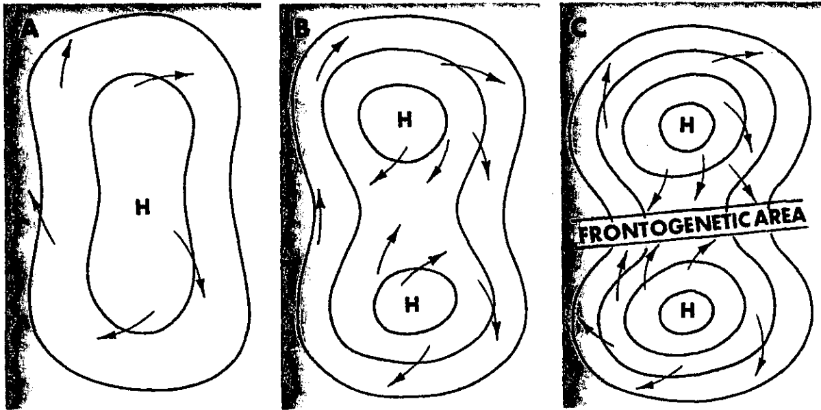
FIGURE 81. Frontogenesis.
