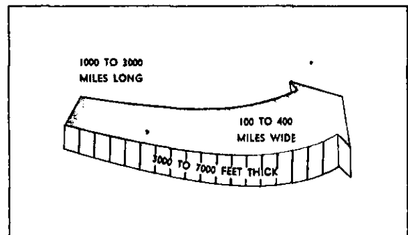
FIGURE 157. Size of a jet stream segment.
