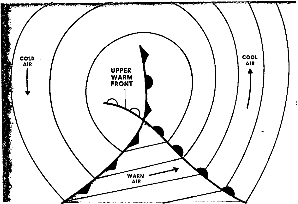
FIGURE 75. The structure of an occluded frontal wave on a surface weather chart.
