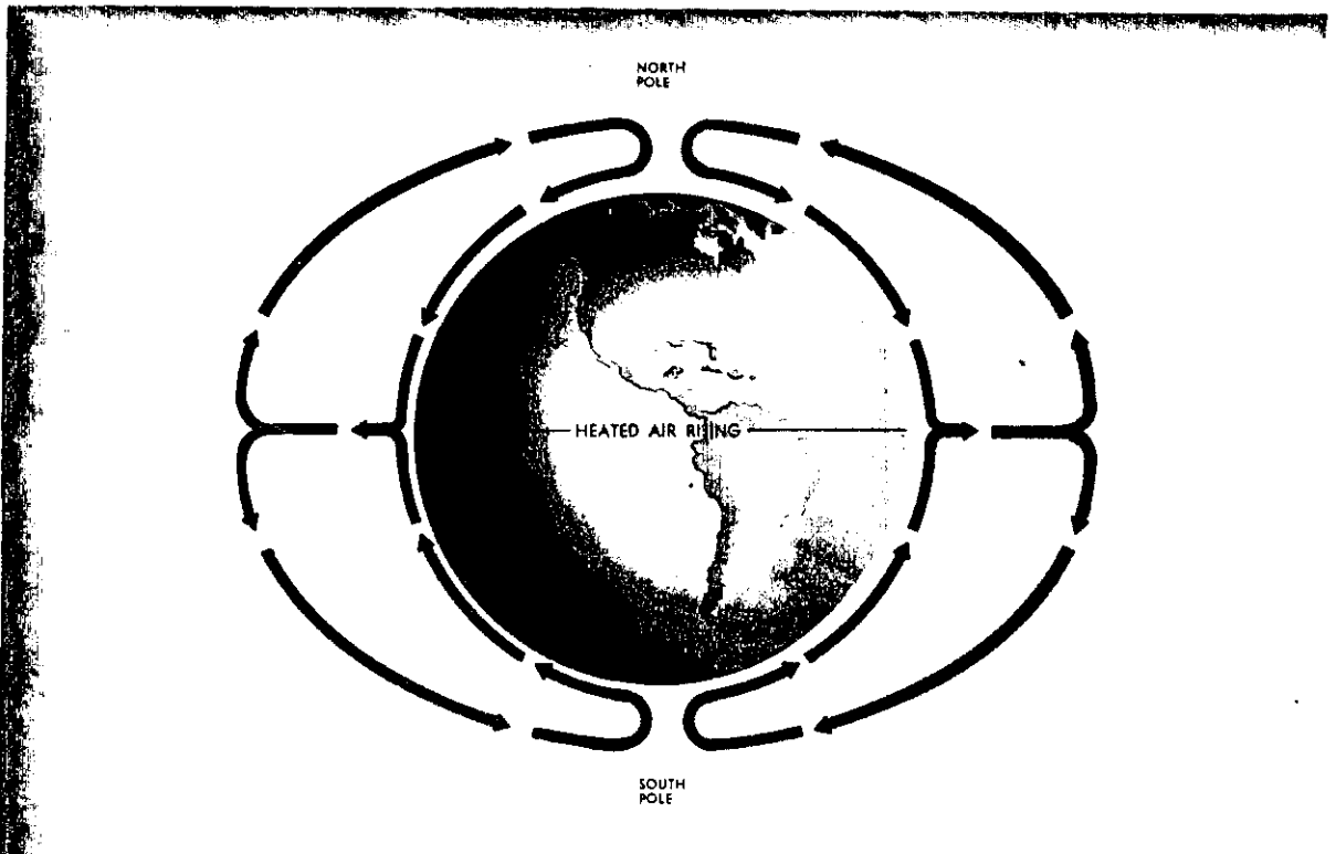
FIGURE 16. Theoretical air movement if the earth did not rotate.
