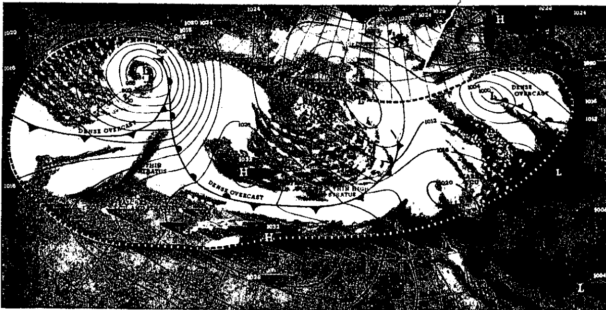
Storm family over the North Pacific Ocean with TIROS cloud pictures superimposed on a conventional surface weather chart, May 20, 1960 (prepared by V. J. Oliver, U.S. Weather Bureau).
