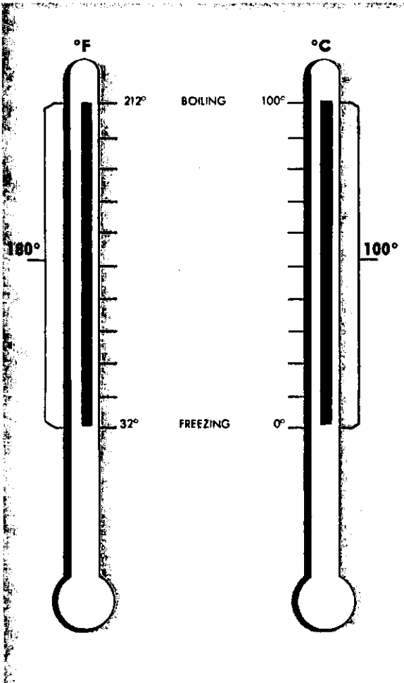
FIGURE 3. Temperature scales.
