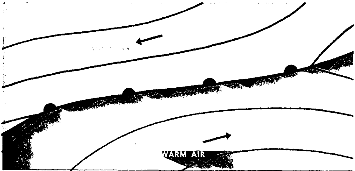
FIGURE 72. A stationary front on a surface weather chart.
