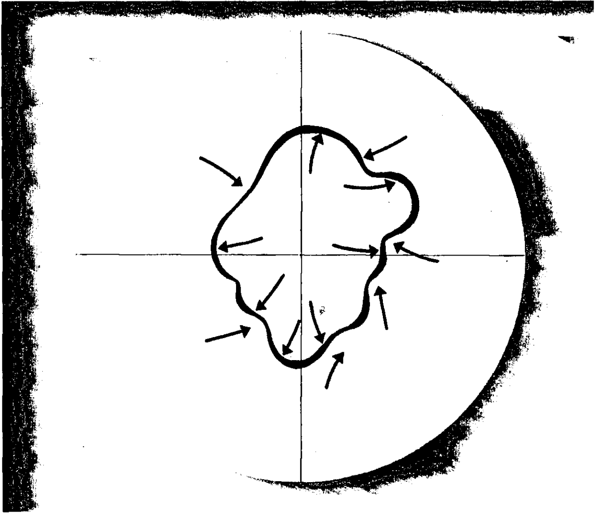
FIGURE 62. Hemispheric view of the polar front.
