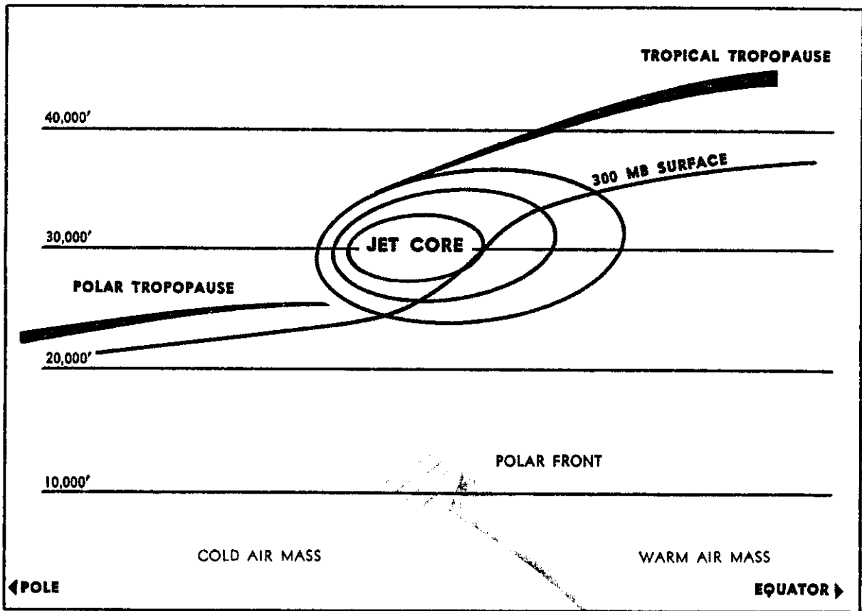
FIGURE 158. Jet winds as related to the polar and tropical tropopauses.
