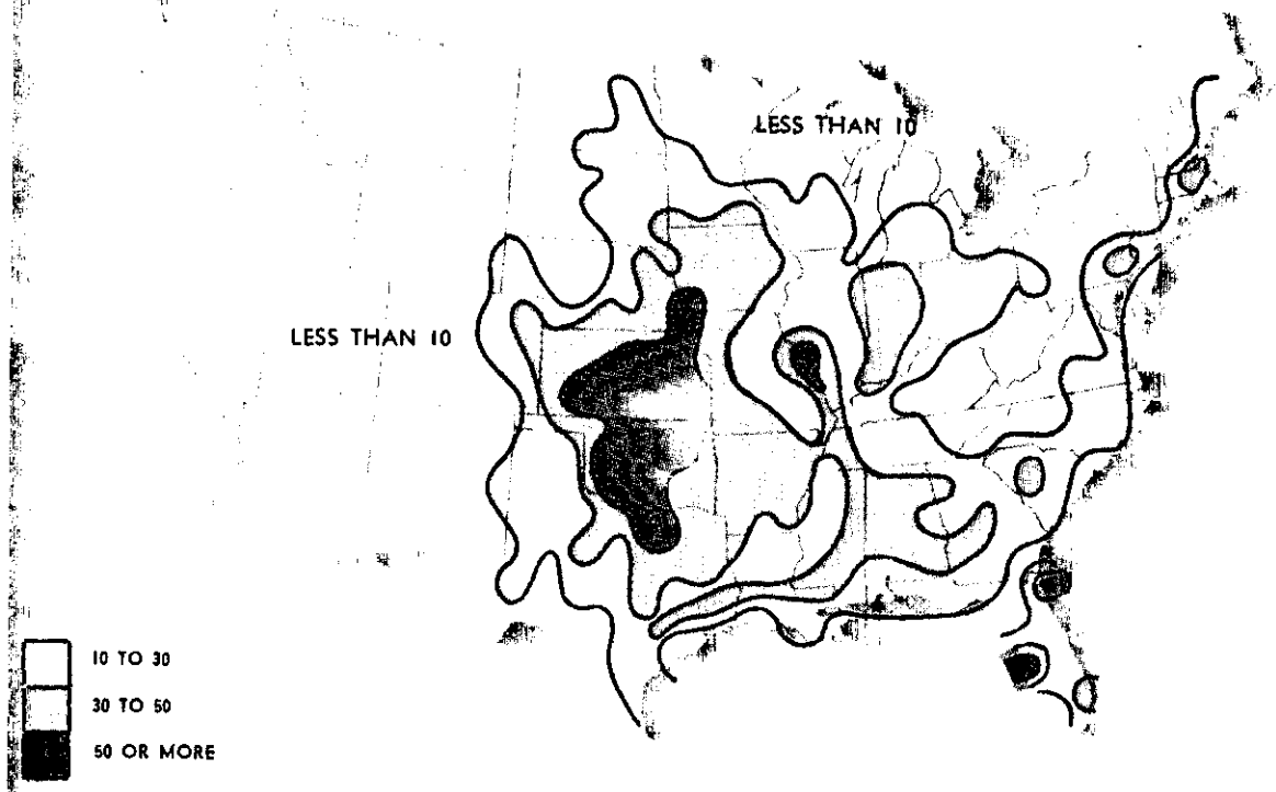
FIGURE 97. Tornado frequency, 1916-63.
