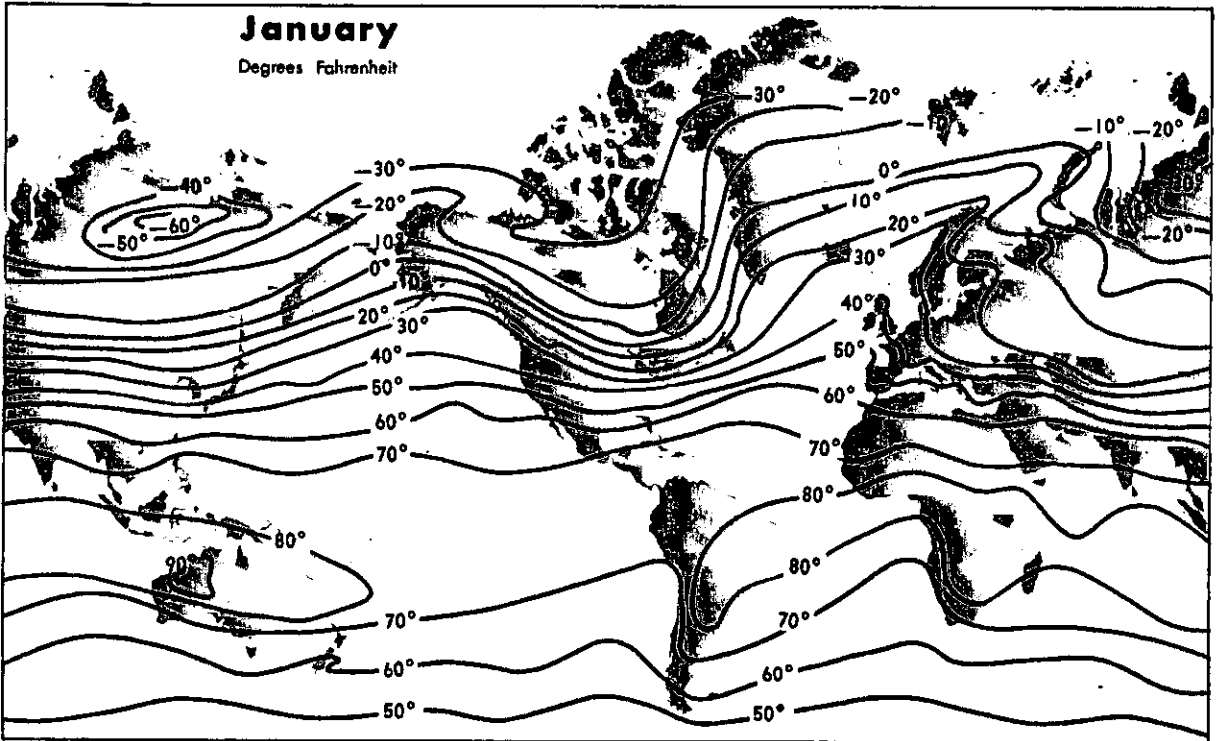
FIGURE 5. World Temperatures (mean).
