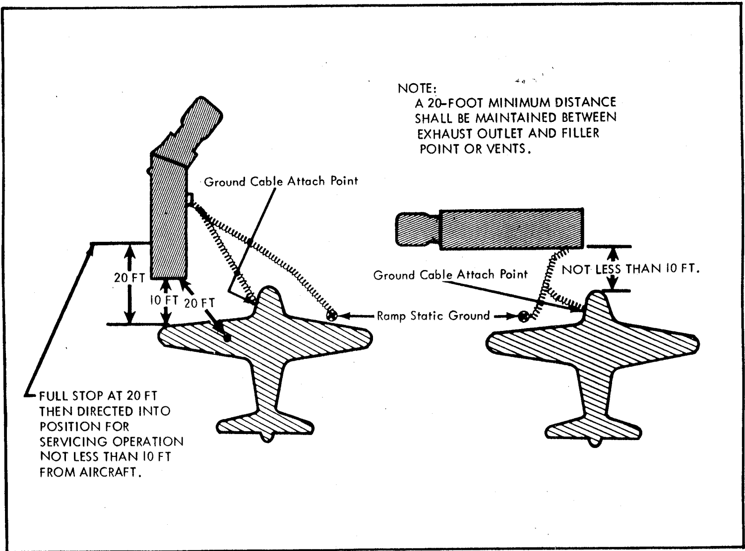
FIGURE 3 POSITIONING FUEL TRUCK
