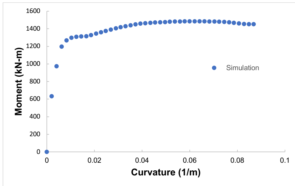
Figure 10. Moment-Curvature Analysis for the RC Critical Cross Section about the Strong Axis (Local Z-Axis) with an Axial Compressive Load of P = -680 Kn
