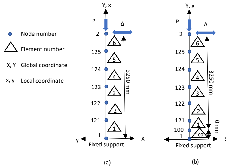
Figure 6. Nonlinear Static Cyclic Pushover Analysis of (a) Model 1 (Excluding Bond-Slip) and (b) Model 2 (Including Bond-Slip)
