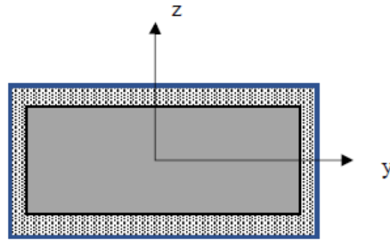
Full spalling
