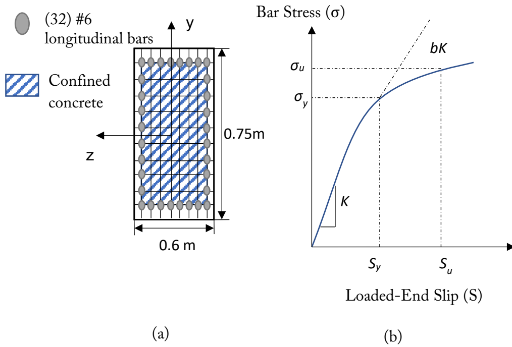
Figure 3. (a) Fiber Element Discretization of the Cross Section of the RC Bridge Column; (b) Envelope Curve of the Bars Stress Vs. Loaded-End Slip Relationship as Modeled in Bond_Sp01 [28]
