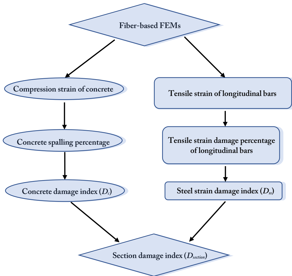
Figure 4. Section Damage Indices [17]
