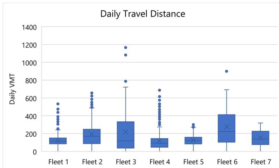
Figure 2. Distribution of daily travel distance per vehicle.
