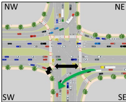
B) Schematic of Offset Crossing - crosswalks are "offset" toward the inside of the intersection (black) and do not conflict with the parallel left turns (green)
