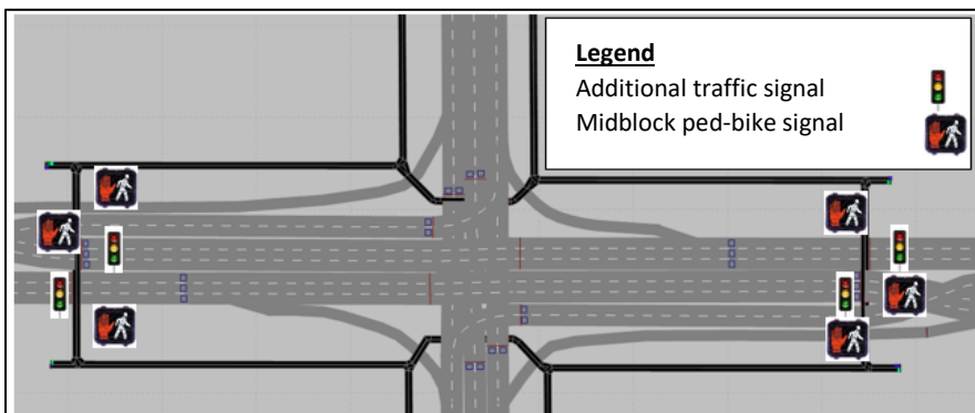
C) Schematic of a Midblock Crossing - pedestrians have a very short travel path between the left corners of the NW and SW quadrant and between the right corners of NE and SE quadrant. However, some other routes experience significant out of direction travel.
