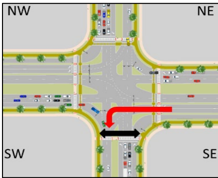
A) Schematic of Traditional Crossing - vehicular left-turn movement from one approach (red) conflicts with the parallel pedestrian-bicycle crossing (black)
