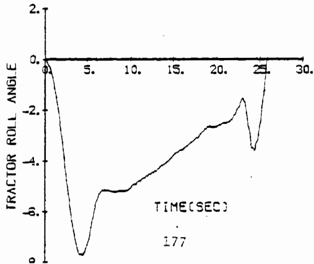
Figure 42. Site 7, hi-c.g., 35 mi/h.
