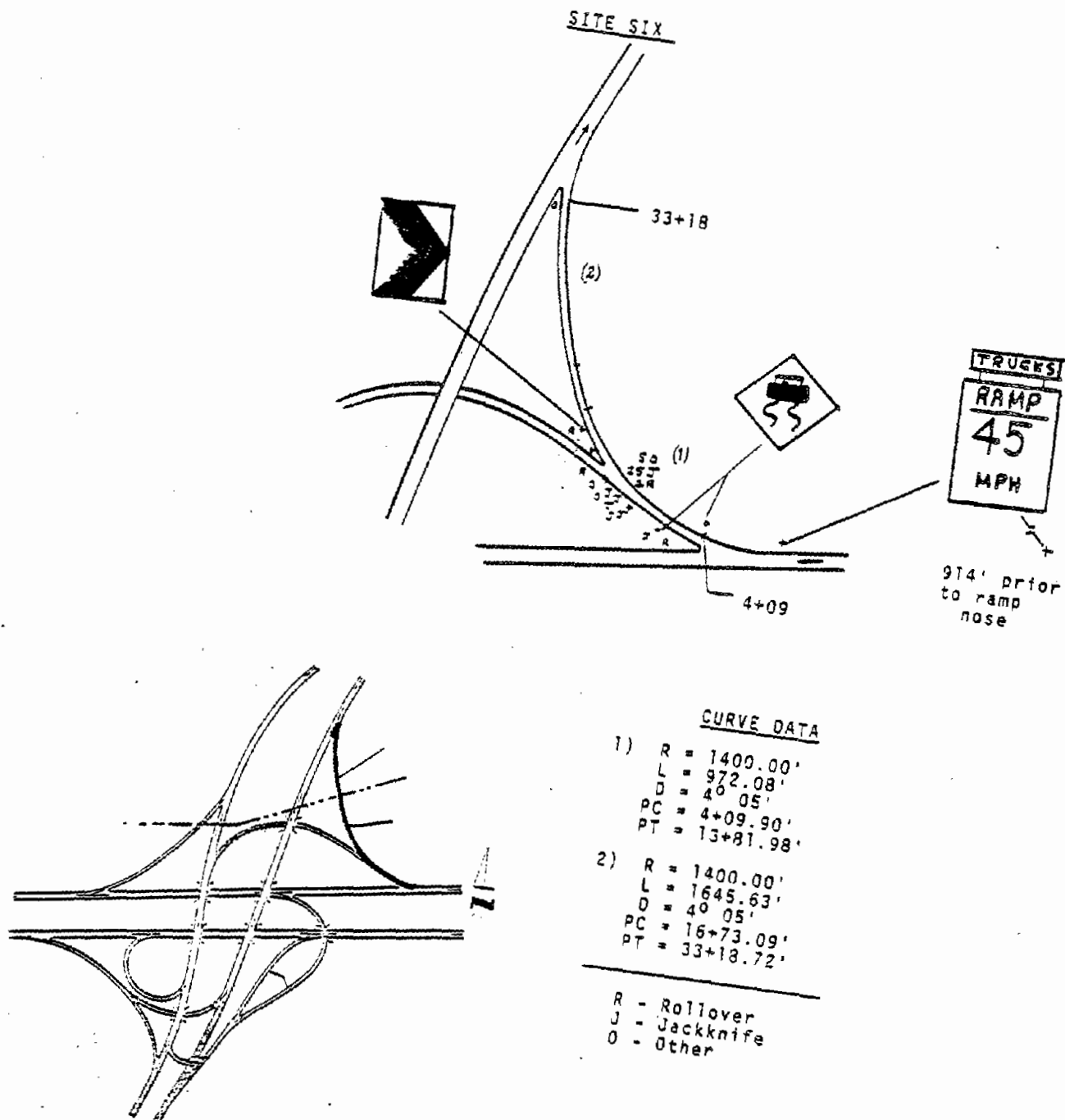
Figure 5. Layout of site 6.
