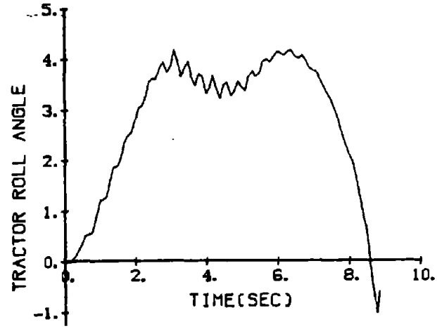
Figure 29. Site 4 - empty vehicle M = 0.50 , 55 mi/h, 20 PSI.
