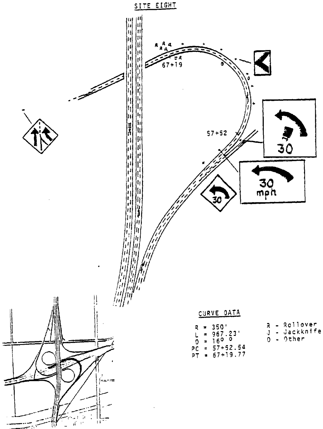
Figure 7. Layout of site 8.
