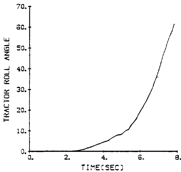
Figure 51. Site 12, hi-c.g 45 mi/h.
