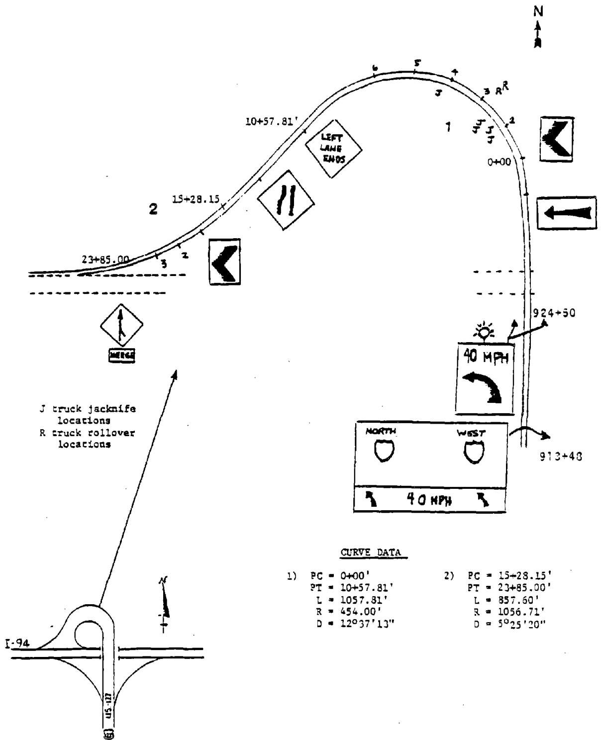
Figure 10. Layout of site 12.
