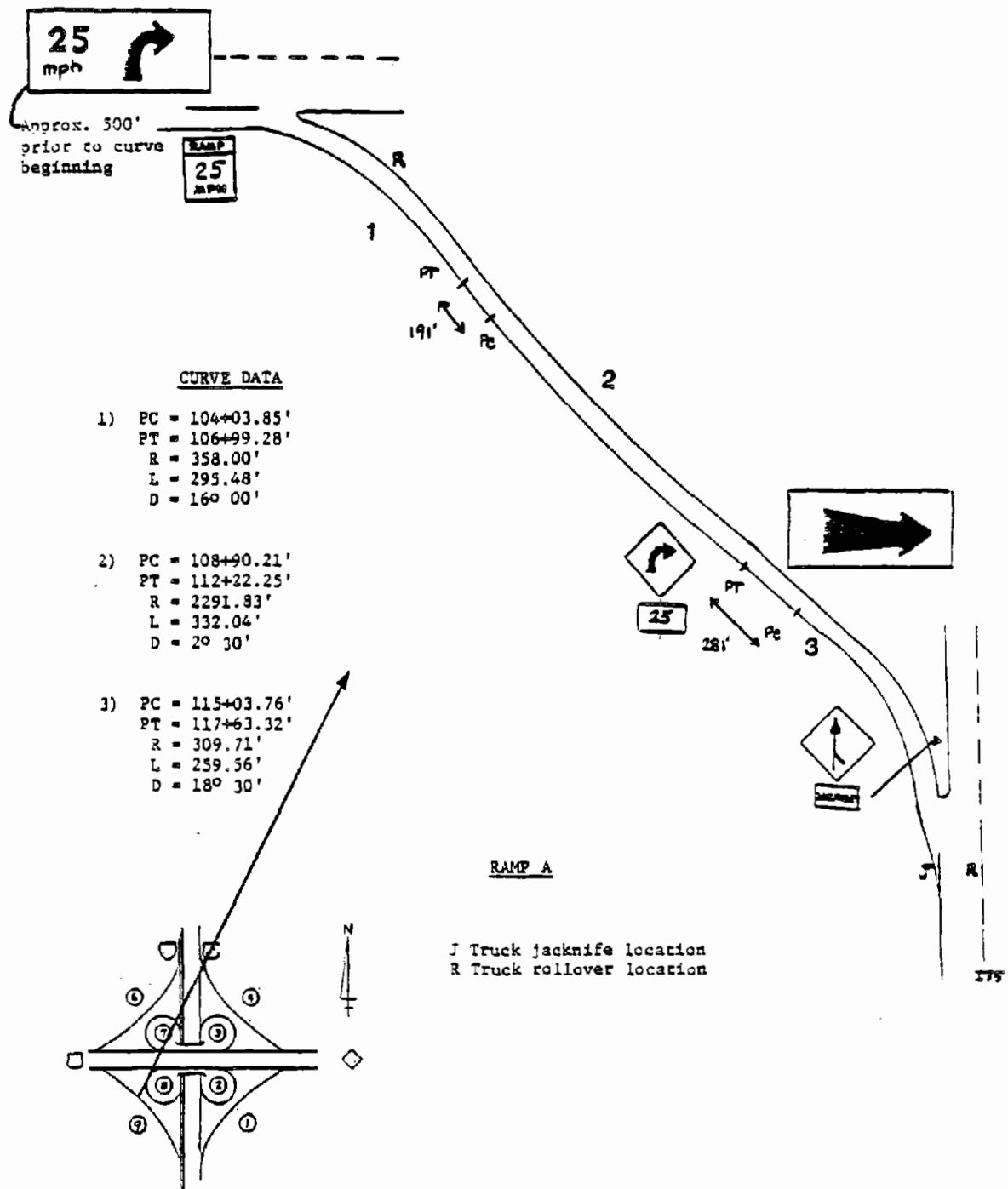
Figure 9. Layout of sites 10 and 11.
