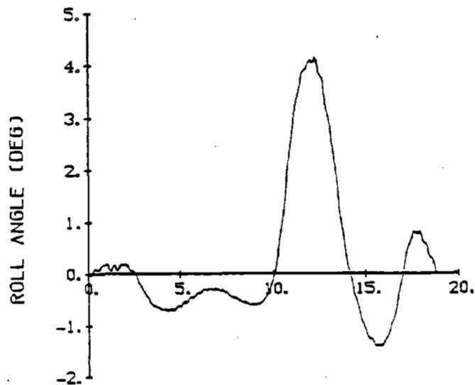
Figure 37. Site 6 base- line, 70 mi/h
