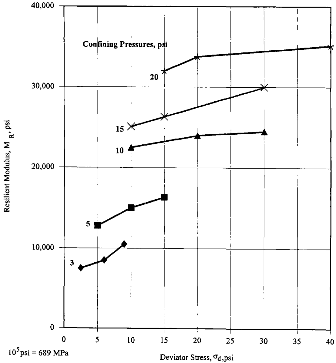
Figure 3. Example of repeated load triaxial resilient modulus test results of a granular base material.
