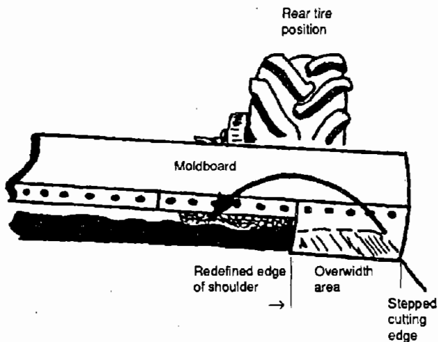
Recover Material from Overwidth Areas
