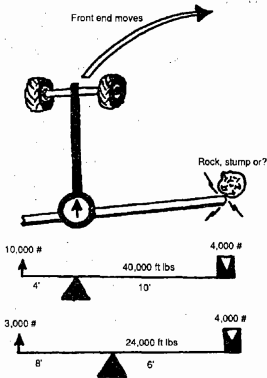
Sidsift Increases Forces on Graders
