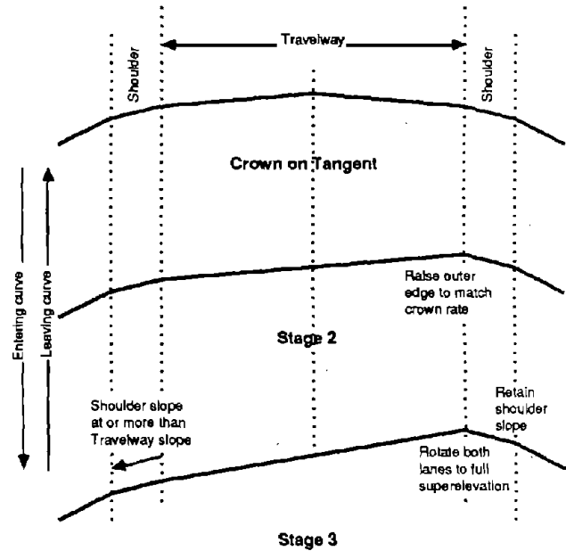
Changing Crown and Superelevation
