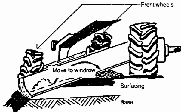
Recover Stored and Wraparound Slope Materials
