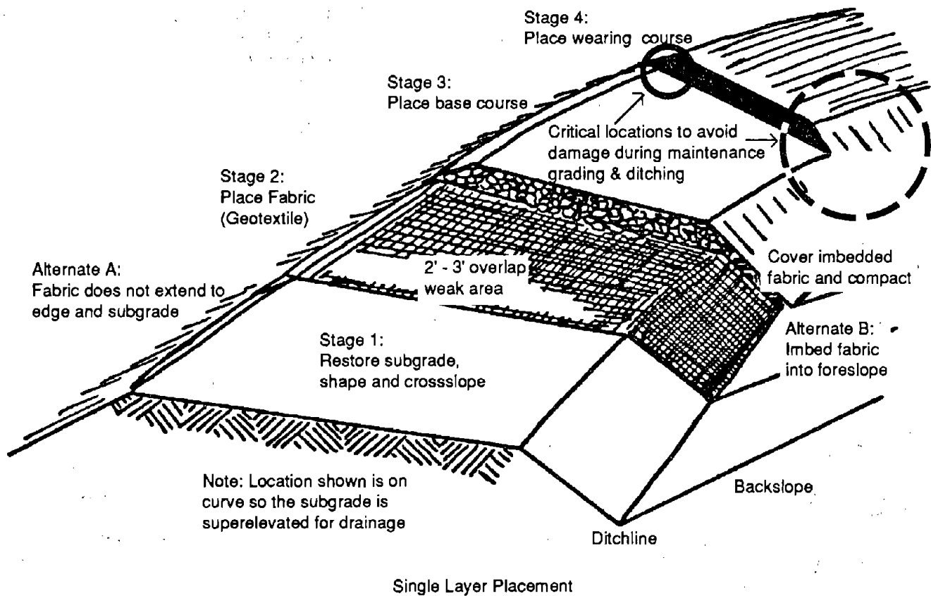
Placement of Geotextile Fabrics
