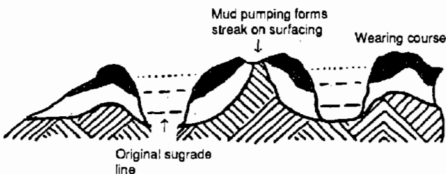
Subgrade Rutted, Severe Damage
