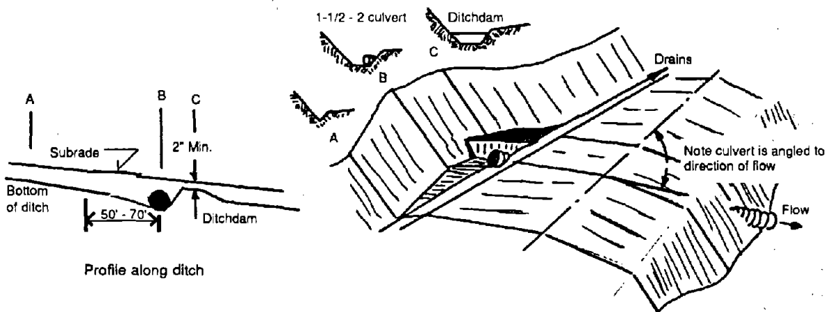
Ditchdam and Catch Basin
