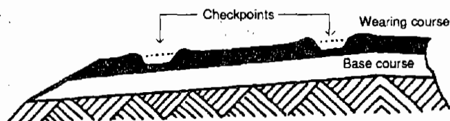
Rutting of Surfacing
