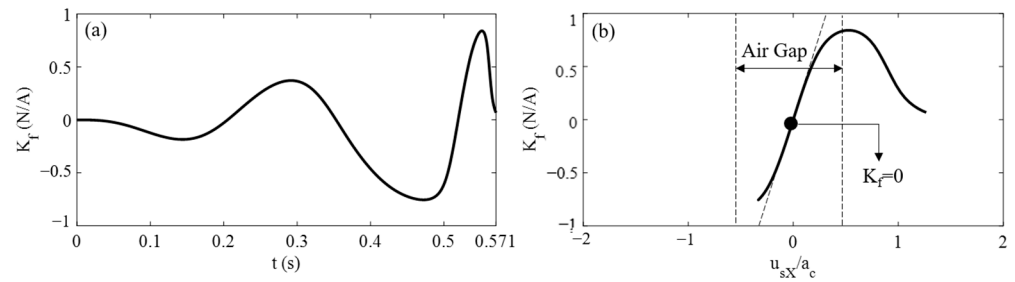
Figure 7. Variation of the electromechanical coupling coefficient with (a) time and (b) displacement of the coil.
