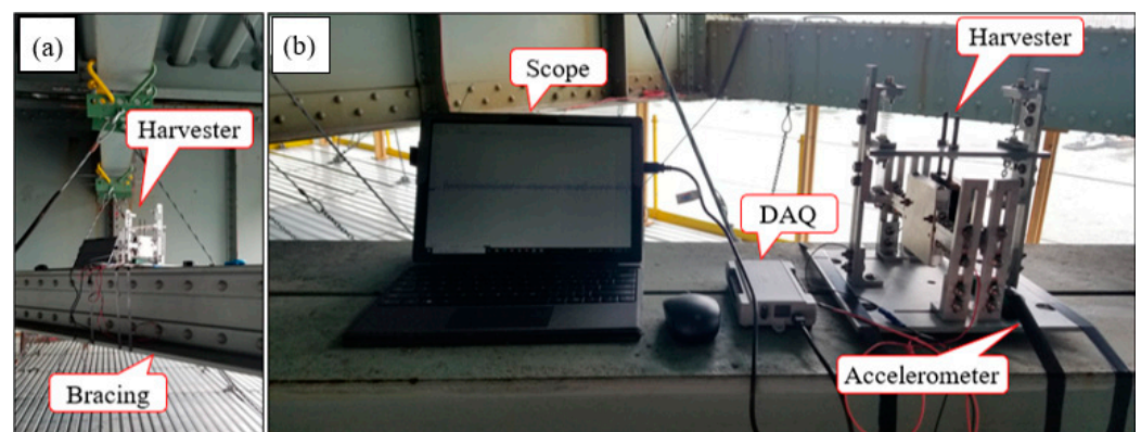
Figure 15. Field testing of the proof-of-concept prototype of EMEH (a) placement of the device on the middle of a horizontal lateral bracing of the deck, and (b) testing setup.
