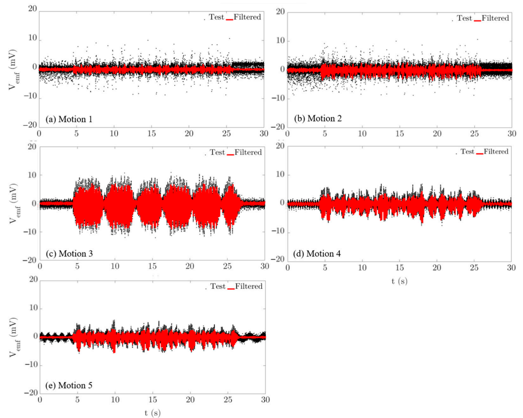
Figure 12. Voltage output from the prototype EMEH subjected to five different base excitations with the frequencies from f_b = 1.5 Hz to f_b = 3.0 Hz; RMSs of these voltage signals are (a) 0.54 mV, (b) 0.93 mV, (c) 2.9 mV, (d) 1.6 mV, and (e) 1.3 mV.
