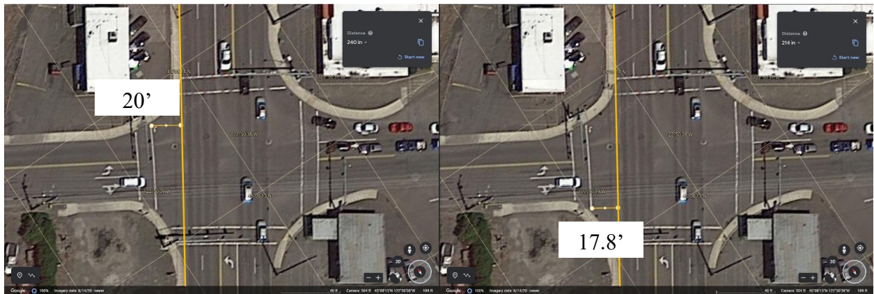
Average Setback Distance Measurement at Young St. and OR 99E
