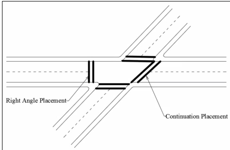
Figure 2.5: Possible crosswalk configurations
