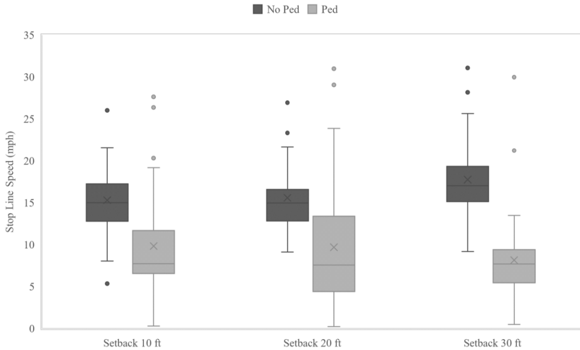
Figure 4.18: Stop line speed with and without pedestrian for left turn at radius 15 ft
