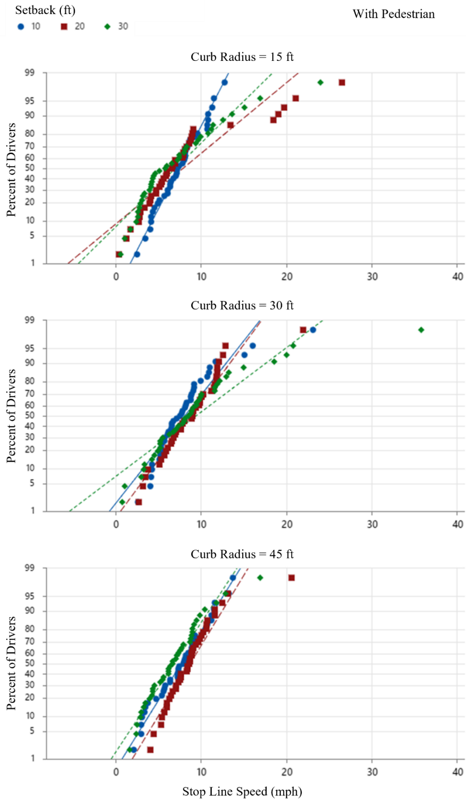
Figure 4.21: Interaction among independent variables with pedestrian
