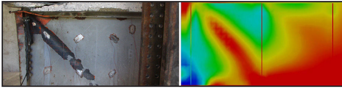
Forensic evaluation of PBES buckled web due to extreme load testing in laboratory (left) and modeling of principal tensile stress (right).
