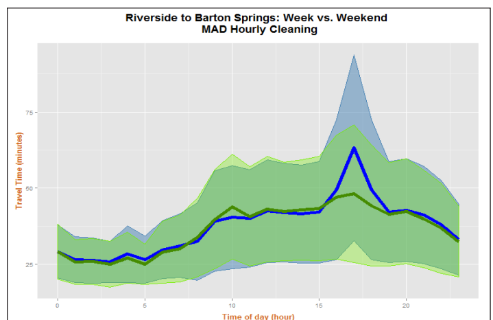
Figure 2. Travel time variability by time of day created by selecting two of the Bluetooth readers from the Figure 1 map.
