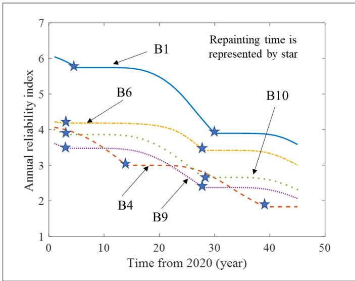
Figure 4. Annual reliability index profiles of the steel bridges in the network.
