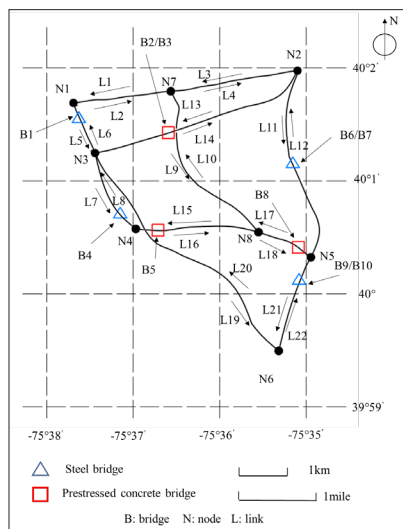
Figure 1. Bridge network in Chester County, PA
