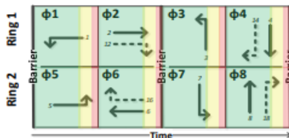
Figure 6. Example of a Ring-Barrier Diagram [6]
