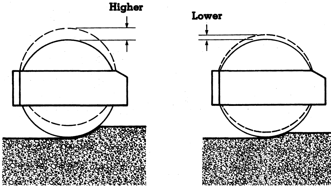
FIGURE 6.15—Illustration of Amplitude.
