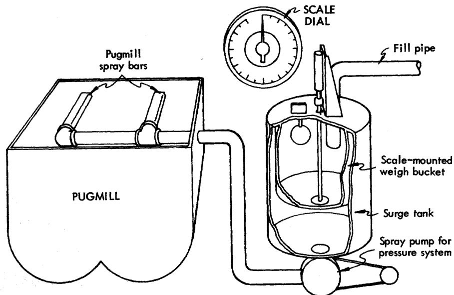
FIGURE 4.48—Typical Asphalt Measuring and Delivery System. (Courtesy Tennessee Department of Transportation).
