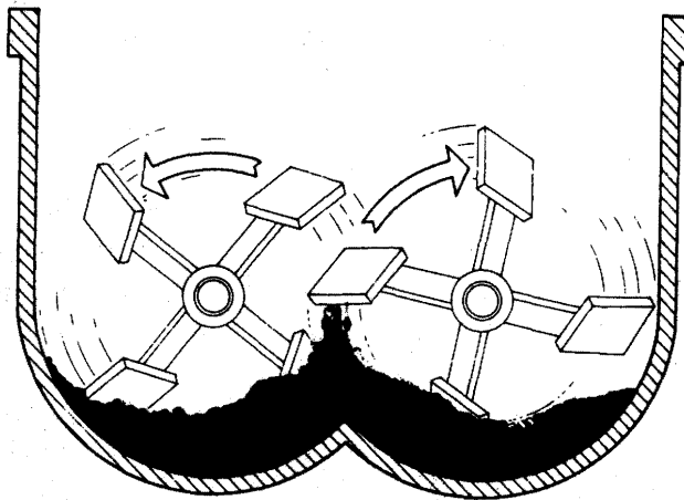
FIGURE 4.52—Underfilled Pugmill.
