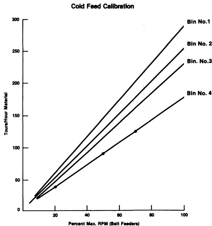
FIGURE 4.16—Calibration Chart.
