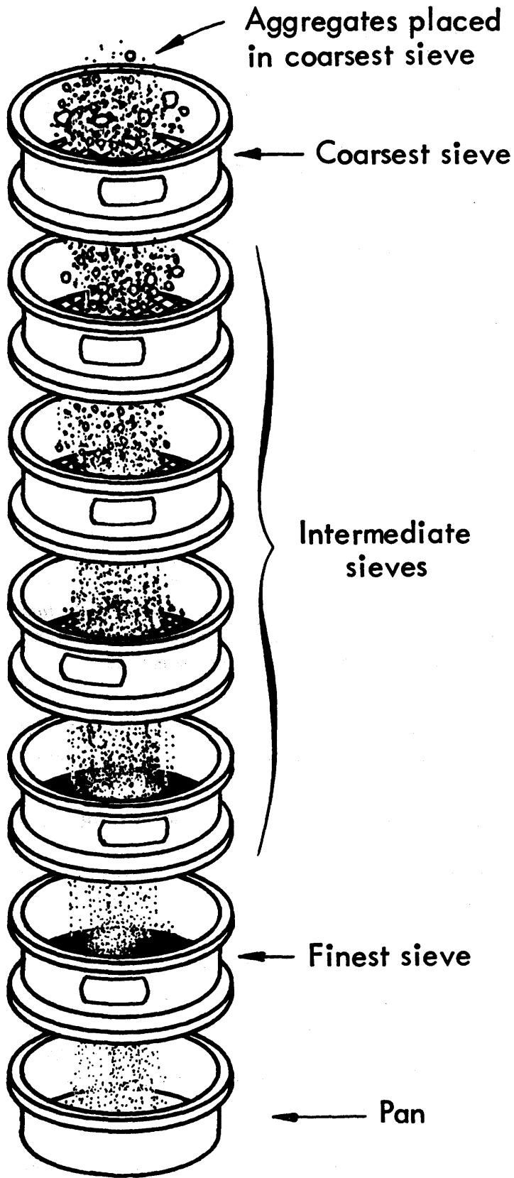
Figure 2.22—Sieve Analysis.
