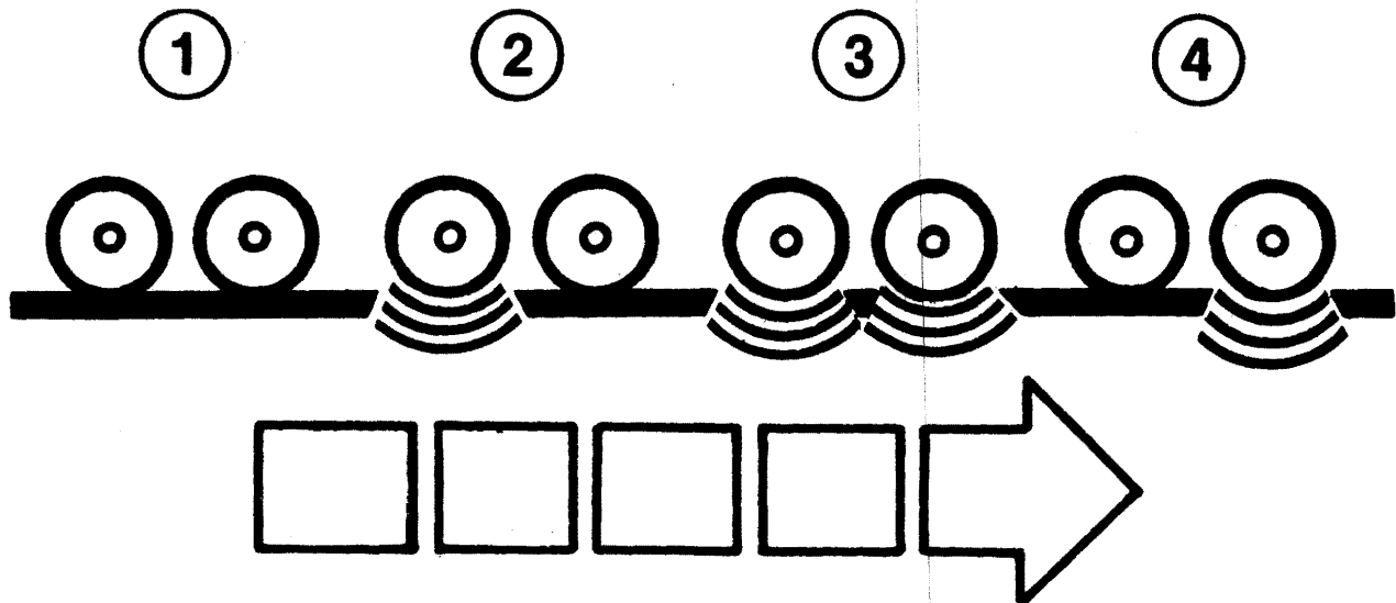
FIGURE 6.17—Vibration Modes.
