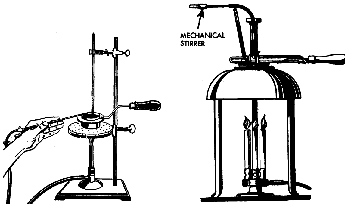
FIGURE 2.13—Flashpoint Tests; (left) Cleveland Open Cup Test, (rt) Pensky-Martens Test.
