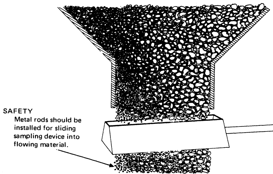
FIGURE 4.41—Correct Use of Sampling Device.
