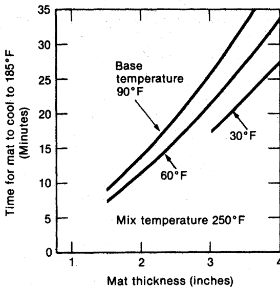
Figure 1 — Times for asphalt to cool to 185°F.
