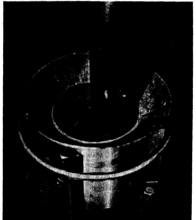
FIGURE 3.26—Mechanical Compactor Compacting Mixture Sample.
