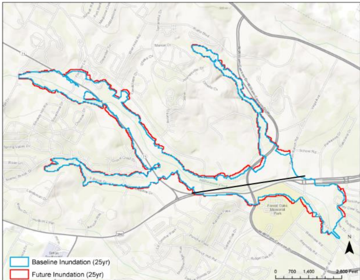
Figure C-1 Inundation extent for baseline (blue) and future (red) 25-yr event at Location 5.
