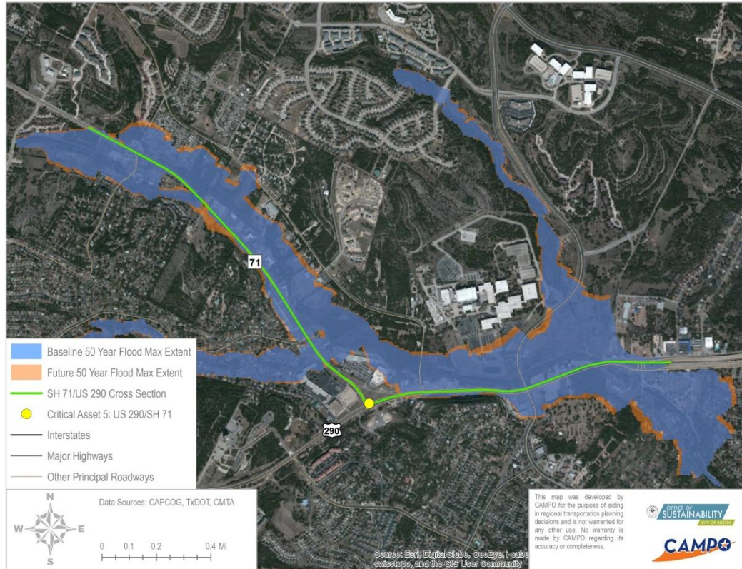
Figure D-9 FEWS 50 Year Maximum Flood Extents and Cross-section Location
