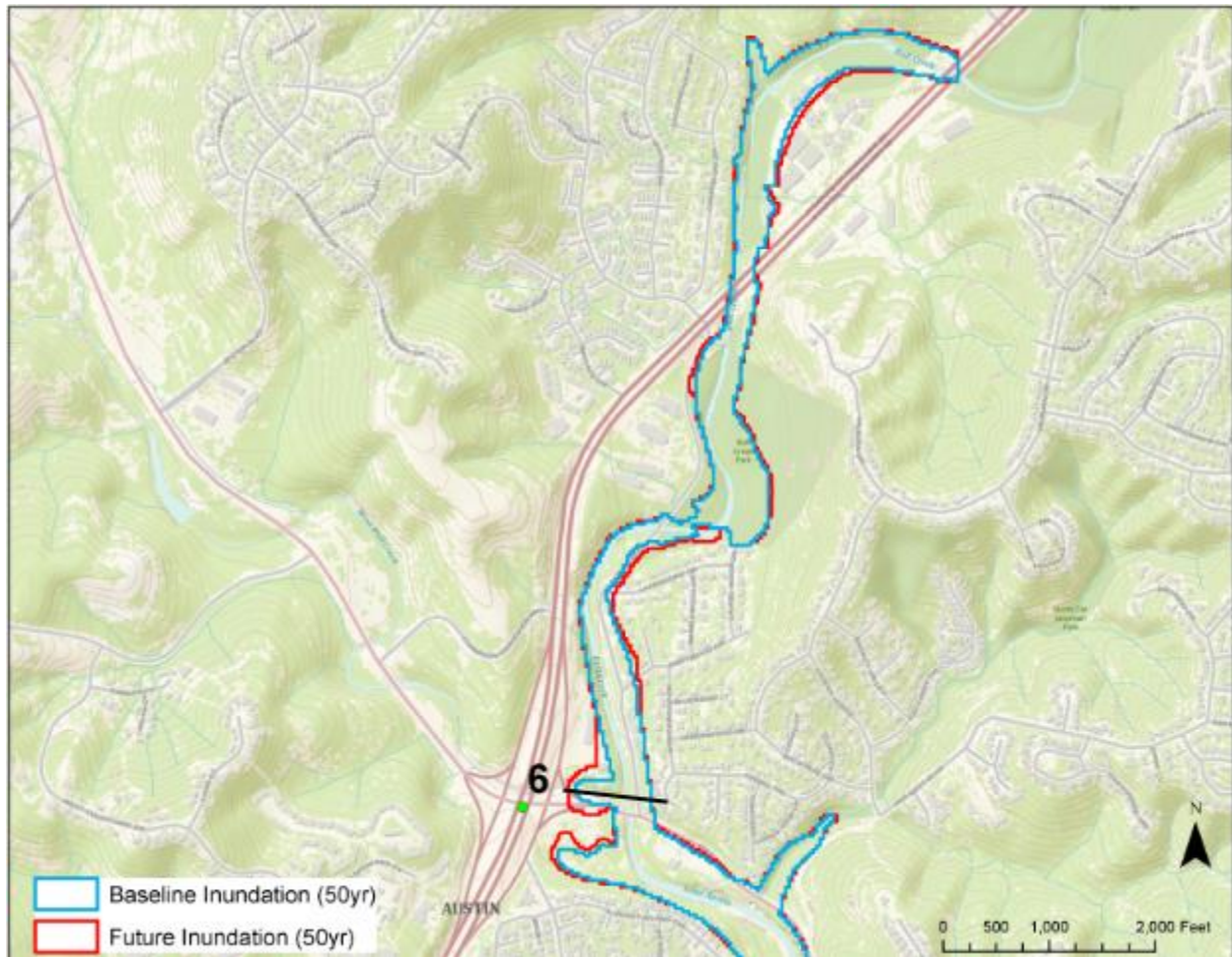
Figure D-2 Inundation extent for baseline (blue) and future (red) 50-yr event at Location 6.
