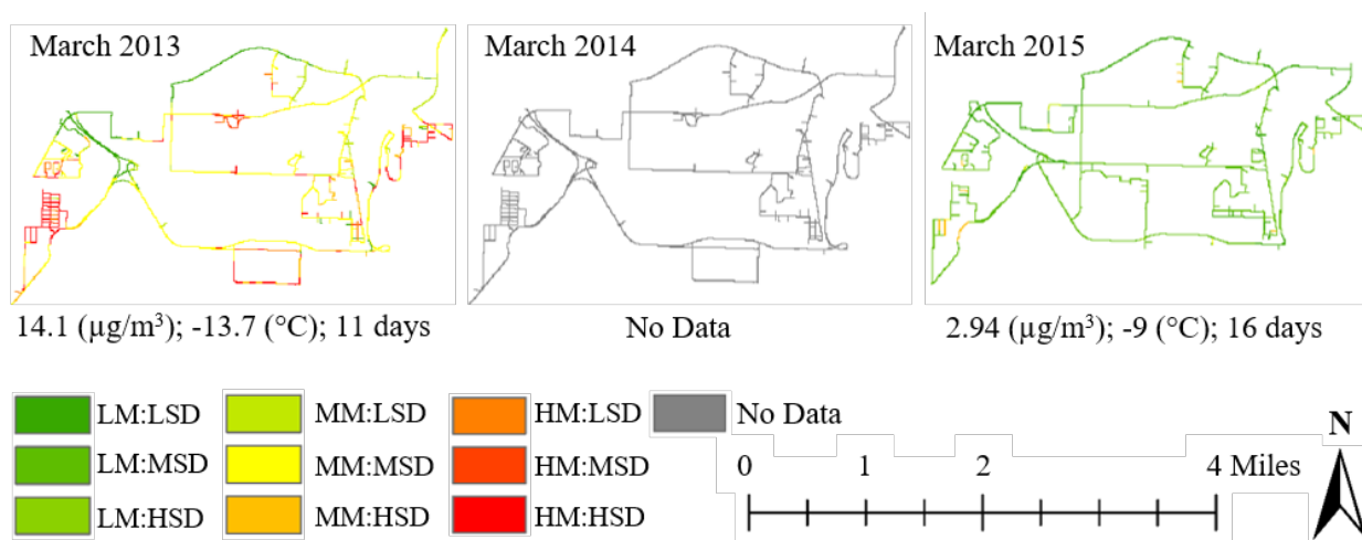
Figure 2.4 Monthly mean \text{PM}_{2.5} concentration in Fairbanks. The numbers below each map represent the consecutive monthly average of \text{PM}_{2.5} , the monthly average temperature, and the number of days the MMV was driven during that month.
