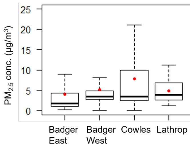
Figure 3.6 Distribution of PM_{2.5} concentrations at different locations in Fairbanks and North Pole. Box represents 25 th , 50 th , and 75 th percentiles; whiskers extend at most to 1.5 interquartile ranges. Red dots denote mean value
