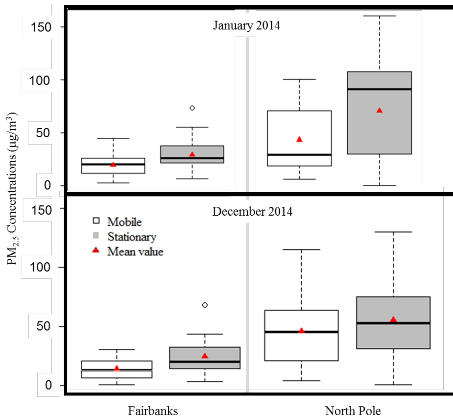
Figure 2.7 Average concentrations of hourly PM 2.5 data. Only the MMV operating days (during the hours that the MMV was driven) are considered for MMV as well as stationary data. The boxes represent the 25 th , 50 th , and 75 th percentiles; whiskers extend at most to 1.5 interquartile ranges.
