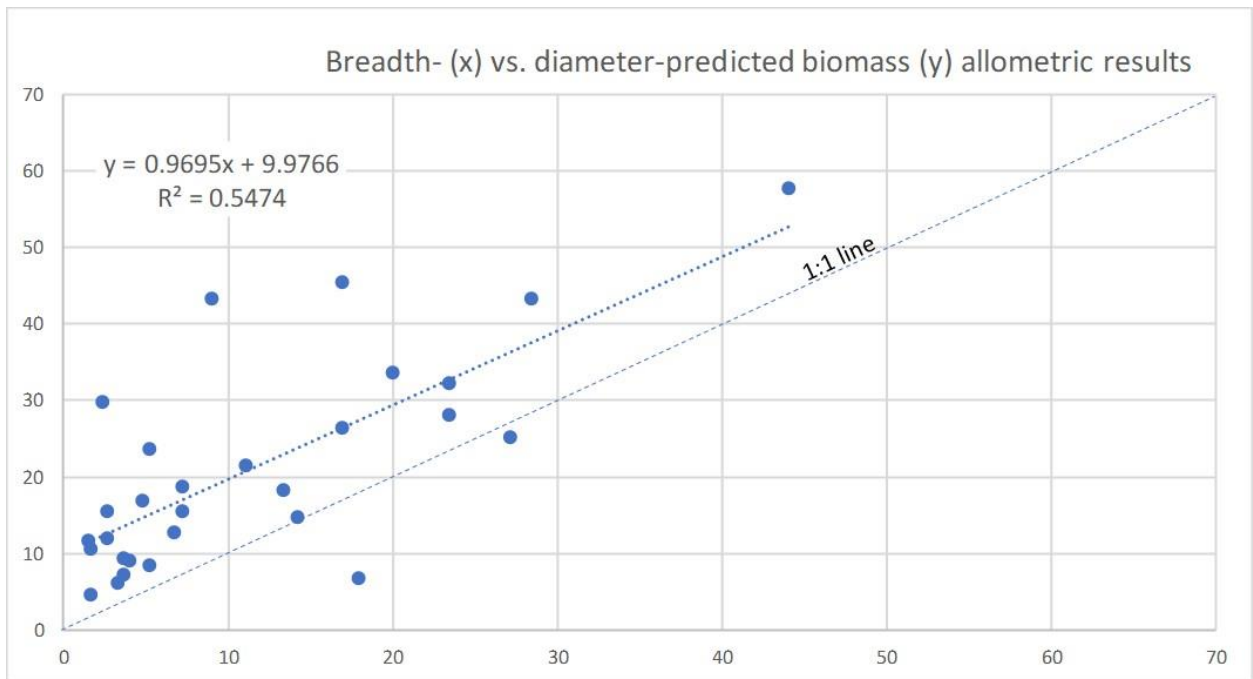
Figure 20. Comparison of predicted biomass using two approaches. X-axis shows biomass predicted with breadth measurements, and Y-axis shows biomass predicted with basal diameter measurements.
