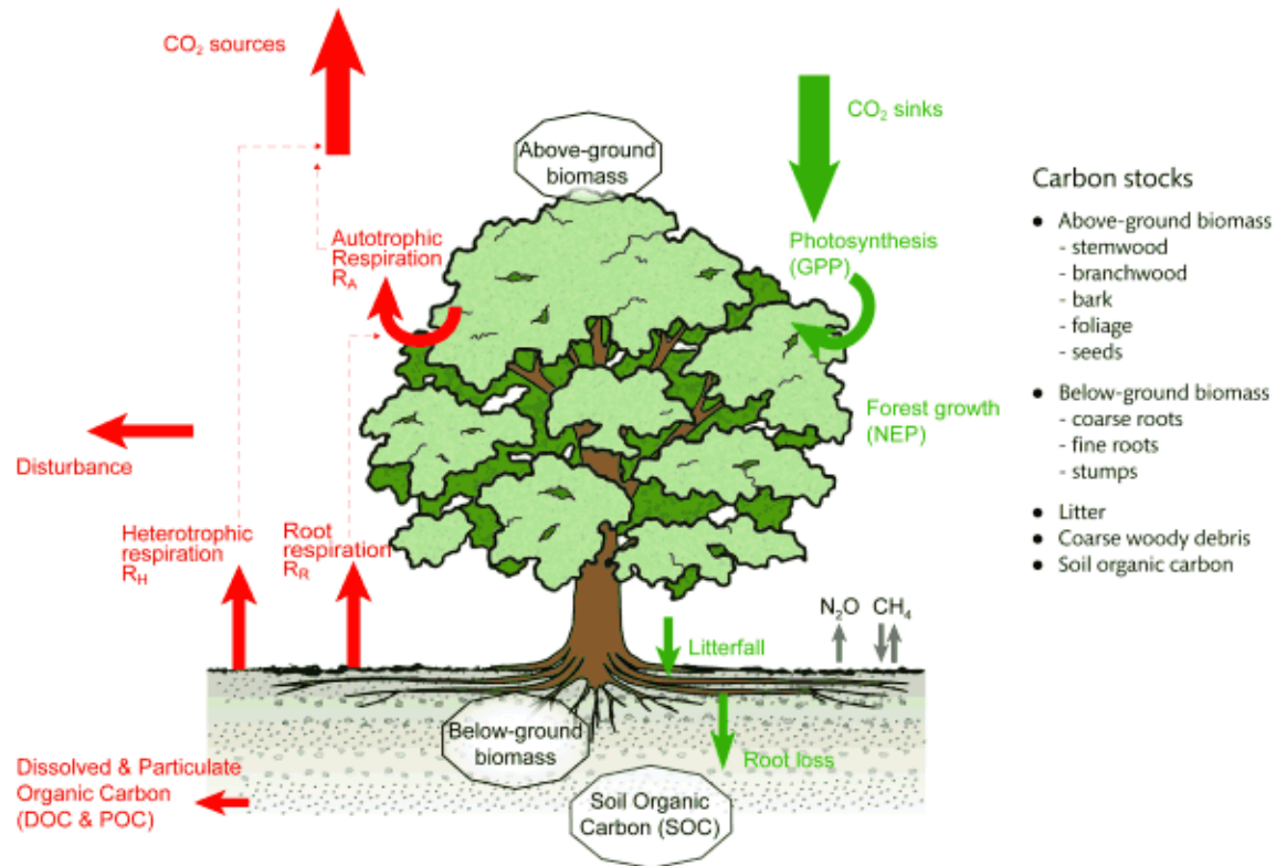
Figure 3 – Terrestrial Carbon sequestration diagram.
