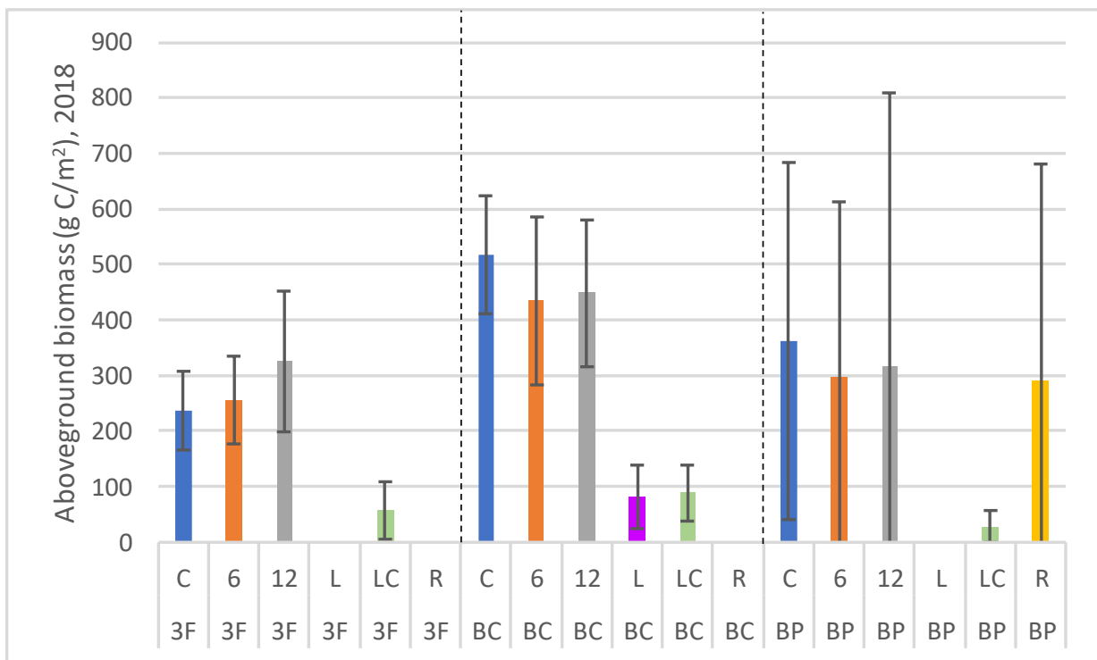
Figure 19. Summary of average ( \pm 1 SD; n=4-10 ) estimated aboveground biomass carbon ( \text{g m}^{-2} ; 2018), by site (3F=Three Forks, BC=Bear Canyon, BP=Bozeman Pass) and treatment (C=control, 6=6 in. mow, 12=12 in. mow, L=legume, LC=legume “control,” and R=rabbitbrush). Estimates assume dry biomass is 50% carbon.
