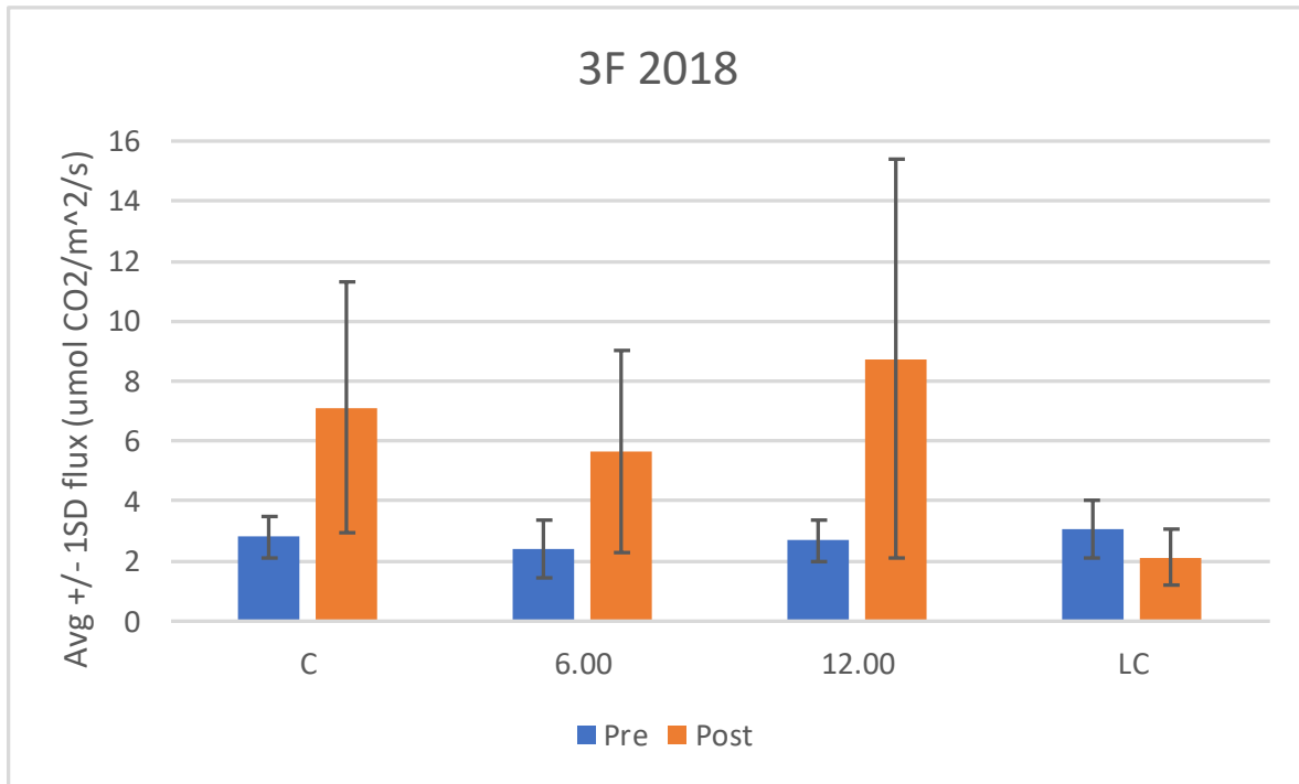
Figure 25. Summary of average soil respiration rates (SD; n=10 duplicate readings; \mu\text{mol CO}_2 \text{ m}^{-2} \text{ s}^{-1} ) at 3F, by treatment (6=6 in. mow, 12=12 in. mow, C=control, LC=cleared-legume).
