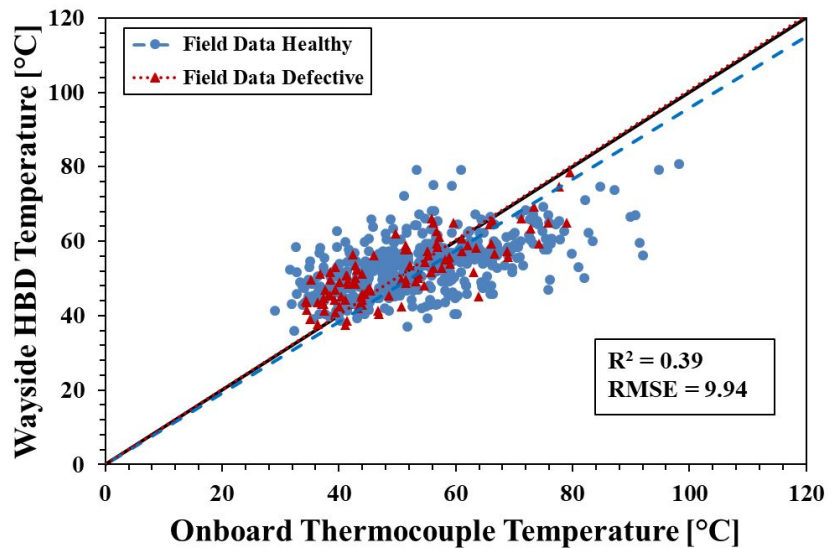
Figure 6. Calibrated field-test wayside HBD temperature versus onboard thermocouple temperature
