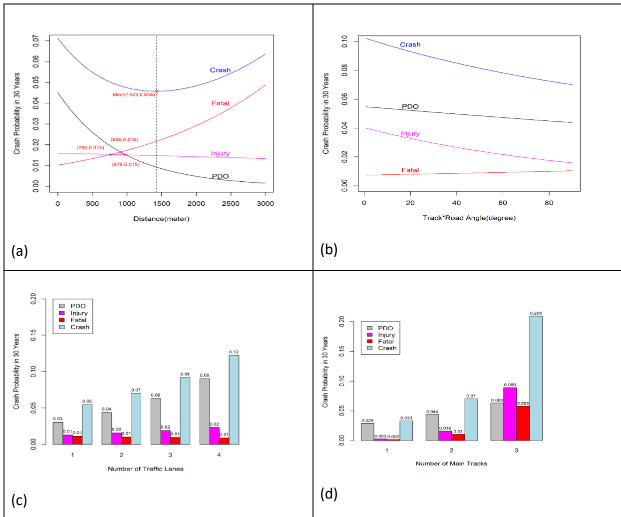
Figure 4.1 Cumulative Crash/Severity Probabilities for Geometric Factors
