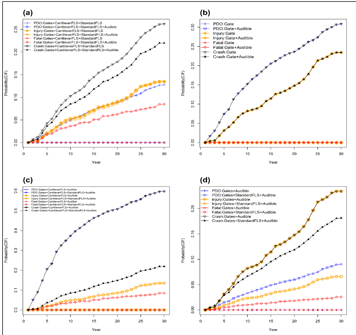
Figure 5.2 Crash Severity and Frequency Likelihoods for the Second HRGC Control Pairs
