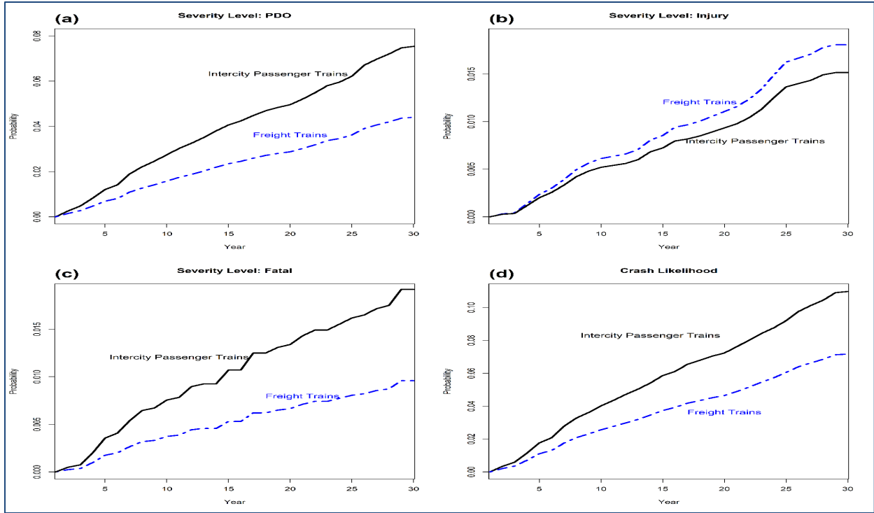
Figure 3.1 CIF of Crash and Severity for Train Services
