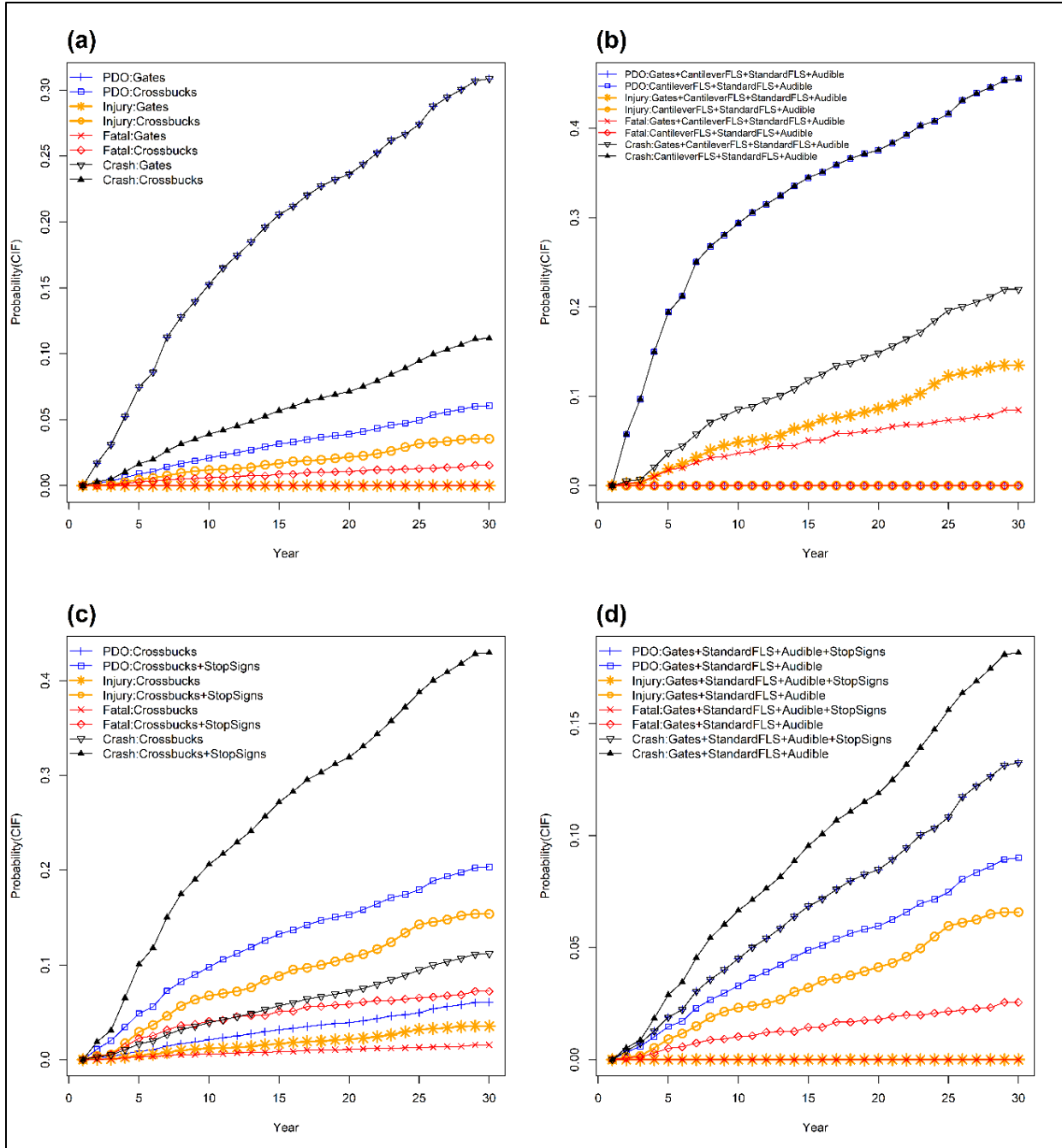
Figure 5.1 Crash Severity and Frequency Likelihoods for the First HRGC Control Pairs
