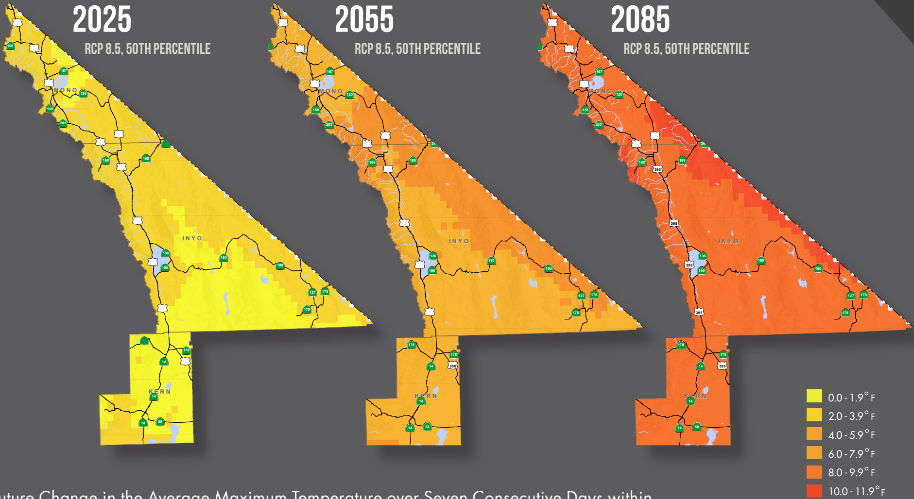
Future Change in the Average Maximum Temperature over Seven Consecutive Days within District 9, Based on the RCP 8.5 Emissions Scenario
