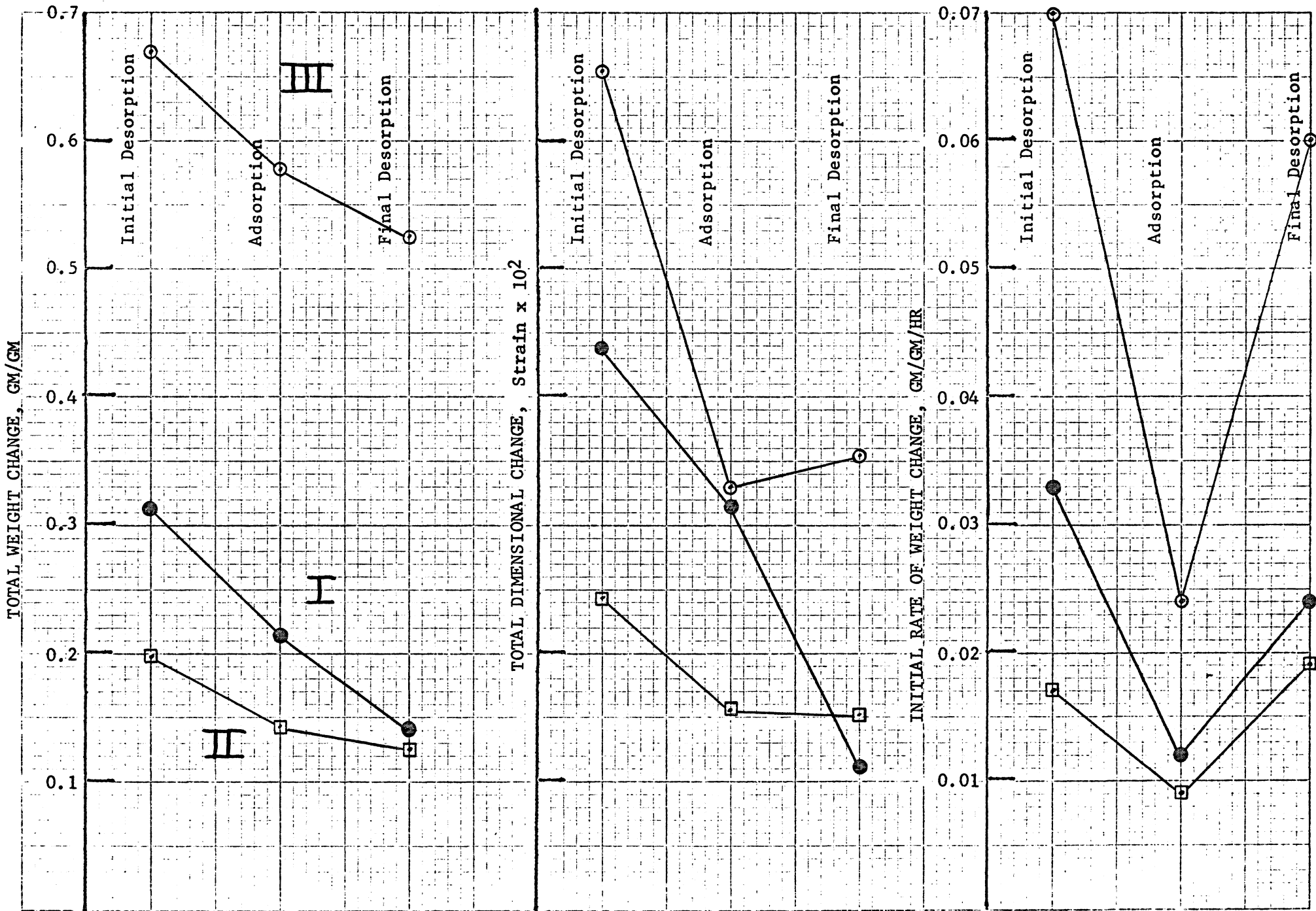
FIGURE 19. CEMENT #27, TYPE I. TOTAL WEIGHT CHANGE, TOTAL DIMENSIONAL CHANGE, AND INITIAL RATE OF WEIGHT CHANGE (0-5 HR) EXHIBITED DURING INITIAL DESORPTION, ADSORPTION, AND FINAL DESORPTION.
