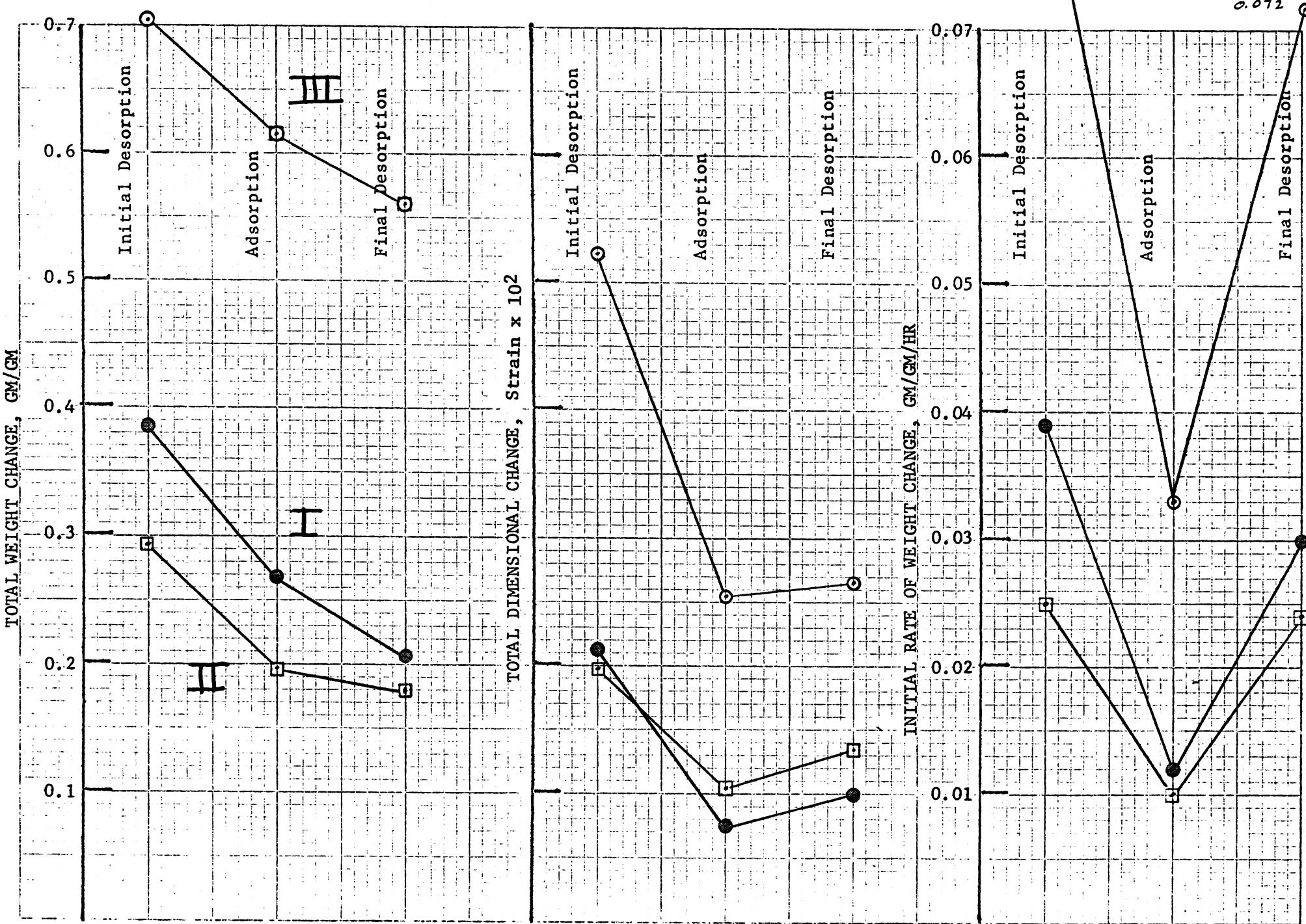
FIGURE 11. CEMENT #9. TYPE I. TOTAL WEIGHT CHANGE, TOTAL DIMENSIONAL CHANGE, AND INITIAL RATE OF WEIGHT CHANGE (0.5 HR) EXHIBITED DURING INITIAL DESORPTION, ADSORPTION, AND FINAL DESORPTION
