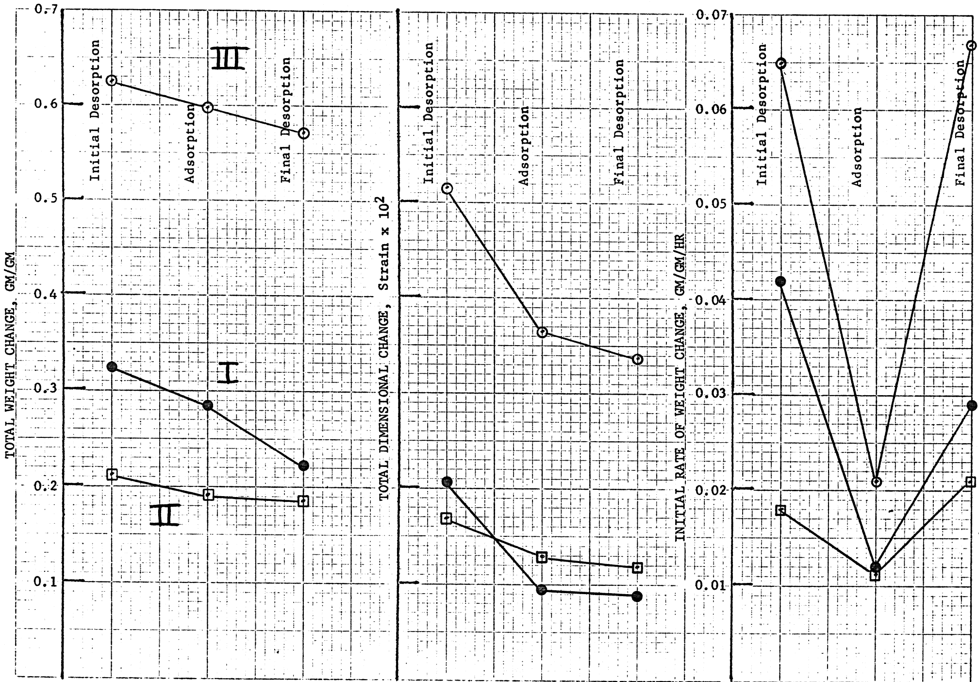
FIGURE 26. CEMENT #17, TYPE II. TOTAL WEIGHT CHANGE, TOTAL DIMENSIONAL CHANGE, AND INITIAL RATE OF WEIGHT CHANGE (0-5 HR) EXHIBITED DURING INITIAL DESORPTION, ADSORPTION, AND FINAL DESORPTION.
