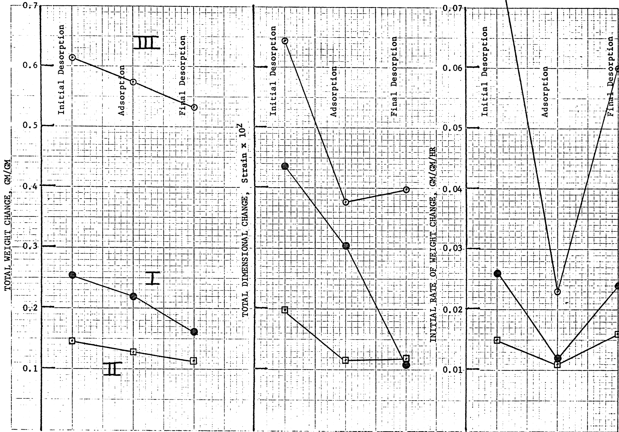
FIGURE 17. CEMENT #23, TYPE I. TOTAL WEIGHT CHANGE, TOTAL DIMENSIONAL CHANGE, AND INITIAL RATE OF WEIGHT CHANGE (0-5 HR) EXHIBITED DURING INITIAL DESORPTION ADSORPTION AND FINAL DESORPTION
