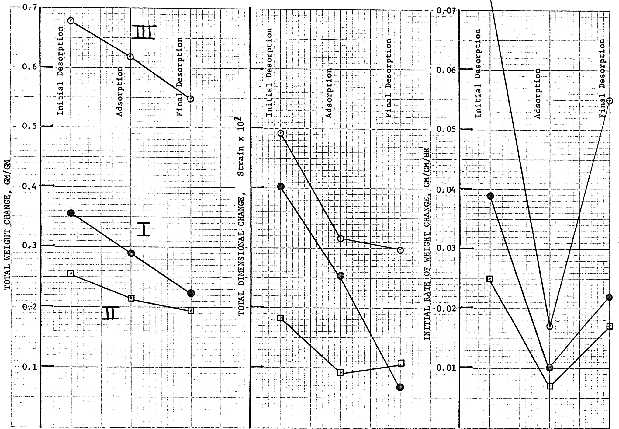
FIGURE 33. CEMENT #21, TYPE V. TOTAL WEIGHT CHANGE, TOTAL DIMENSIONAL CHANGE, AND INITIAL RATE OF WEIGHT CHANGE (0-5 HR) EXHIBITED DURING INITIAL DESORPTION, ADSORPTION, AND FINAL DESORPTION.
