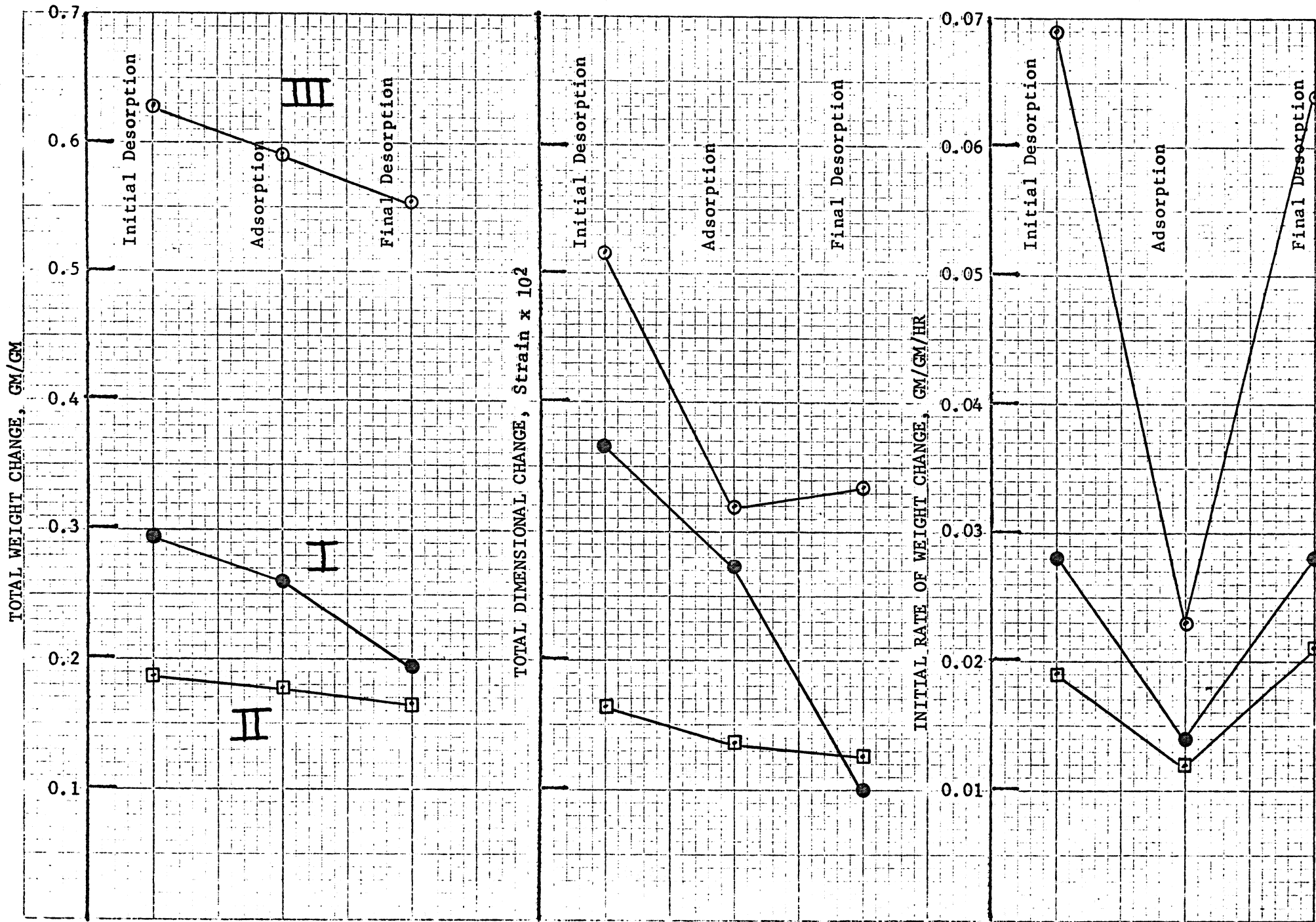
FIGURE 16. CEMENT #22, TYPE I. TOTAL WEIGHT CHANGE, TOTAL DIMENSIONAL CHANGE, AND INITIAL RATE OF WEIGHT CHANGE (0-5 HR) EXHIBITED DURING INITIAL DESORPTION, ADSORPTION, AND FINAL DESORPTION.
