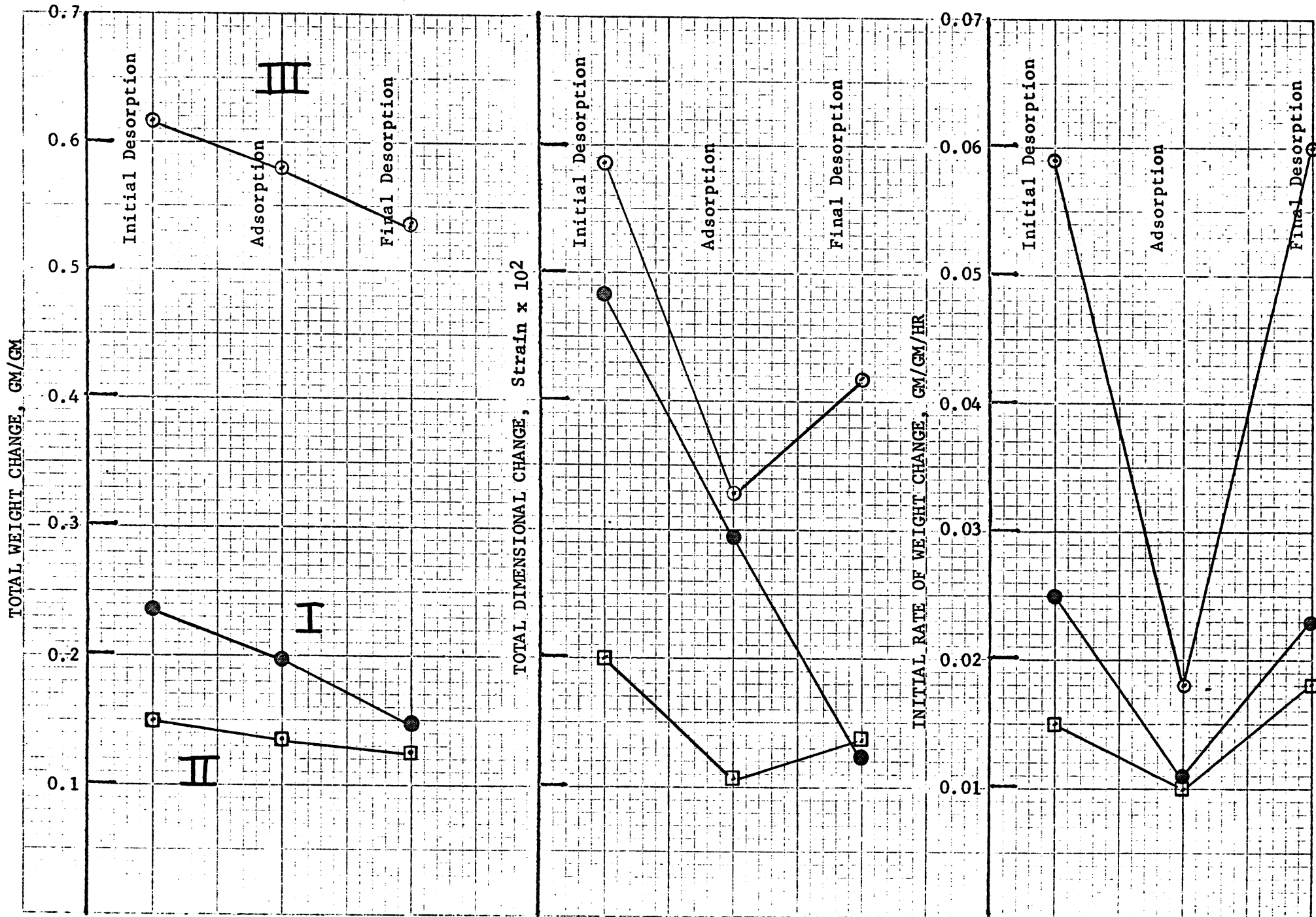
FIGURE 28. CEMENT #20. TYPE III. TOTAL WEIGHT CHANGE, TOTAL DIMENSIONAL CHANGE, AND INITIAL RATE OF WEIGHT CHANGE (0-5 HR) EXHIBITED DURING INITIAL DESORPTION, ADSORPTION, AND FINAL DESORPTION.
