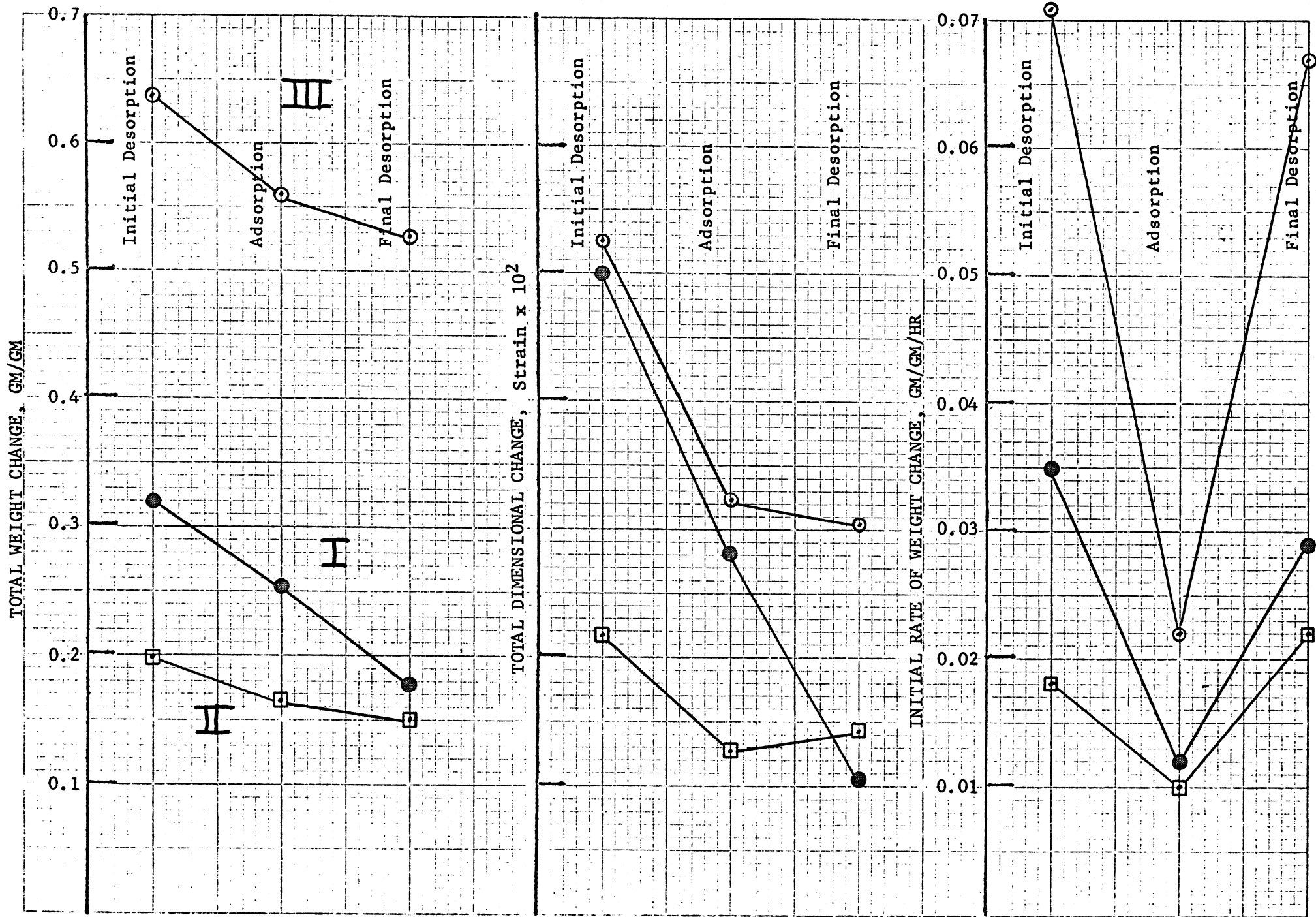
FIGURE 20. CEMENT #71. TYPE I. TOTAL WEIGHT CHANGE, TOTAL DIMENSIONAL CHANGE, AND INITIAL RATE OF WEIGHT CHANGE (0-5 HR) EXHIBITED DURING INITIAL DESORPTION, ADSORPTION, AND FINAL DESORPTION.
