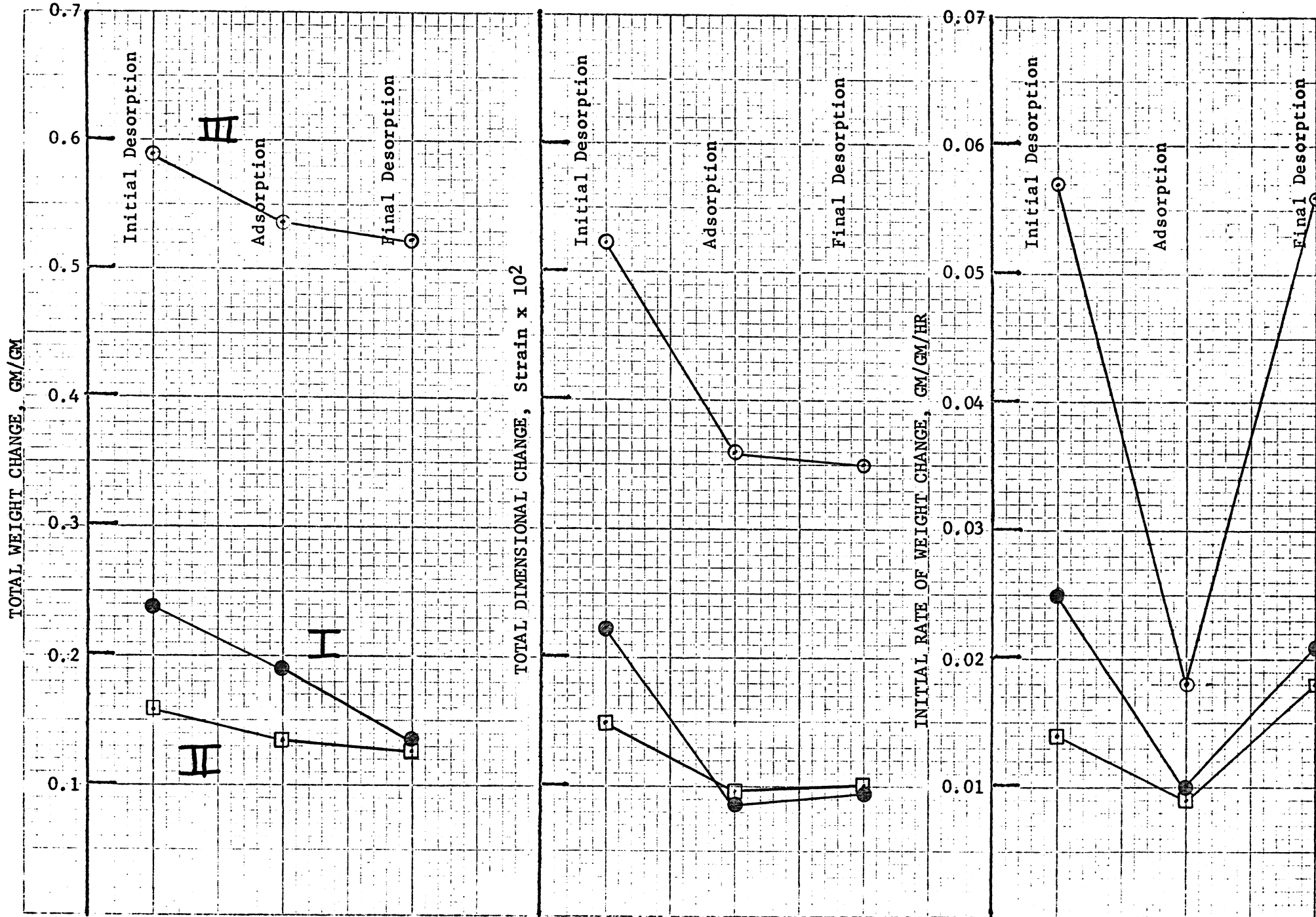
FIGURE 7. CEMENT #4. TYPE I. TOTAL WEIGHT CHANGE, TOTAL DIMENSIONAL CHANGE, AND INITIAL RATE OF WEIGHT CHANGE (0-5 HR) EXHIBITED DURING INITIAL DESORPTION, ADSORPTION, AND FINAL DESORPTION.
